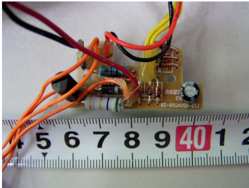
EUT-Charging board Bottom View
