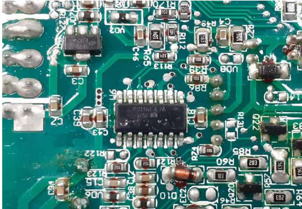
EUT Photo (25)
