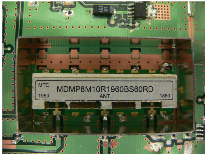
EUT- RF shielding off View 2
