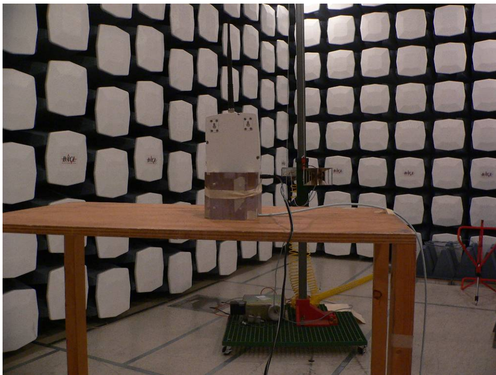
Forward Radiated Emission –Rear View
