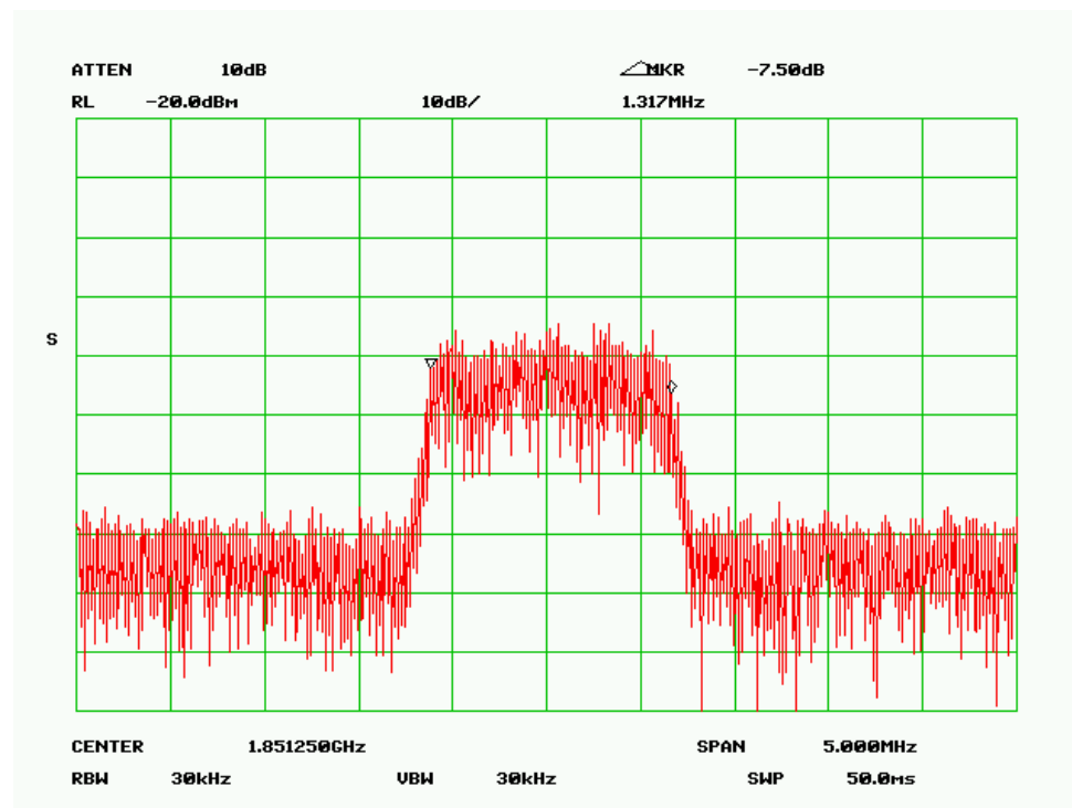
Low channel -99% BW
