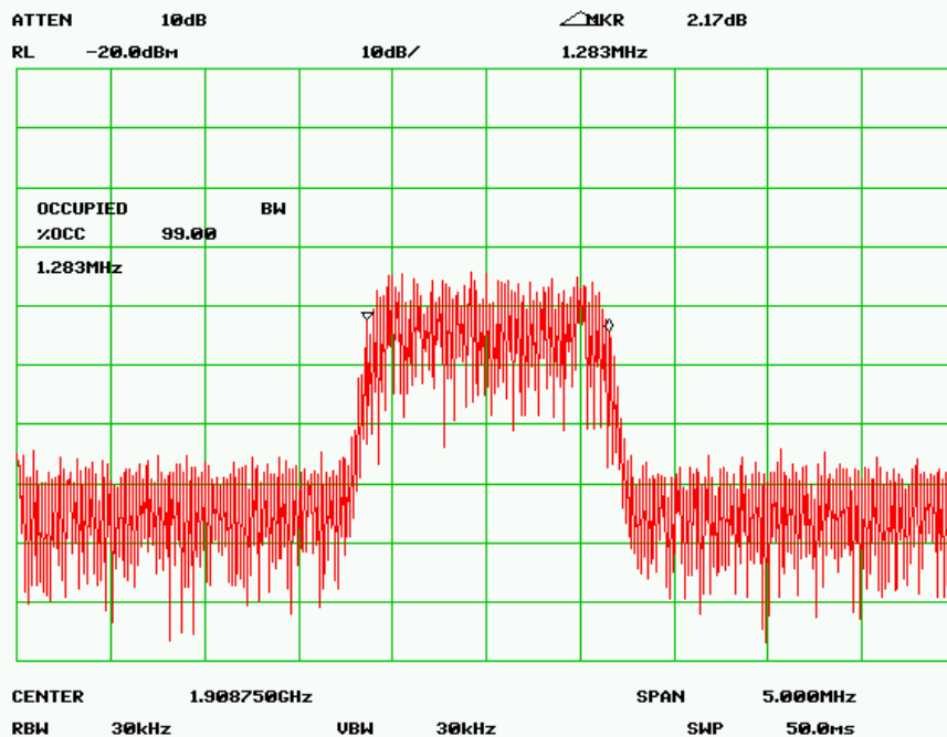
High channel -99% BW
