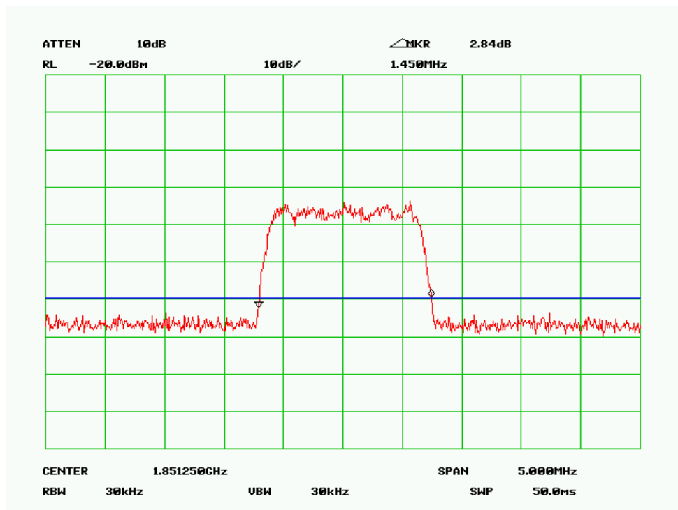
Low Channel -26dB BW
