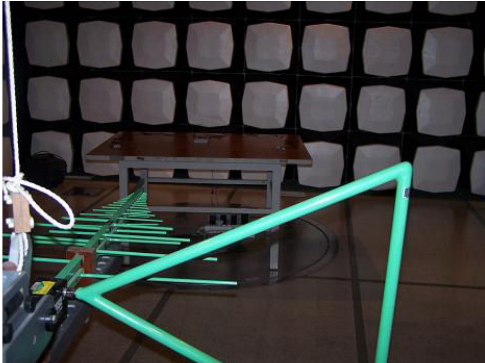
Radiated Emission(30MHz-2GHz)
