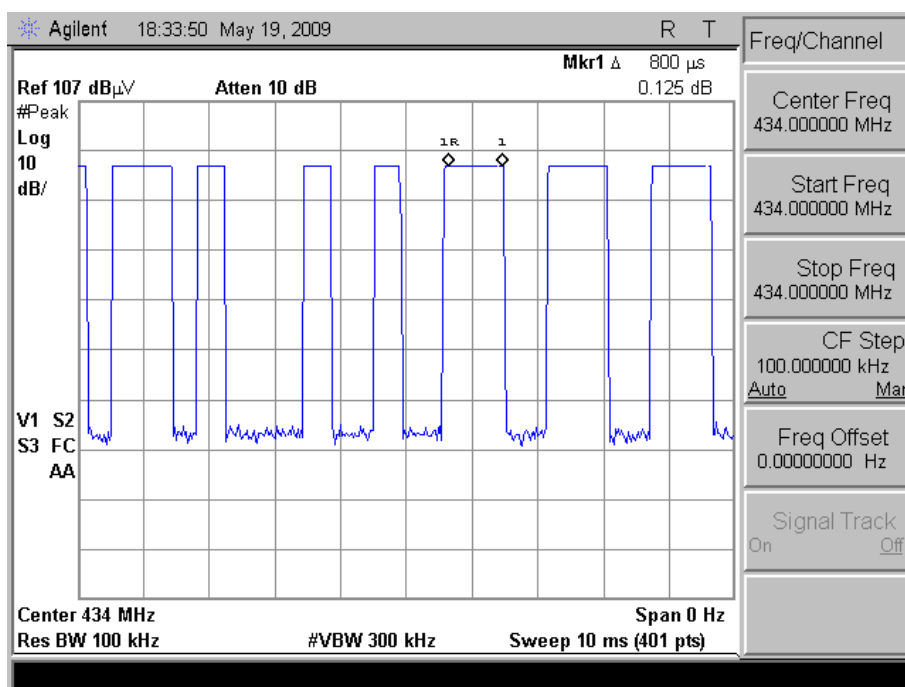
Time Slot 1
