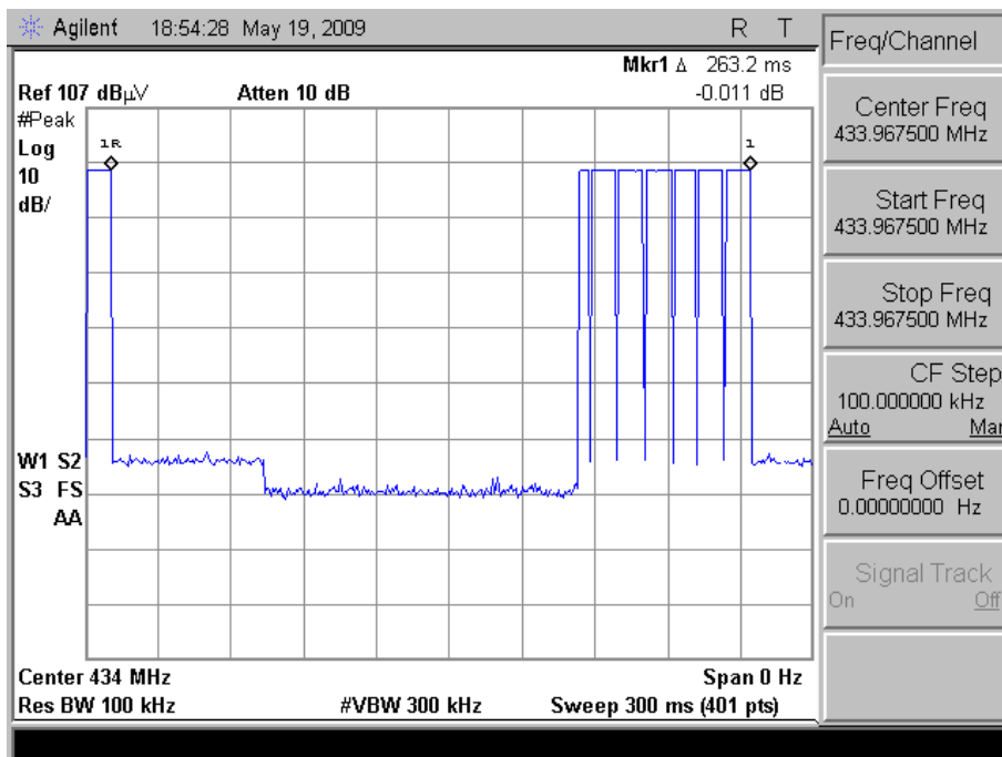
Duty cycle 1
