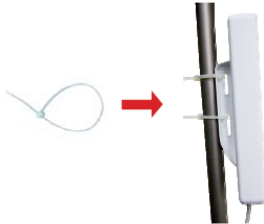
Figure 3-6 Pole Mounting
