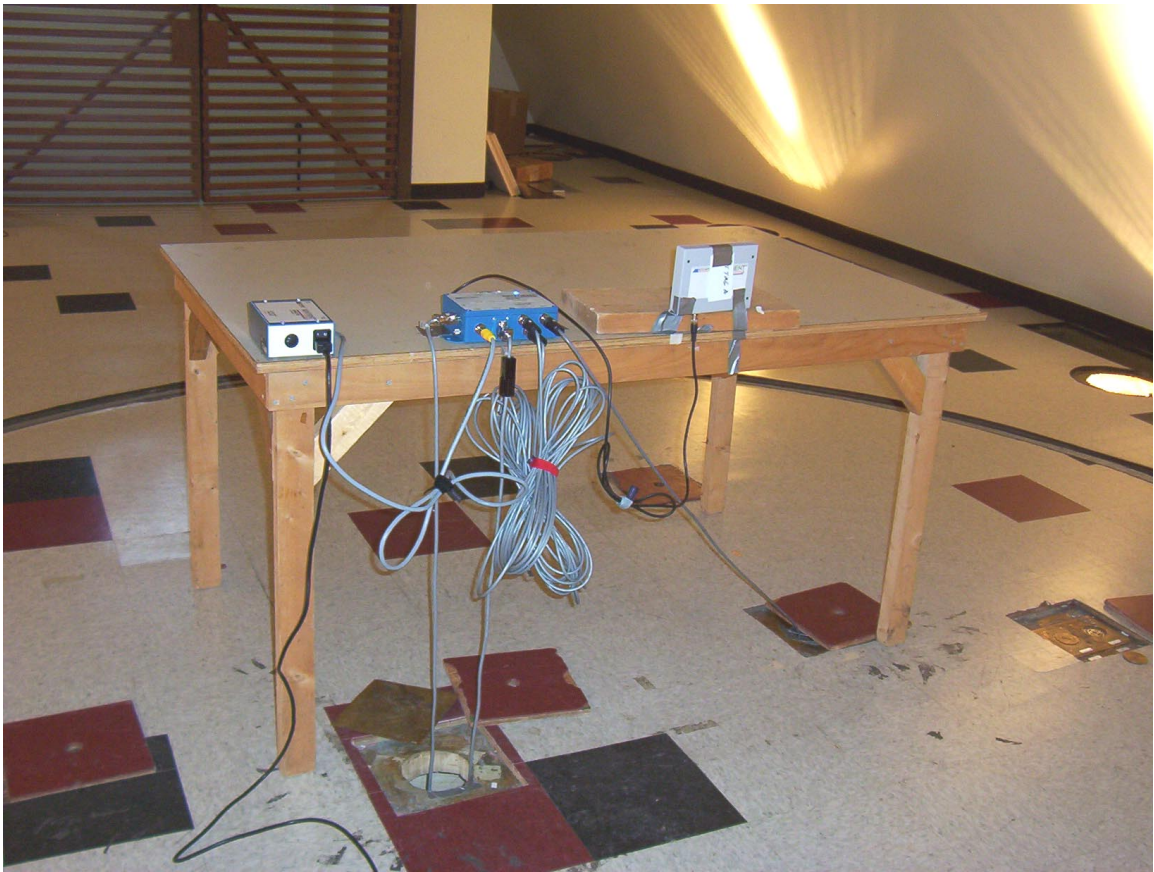
RFR-02/RFA-02 Radiated Emission Test Setup
