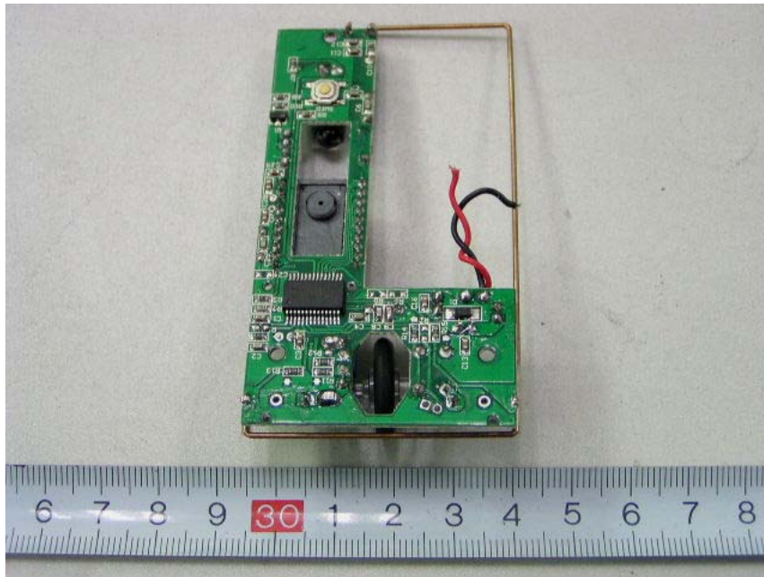
EUT-PCB 2 Back View
