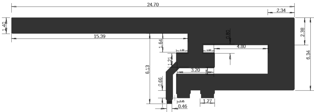
Antenna Dimensions
