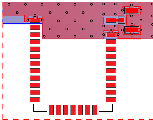
FIGURE 11-6: BM78SPP05NCS HOST PCB MOUNTING SUGGESTION
