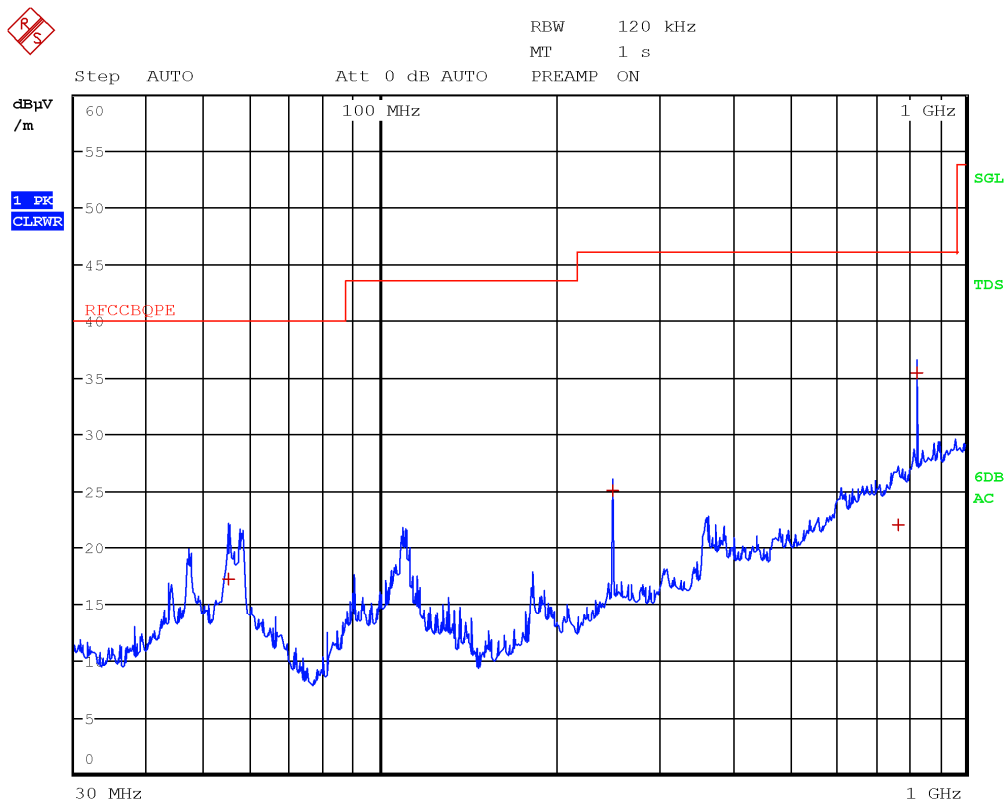
Figure 8.7-53: Radiated spurious emissions 30 to 1000 MHz, High channel with antenna in horizontal polarization
