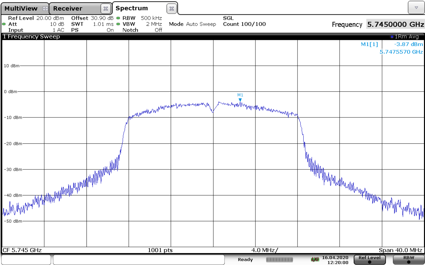
Figure 8.3-4: PSD on 802.11a – low channel
