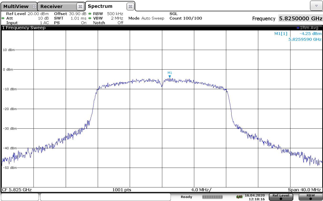
Figure 8.3-6: PSD on 802.11a – high channel
