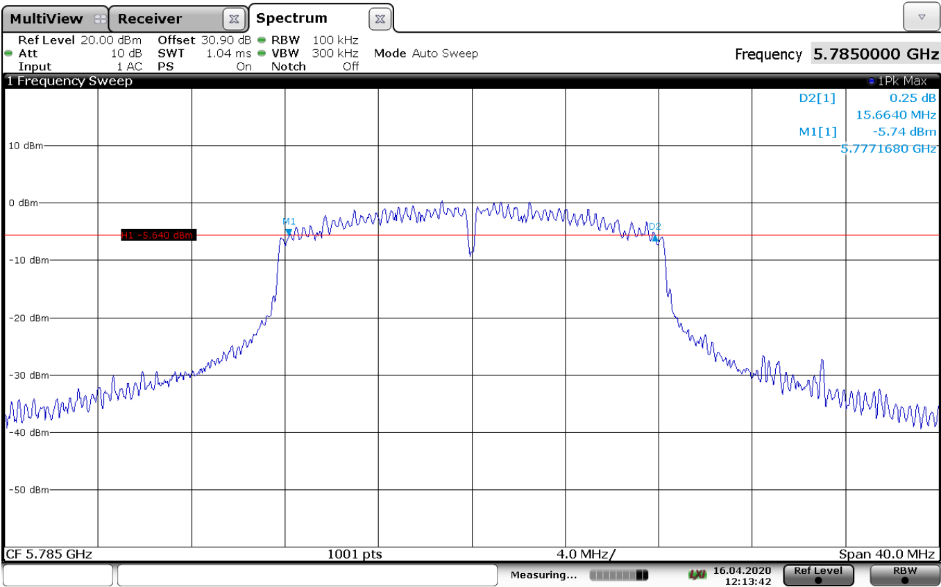
Figure 8.1-5: 6 dB bandwidth on 802.11a, mid channel
