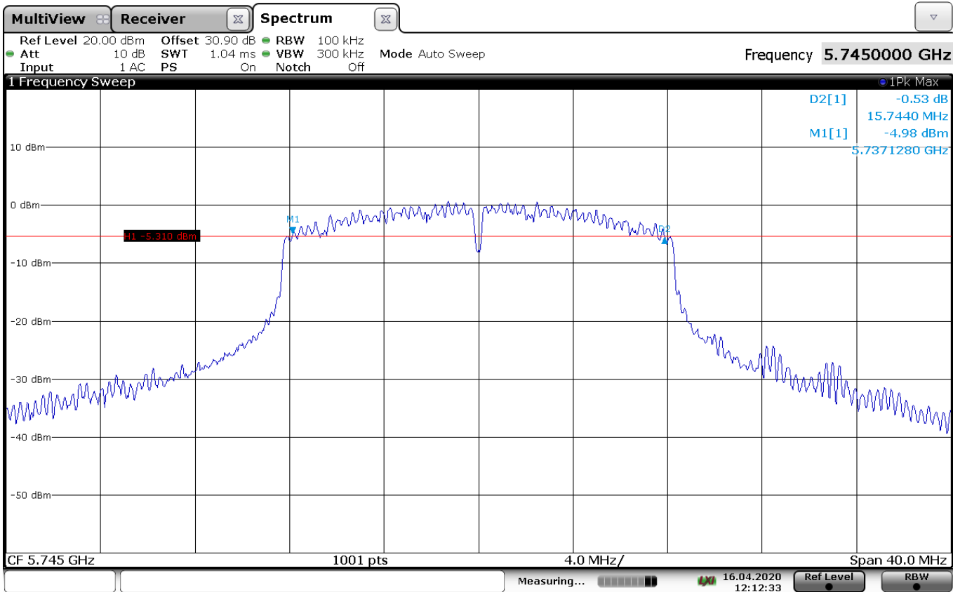
Figure 8.1-4: 6 dB bandwidth on 802.11a, low channel
