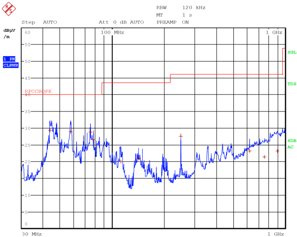
Figure 8.4-28: Radiated spurious emissions 30 to 1000 MHz, mid channel with antenna in vertical polarization
