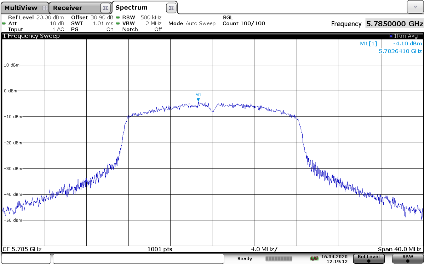
Figure 8.3-5: PSD on 802.11a – mid channel
