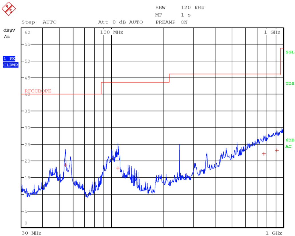
Figure 8.4-27: Radiated spurious emissions 30 to 1000 MHz, mid channel with antenna in horizontal polarization
