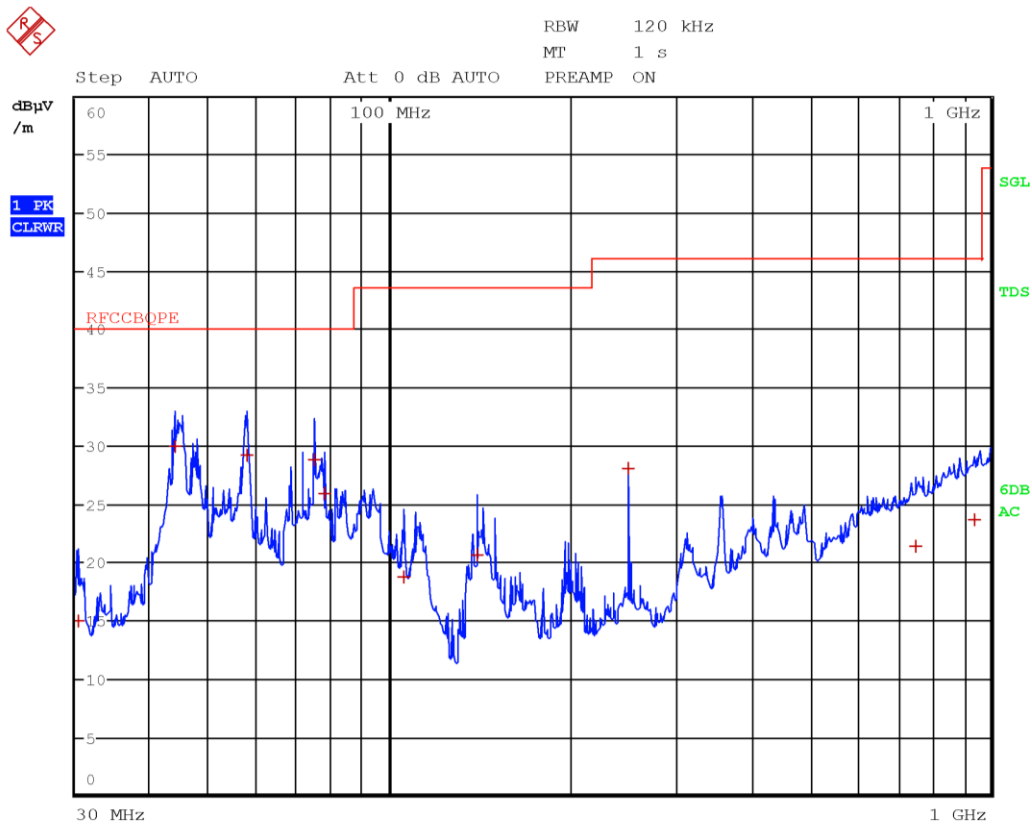
Figure 8.4-30: Radiated spurious emissions 30 to 1000 MHz, high channel with antenna in vertical polarization
