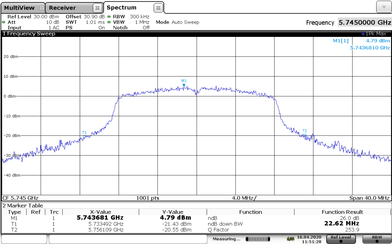
Figure 8.1-1: 26 dB bandwidth on 802.11a, low channel
