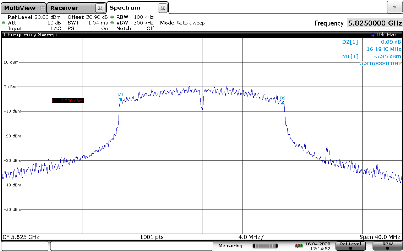
Figure 8.1-6: 6 dB bandwidth on 802.11a, high channel
