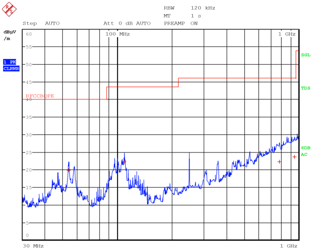
Figure 8.4-29: Radiated spurious emissions 30 to 1000 MHz, high channel with antenna in horizontal polarization
