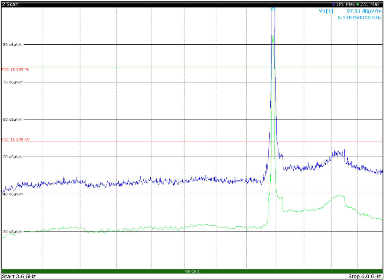
Figure 8.4-37: Radiated spurious emissions 3.6 to 6 GHz, Low channel with antenna in horizontal polarization Limit exceeded by the carrier
