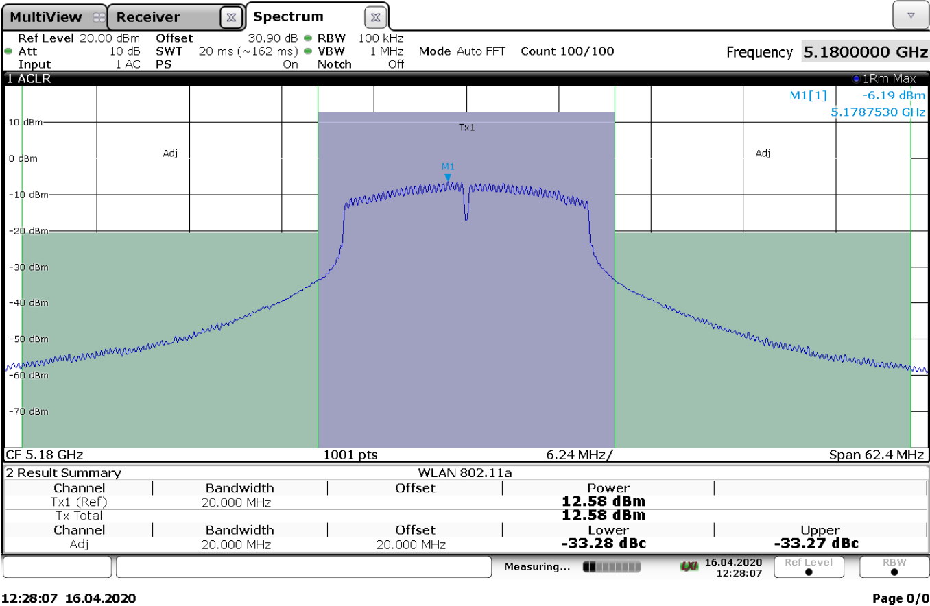
Figure 8.3-1: Output power on 802.11a – low channel
