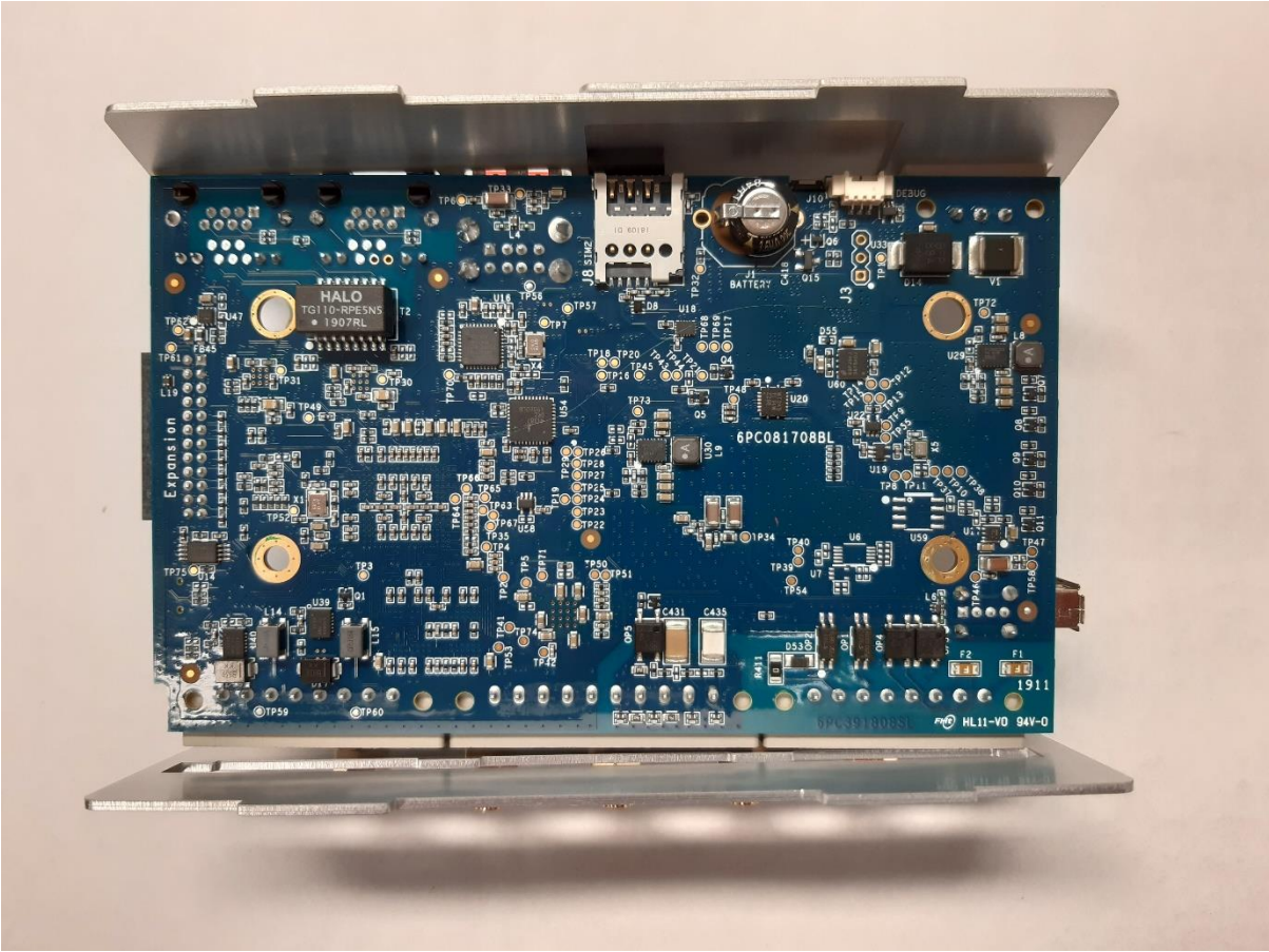
PCB Bottom Side
