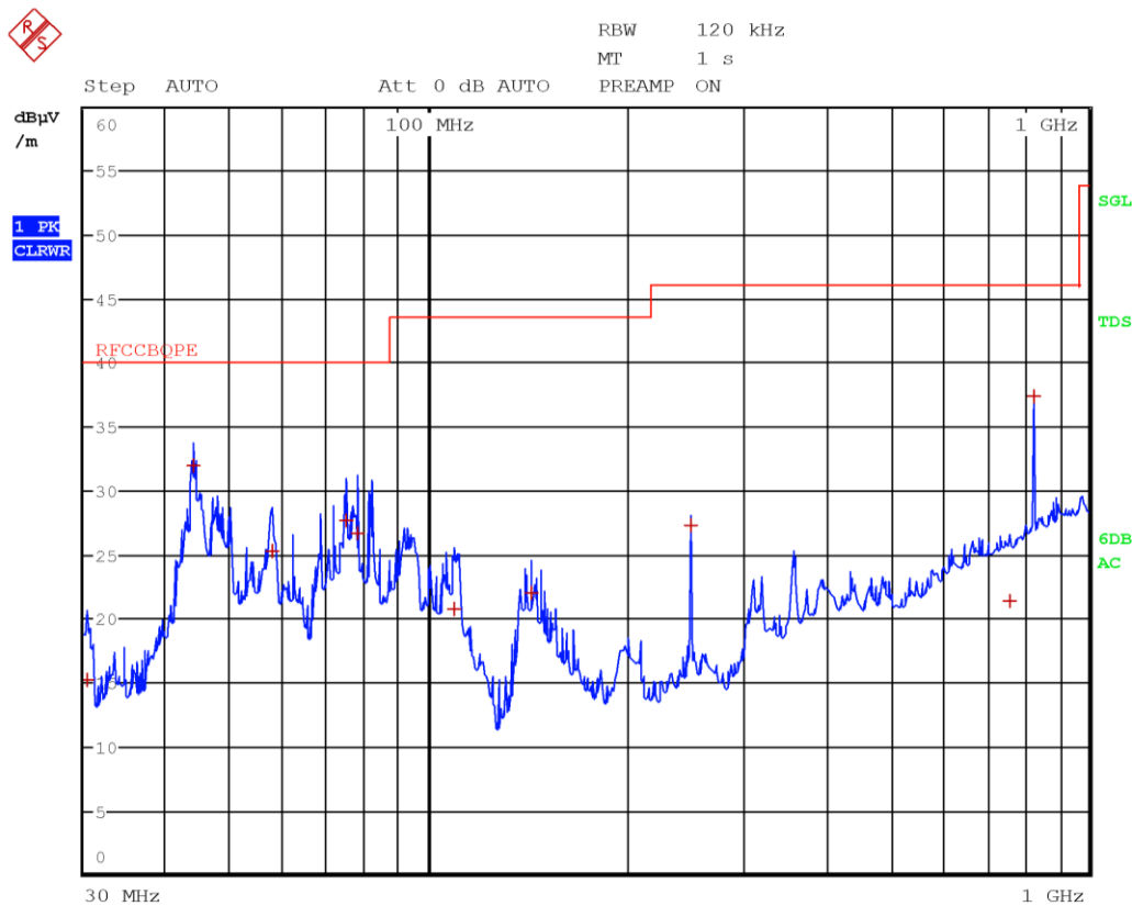
Figure 8.7-30: Radiated spurious emissions 30 to 1000 MHz, High channel with antenna in vertical polarization
