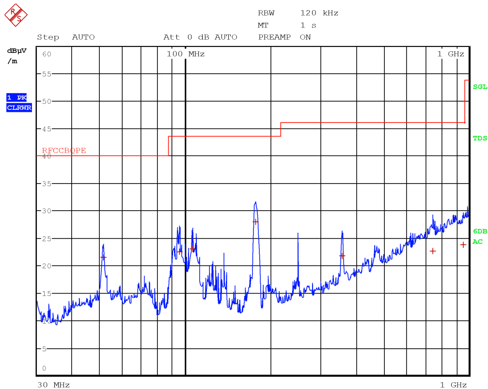
Figure 8.1-153: Radiated spurious emissions, LTE Tx at 1883 MHz, WIFI Tx at 2412 MHz – antenna in horizontal polarization – EUT in configuration 2
