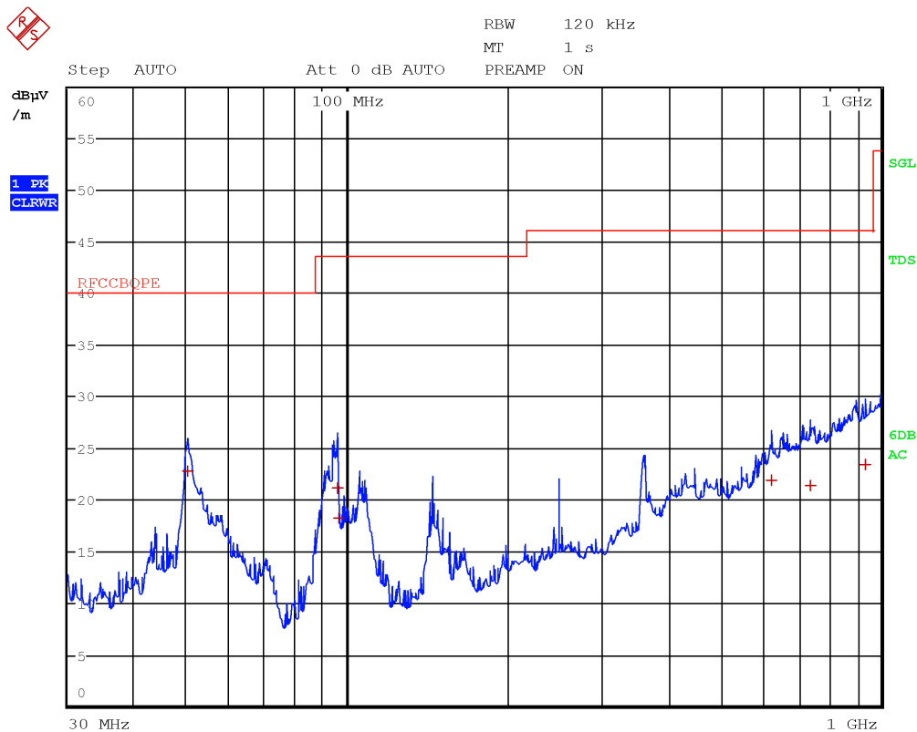
Figure 8.1-121: Radiated spurious emissions, LTE Tx at 1883 MHz, WIFI Tx at 2412 MHz – antenna in horizontal polarization – EUT in configuration 1
