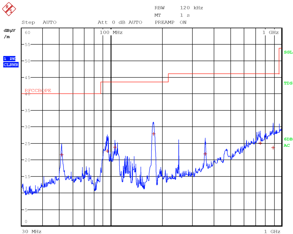
Figure 8.1-161: Radiated spurious emissions, LTE Tx at 1883 MHz, WIFI Tx at 5200 MHz – antenna in horizontal polarization – EUT in configuration 2
