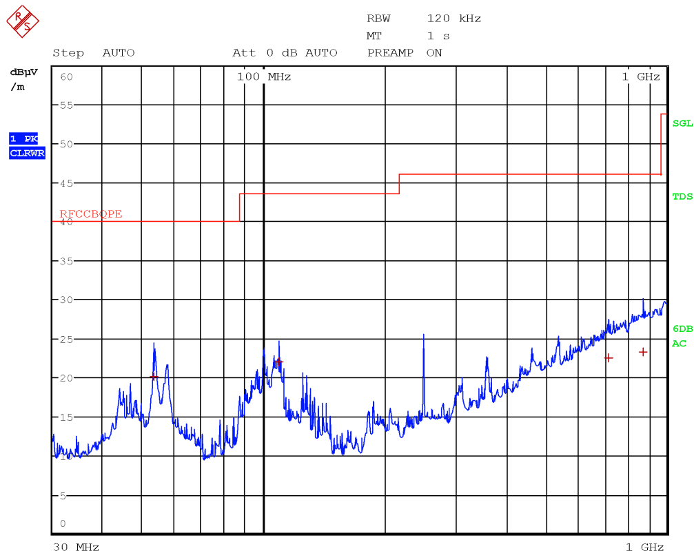
Figure 8.1-185: Radiated spurious emissions, LTE Tx at 1883 MHz, WIFI Tx at 2412 MHz – antenna in horizontal polarization – EUT in configuration 3
