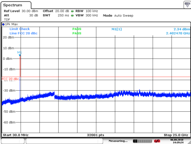
Figure 8.7-12: Conducted spurious emissions outside restricted band, Low channel, \pi/4 -DWPSK
