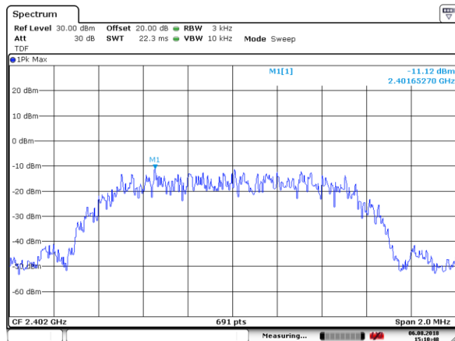
Figure 8.8-2: PSD sample plot on \pi/4 -DWPSK
