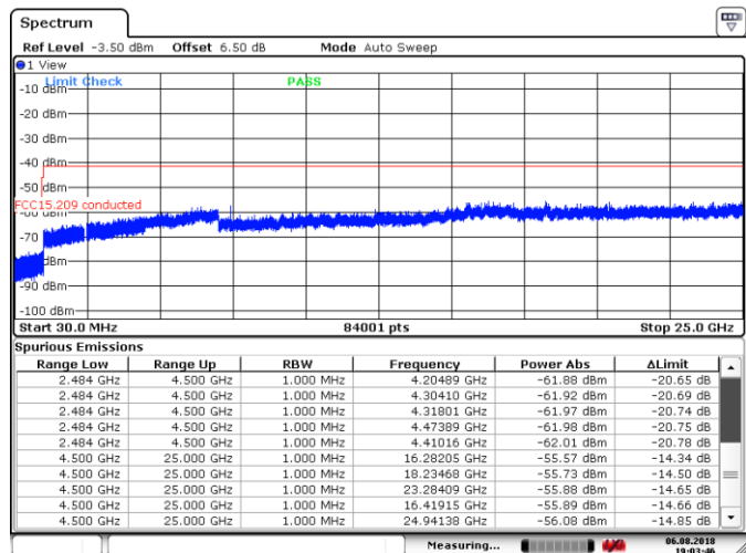
Figure 8.7-23: Conducted spurious emissions within restricted band, High channel, GFSK
