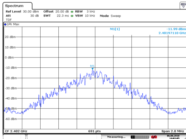
Figure 8.8-1: PSD sample plot on GFSK
