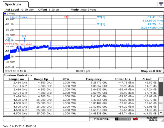
Figure 8.7-25: Conducted spurious emissions within restricted band, Mid channel, \pi/4 -DWPSK
