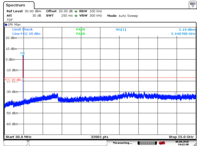
Figure 8.7-16: Conducted spurious emissions outside restricted band, Mid channel, 8DPSK
