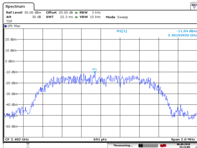
Figure 8.8-3: PSD sample plot on 8-DPSK
