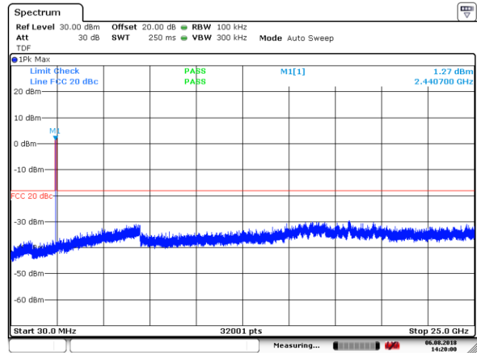
Figure 8.7-13: Conducted spurious emissions outside restricted band, Mid channel, \pi/4 -DWPSK
