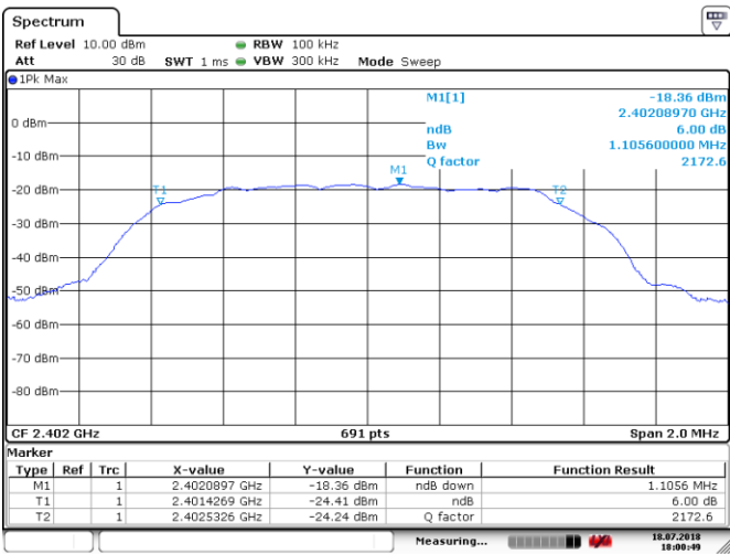
Figure 8.5-3: 6 dB bandwidth of 8-DPSK, sample plot
