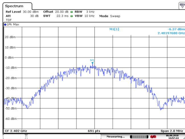
Figure 8.8-4: PSD sample plot on BLE
