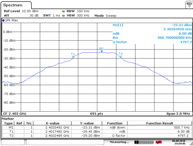
Figure 8.5-1: 6 dB bandwidth of GFSK, sample plot
