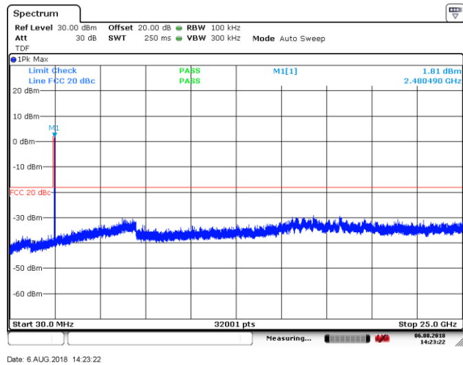
Figure 8.7-17: Conducted spurious emissions outside restricted band, High channel, 8DPSK
