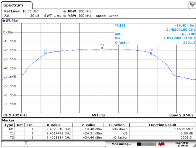
Figure 8.5-2: 6 dB bandwidth of \pi/4 -DWPSK, sample plot
