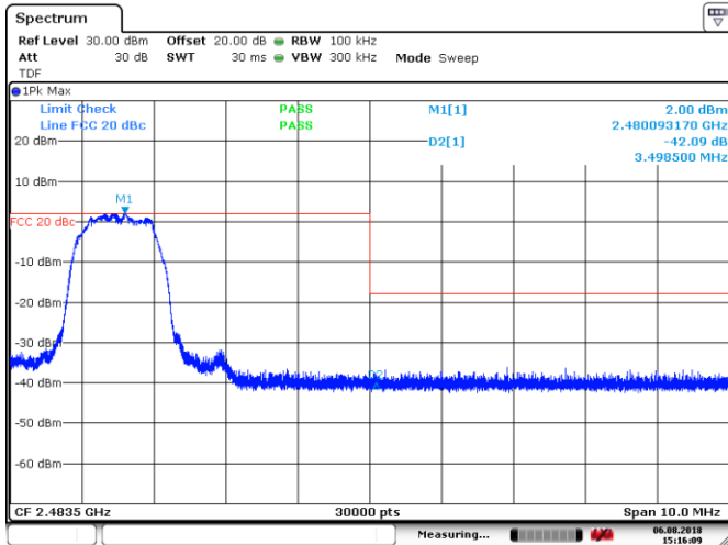
Figure 8.7-6: Conducted spurious emissions at band edge outside restricted band, High channel, 8DPSK
