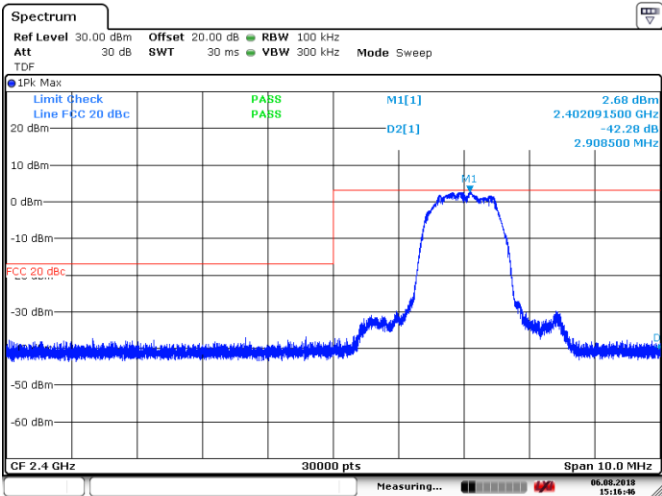
Figure 8.7-5: Conducted spurious emission at band edge outside restricted band, low channel, 8DPSK
