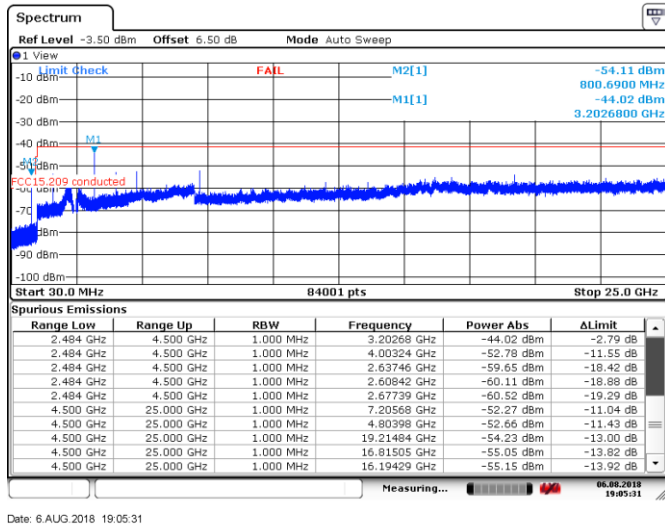
Figure 8.7-24: Conducted spurious emissions within restricted band, Low channel, \pi/4 -DWPSK
