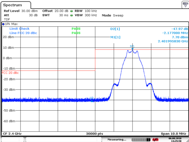
Figure 8.7-7: Conducted spurious emission at band edge outside restricted band, low channel, BLE
