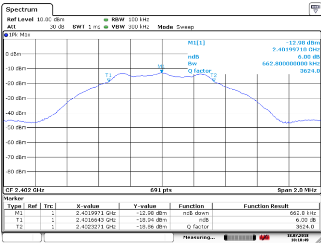
Figure 8.5-4: 6 dB bandwidth of BLE, sample plot
