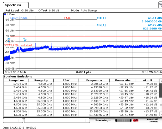
Figure 8.7-26: Conducted spurious emissions within restricted band, High channel, \pi/4 -DWPSK
