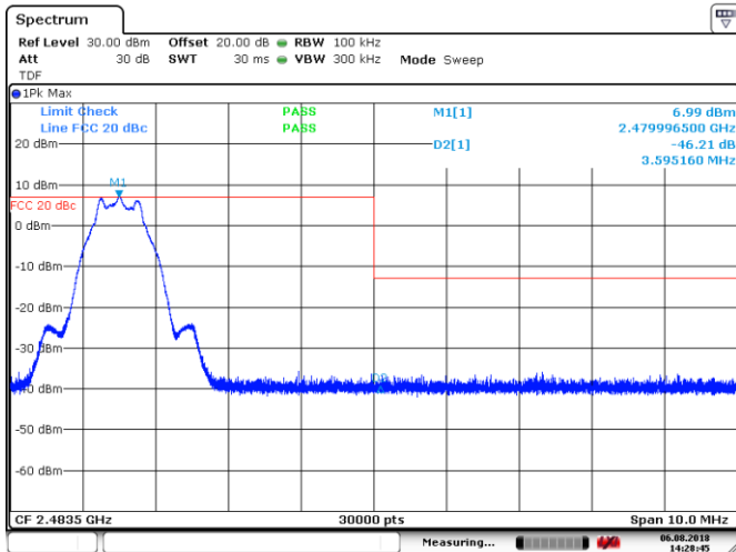
Figure 8.7-8: Conducted spurious emissions at band edge outside restricted band, High channel, BLE
