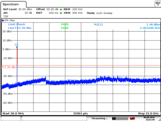
Figure 8.7-15: Conducted spurious emissions outside restricted band, Low channel, 8DPSK
