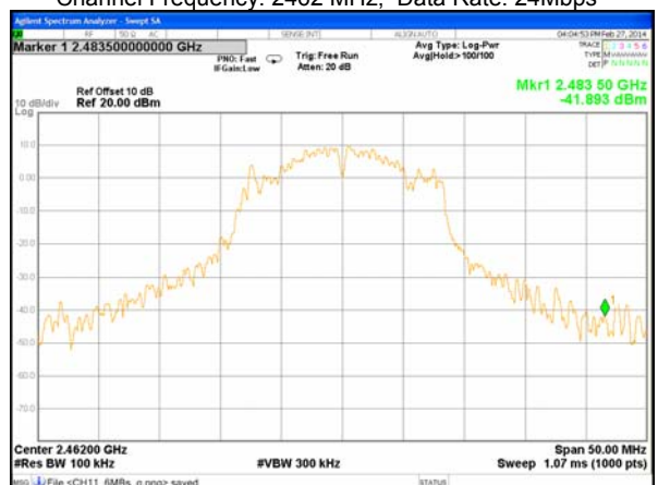
Channel Frequency: 2462 MHz, Data Rate: 24Mbps
