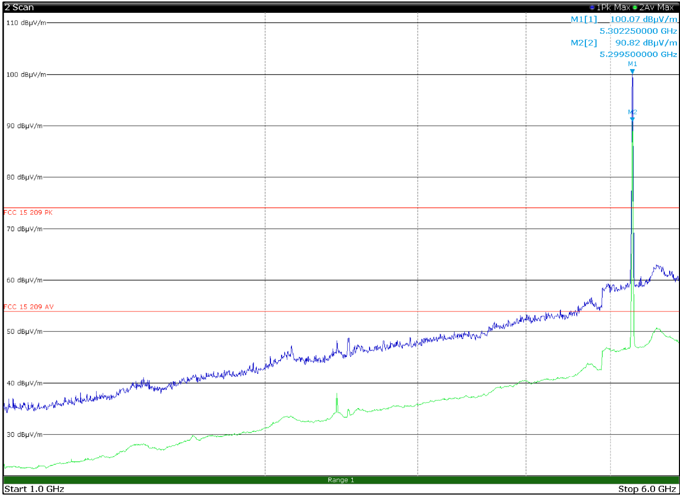
Radiated spurious emissions 1 to 6 GHz, TX 5300 MHz, CH60, 802.11n (20MHz), 6.5Mbps, multi chain with antenna in horizontal polarization
