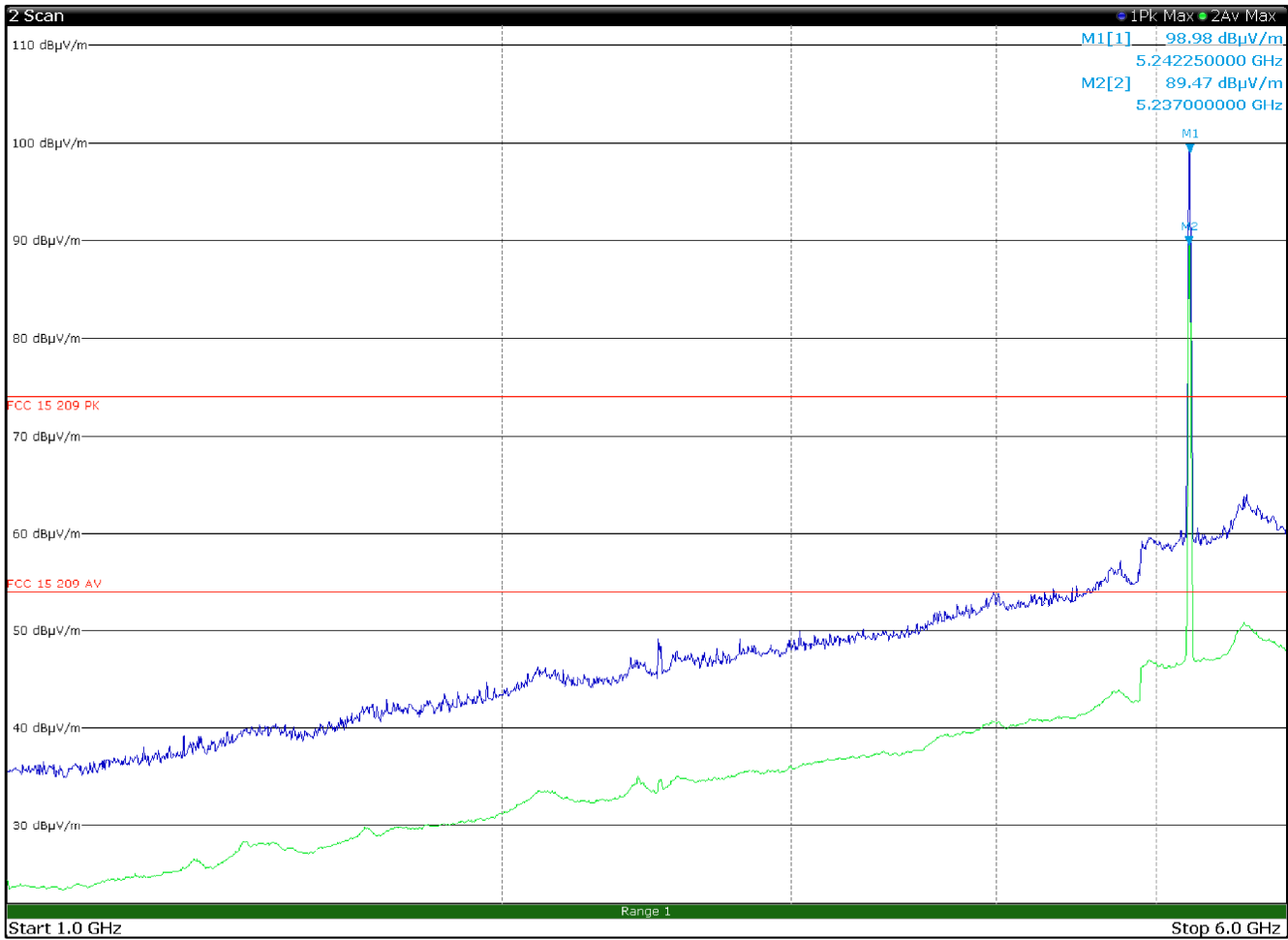
Radiated spurious emissions 1 to 6 GHz, TX 5240 MHz, CH48, 802.11n (20MHz), 6.5Mbps, multi chain with antenna in horizontal polarization
