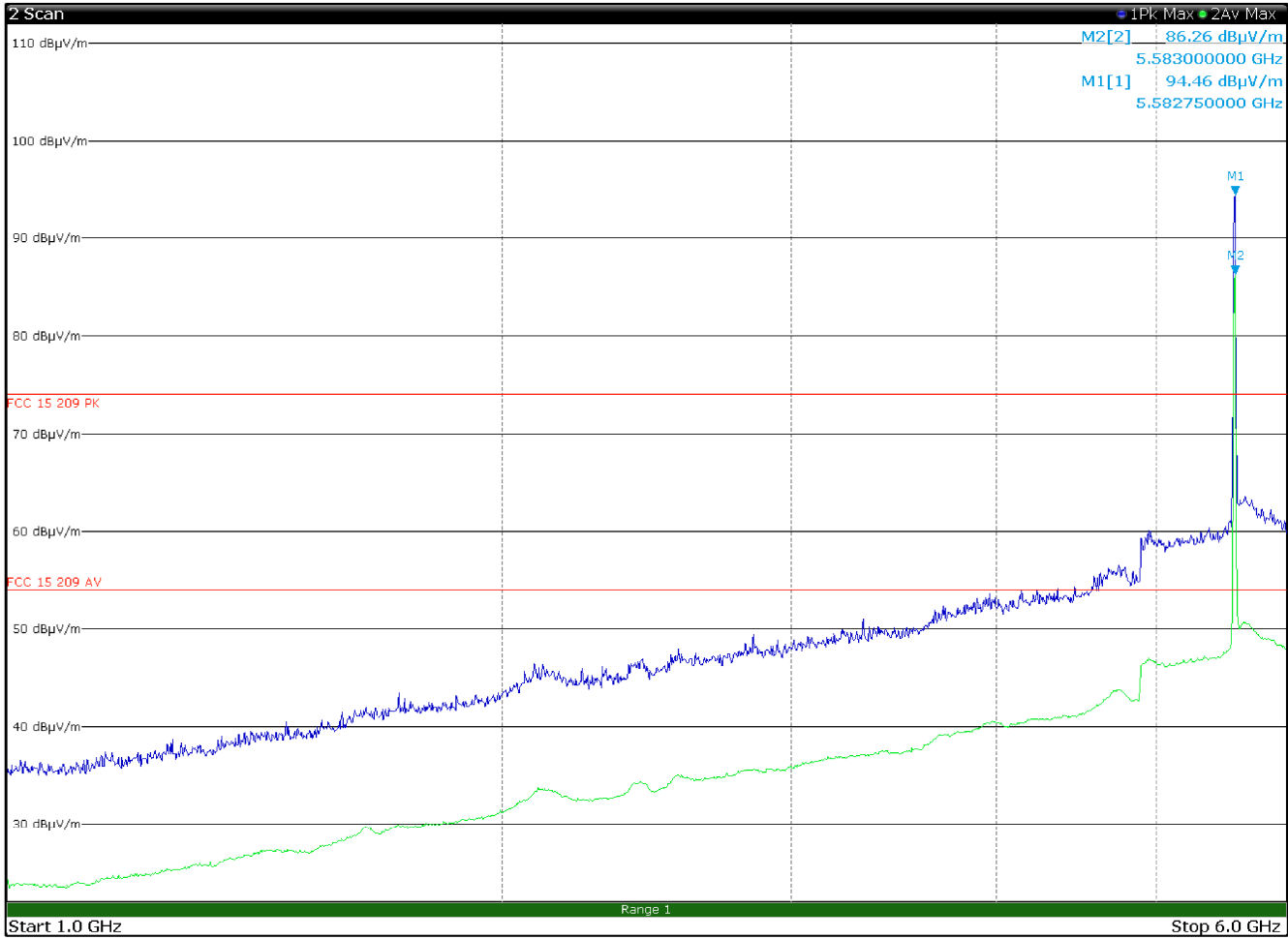
Radiated spurious emissions 1 to 6 GHz, TX 5580 MHz, CH116, 802.11n (20MHz), 6.5Mbps, multi chain with antenna in vertical polarization
