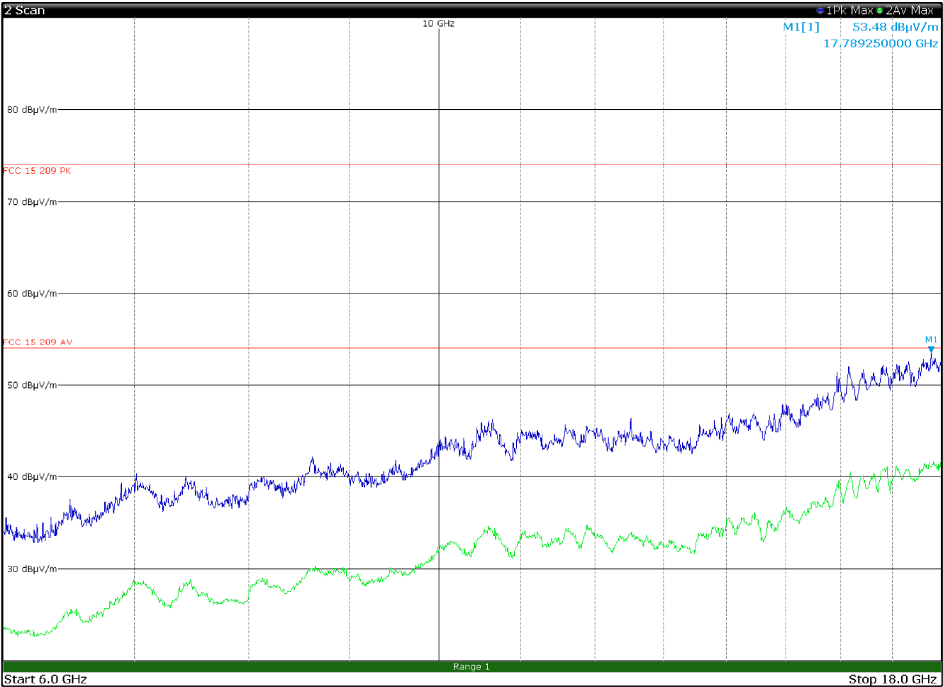
TX 5320 MHz, CH64, 802.11a, 6Mbps, single chain with antenna in vertical polarization
