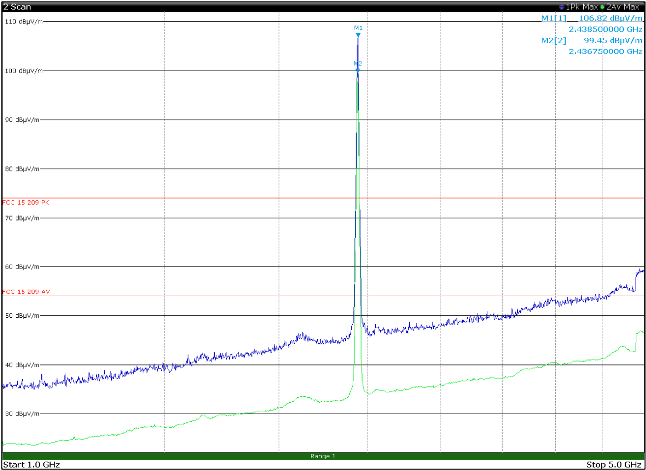
Radiated spurious emissions 1 to 5 GHz, TX 2437 MHz, CH06, 802.11n (20MHz), 6.5Mbps, multiple chainwith antenna in horizontal polarization
