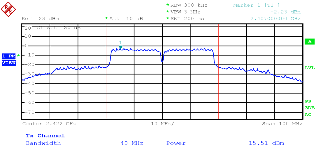
Output power TX 2422 MHz, 802.11 nHT40 13.5 Mbps, multiple chain, chain 1
