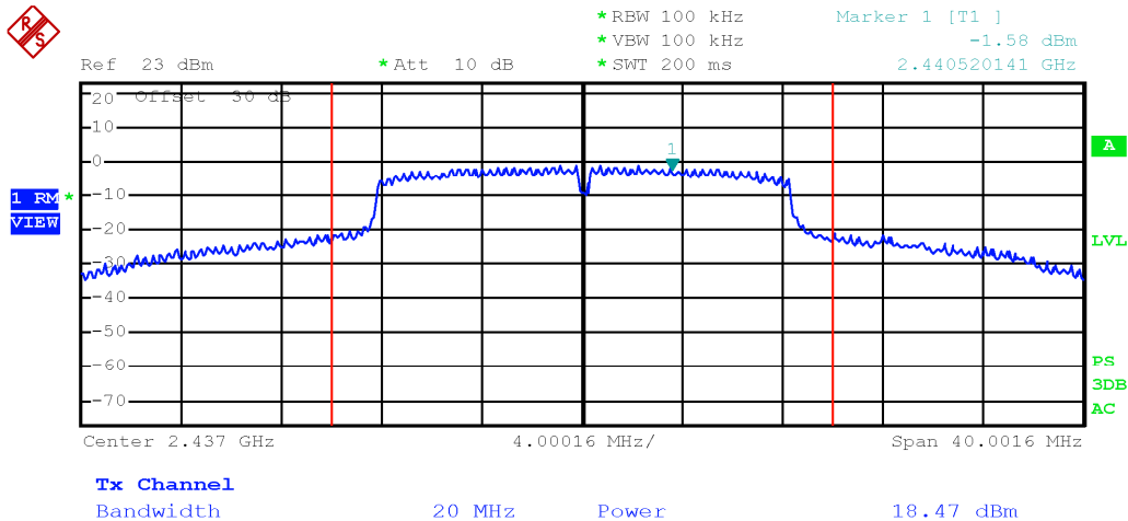
Output power TX 2437 MHz, 802.11 nHT20 6.5 Mbps, multiple chain, chain 1
