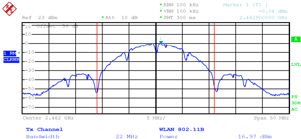
Output power TX 2462 MHz, 802.11b, 1 Mbps, multiple chain, chain 0
