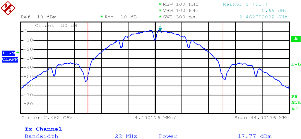
Output power TX 2462 MHz, 802.11b, 1 Mbps, single chain
