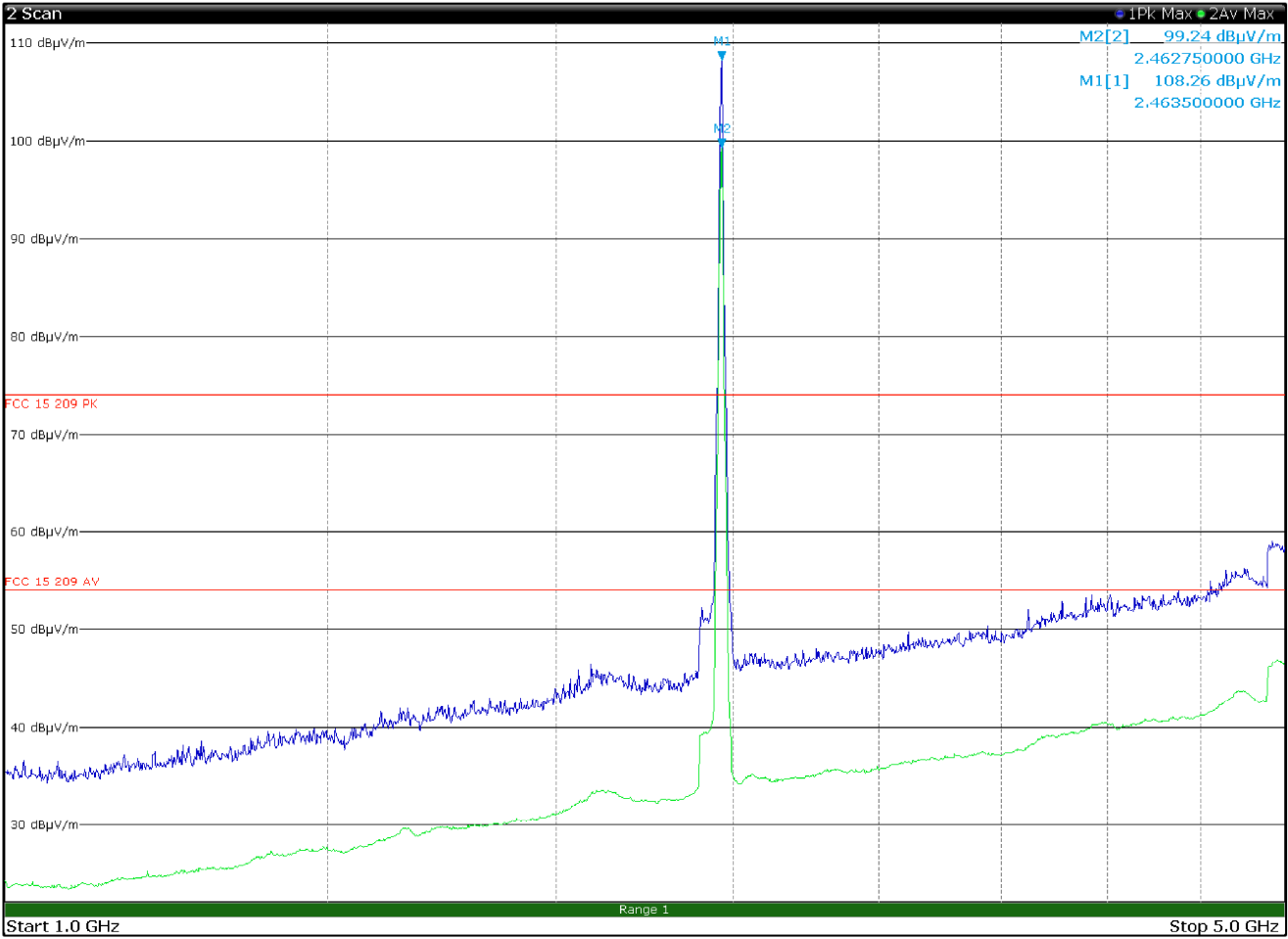
Radiated spurious emissions 1 to 5 GHz, TX 2462 MHz, CH11, 802.11n (20MHz), 6.5Mbps, multiple chain with antenna in horizontal polarization
