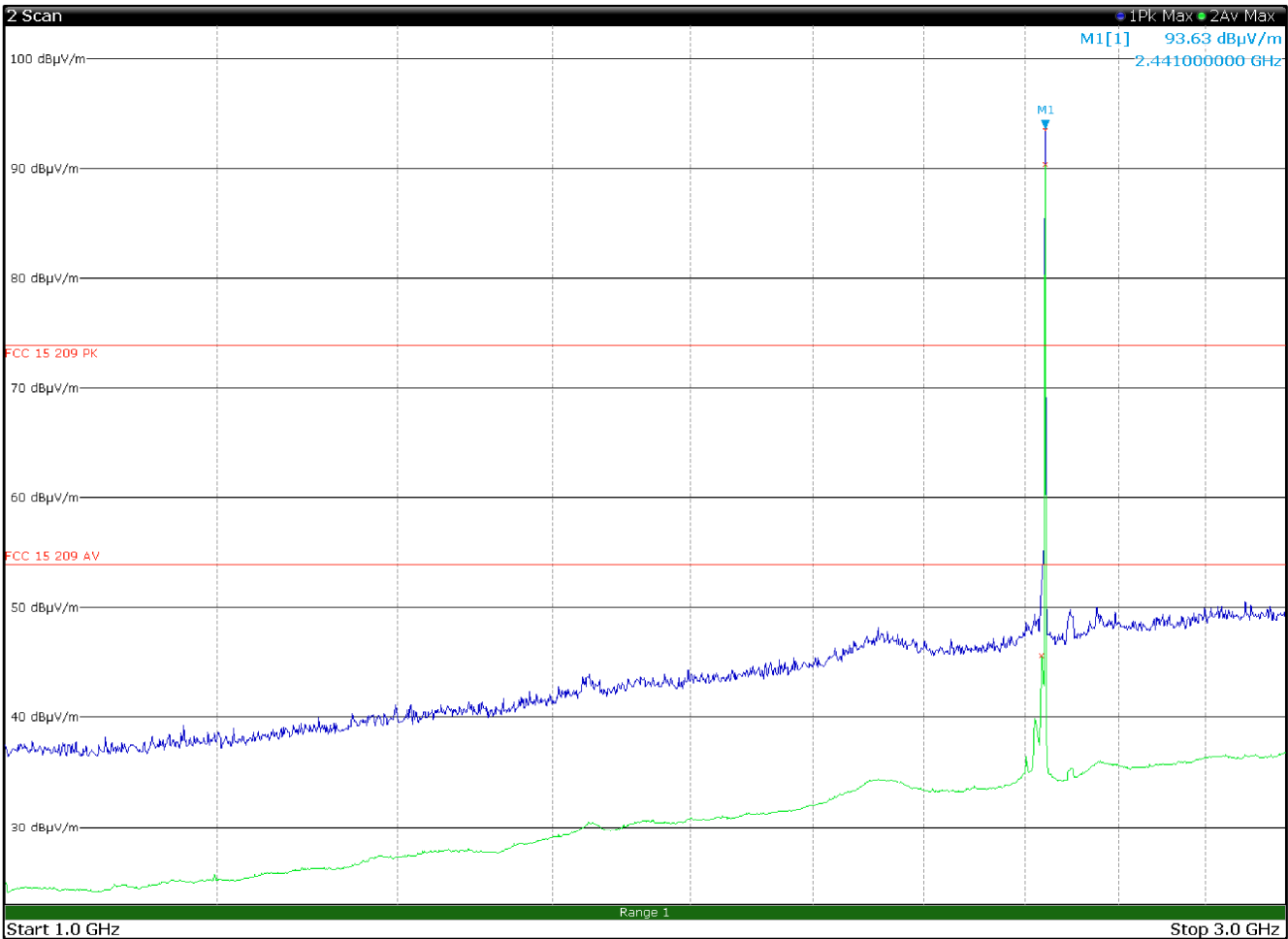
Radiated spurious emissions 1 to 3GHz, TX 2441 MHz, CH 00, 8DPSK MODULATION with antenna in horizontal polarization
