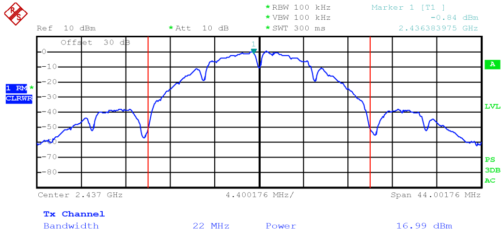
Output power TX 2437 MHz, 802.11b, 1 Mbps, single chain
