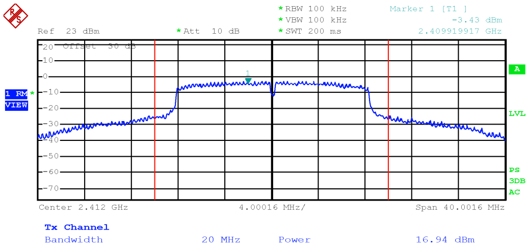
Output power TX 2412 MHz, 802.11 nHT20 6.5 Mbps, multiple chain, chain 0
