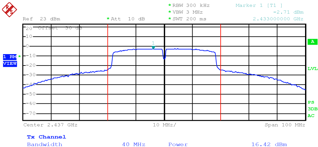
Output power TX 2437MHz, 802.11 nHT40 13.5 Mbps, multiple chain, chain 0
