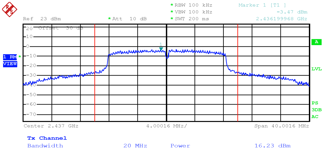
Output power TX 2437 MHz, 802.11 nHT20 6.5 Mbps, multiple chain, chain 0
