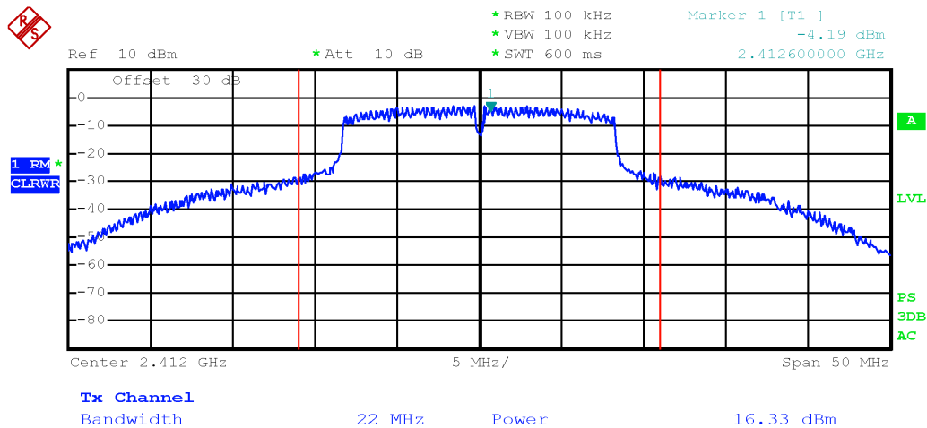
Output power TX 2412 MHz, 802.11g, 6 Mbps, single chain
