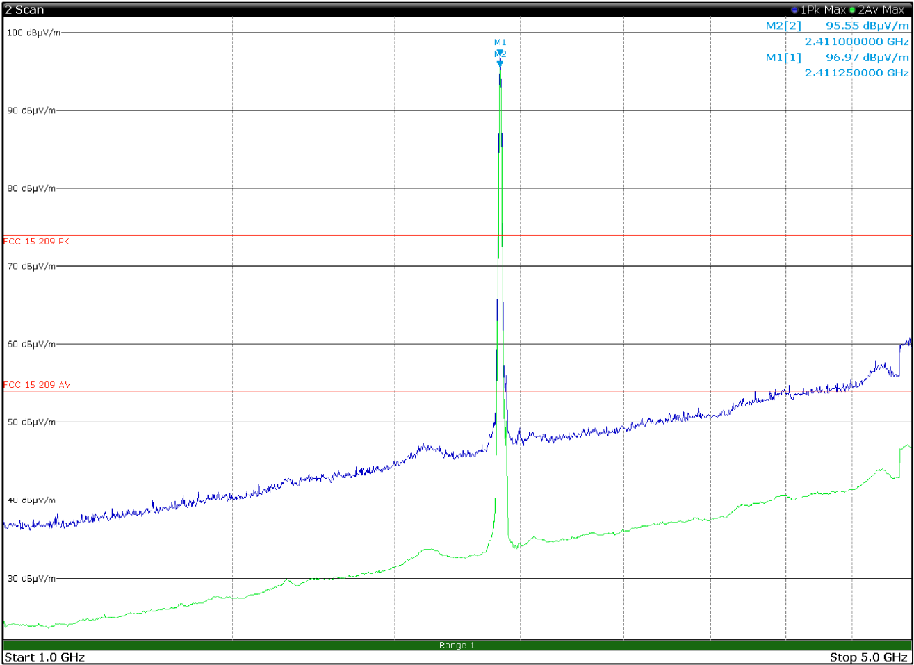
Radiated spurious emissions 1 to 5 GHz, Low channel with antenna in horizontal polarization, TX 2412 MHz, CH01, 802.11b, 1Mbps, multiple chain
