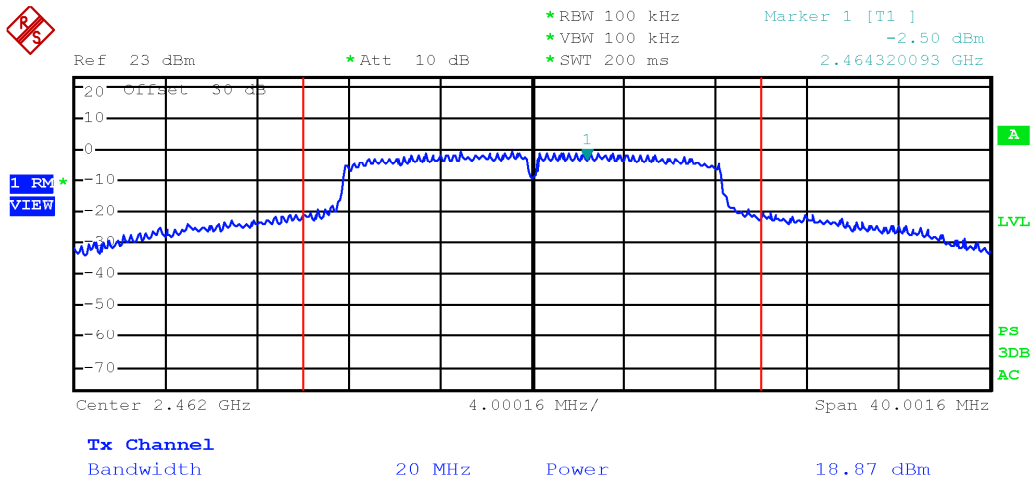
Output power TX 2462 MHz, 802.11 nHT20 6.5 Mbps, multiple chain, chain 1
