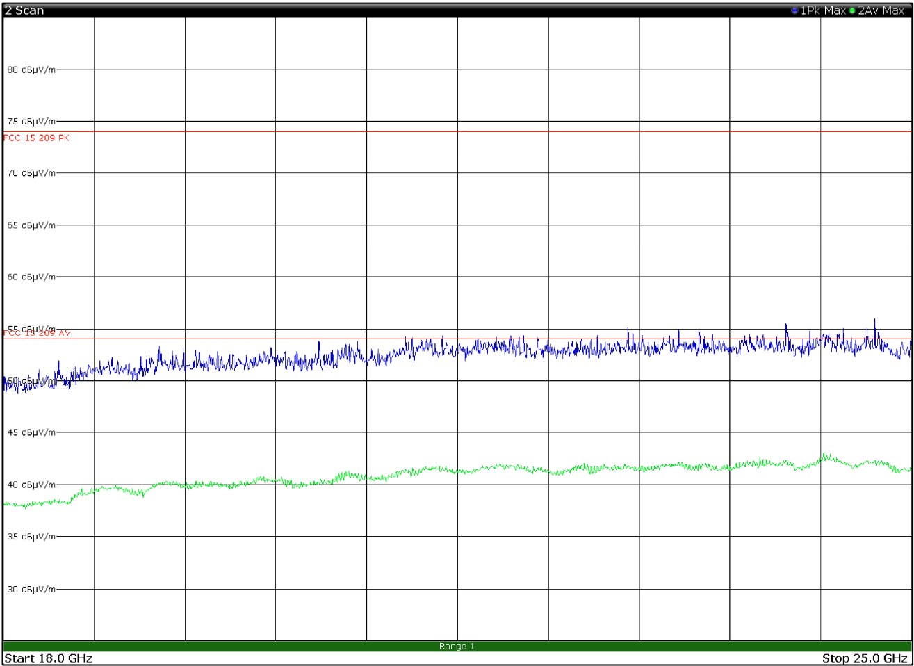
Radiated spurious emissions 18 to 25 GHz, TX 2441MHz, 8DPSK MODULATION with antenna in vertical polarization
