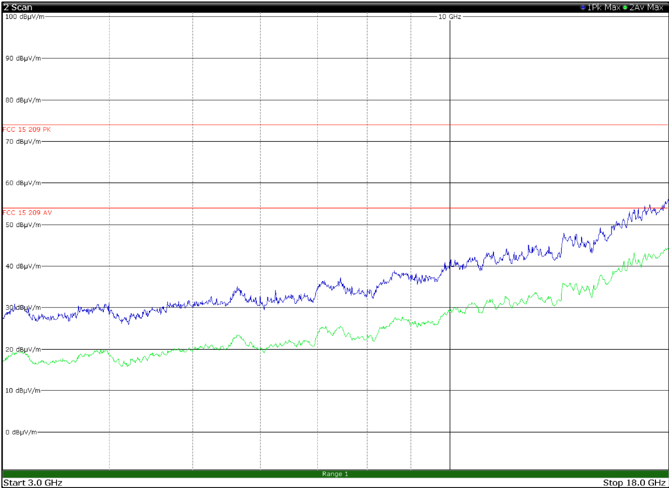
Radiated spurious emissions 3 to 18GHz, TX 2480 MHz, CH 00, 8DPSK MODULATION with antenna in vertical polarization
