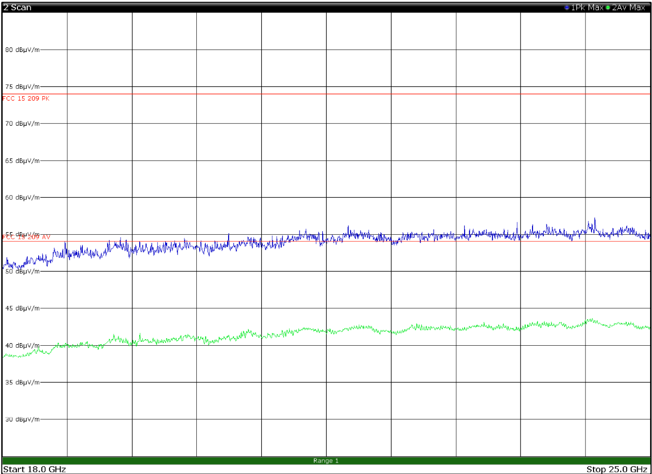
Radiated spurious emissions 18 to 25 GHz, TX 2402MHz, CH 00, 8DPSK MODULATION with antenna in horizontal polarization
