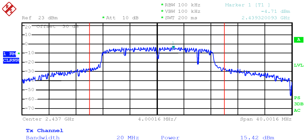
Output power TX 2437MHz, 802.11g, 6 Mbps, multiple chain, chain 0
