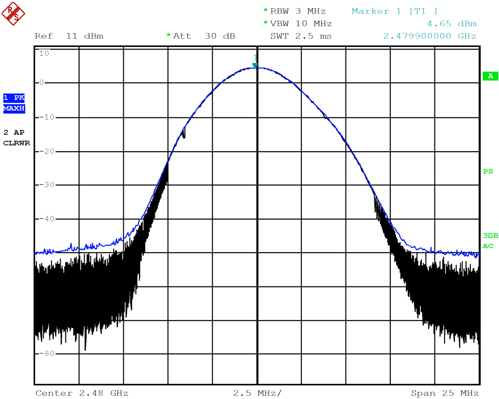
Output power TX 2480MHz, BT 8DPSK
