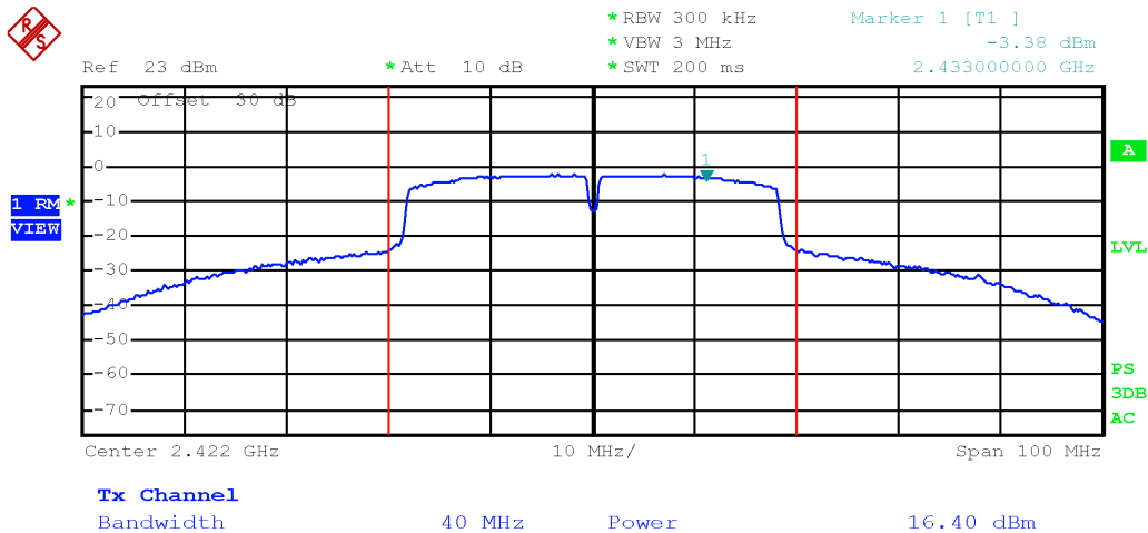
Output power TX 2422 MHz, 802.11 nHT40 13.5 Mbps, multiple chain, chain 0
