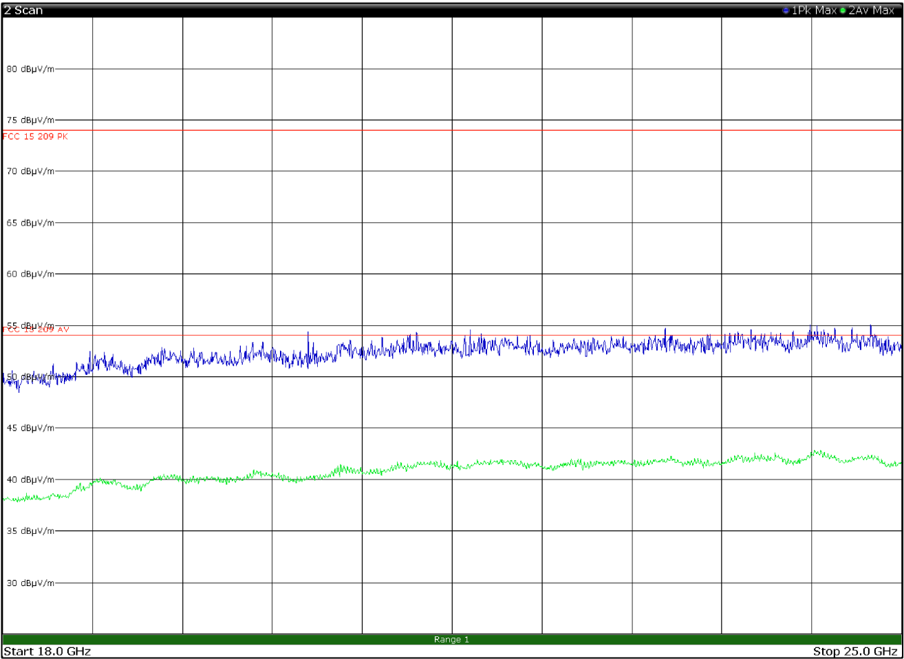
Radiated spurious emissions 18 to 25 GHz TX 2441MHz, 8DPSK MODULATION with antenna in horizontal polarization
