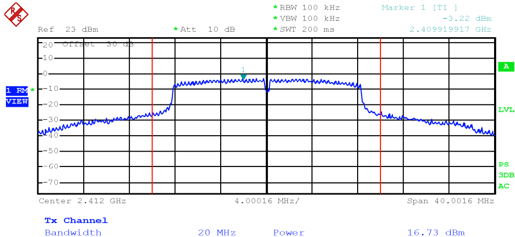
Output power TX 2412 MHz, 802.11g, 6 Mbps, multiple chain, chain 0
