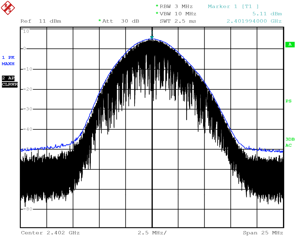
Output power TX 2402MHz, BT 8DPSK
