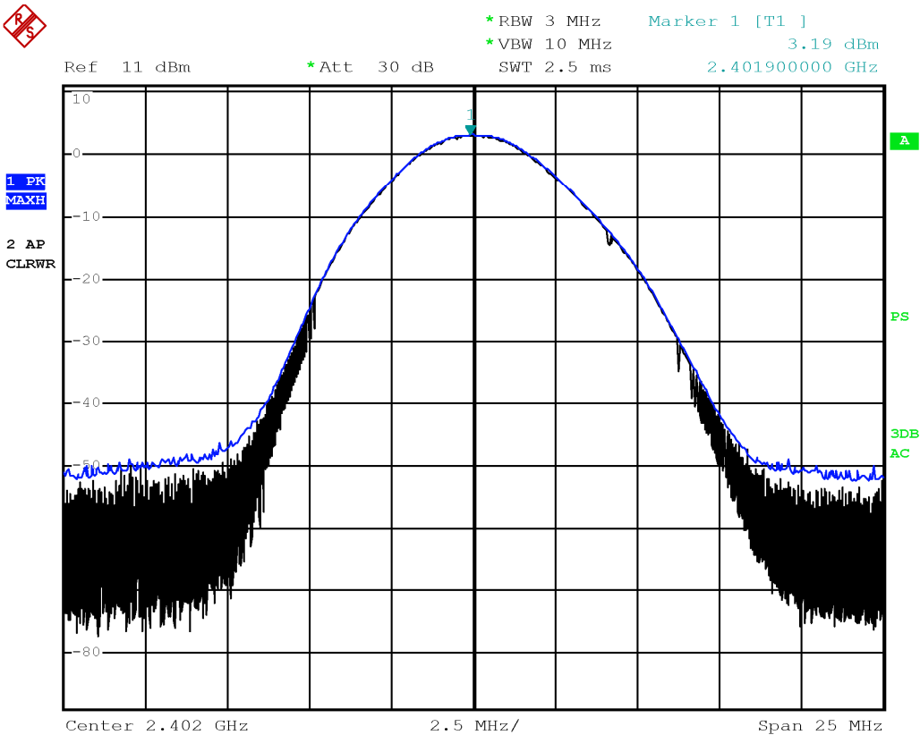
Output power TX 2402MHz, GFSK(LE mode)
