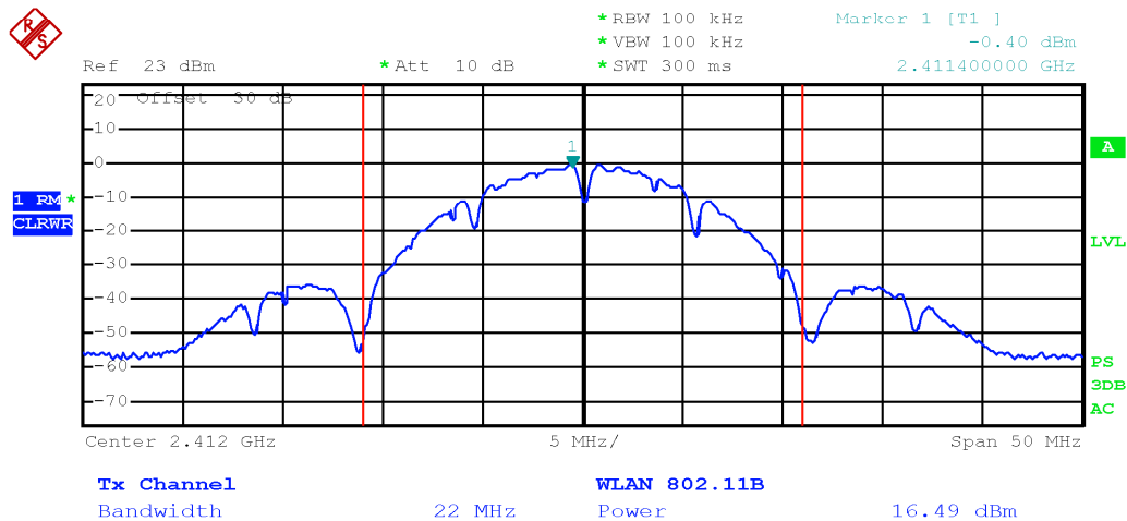
Output power TX 2412 MHz, 802.11b, 1 Mbps, multiple chain, chain 0
