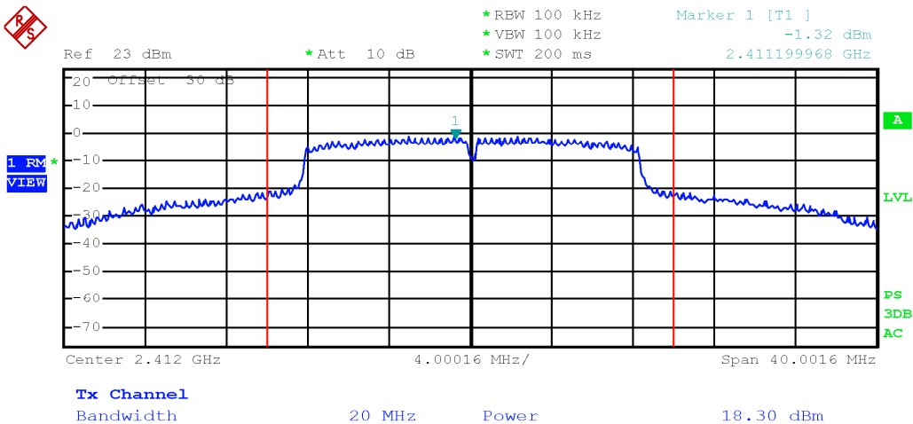
Output power TX 2412 MHz, 802.11 nHT20 6.5 Mbps, multiple chain, chain 1
