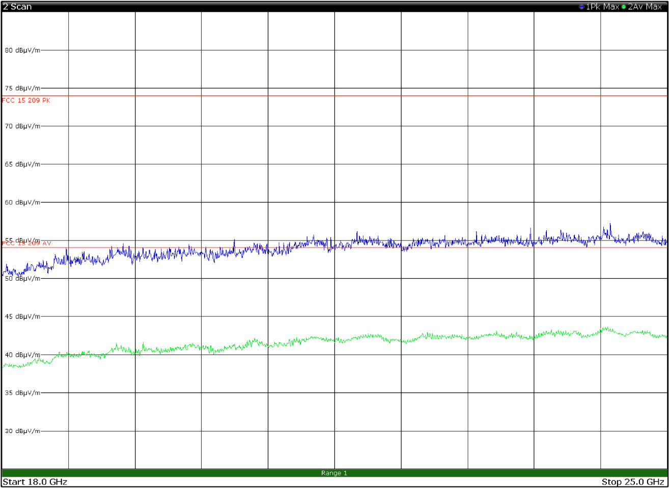
Radiated spurious emissions 18 to 25 GHz, TX 2422 MHz, CH03, 802.11n (40MHz), 13.5Mbps, multiple chain in horizontal polarization
