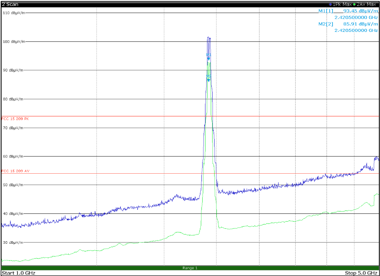
Radiated spurious emissions 1 to 5 GHz, TX 2422 MHz, CH03, 802.11n (40MHz), 13.5Mbps, multiple chain with antenna in vertical polarization
