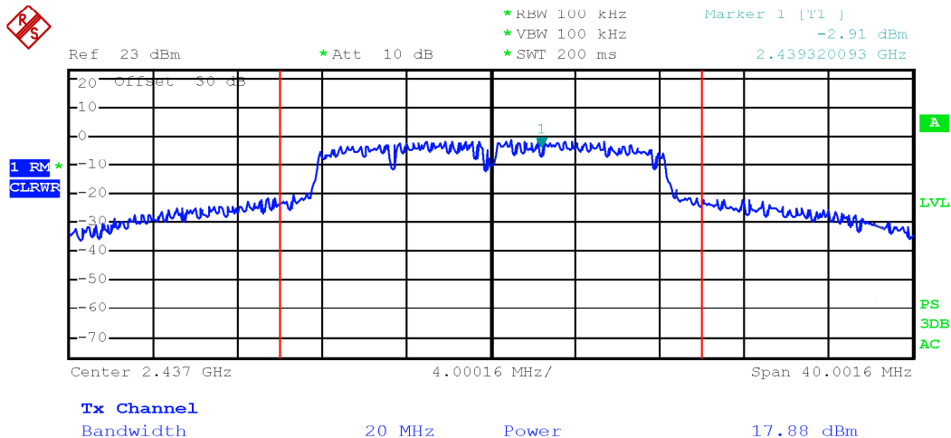
Output power TX 2437MHz, 802.11g, 6 Mbps, multiple chain, chain 1
