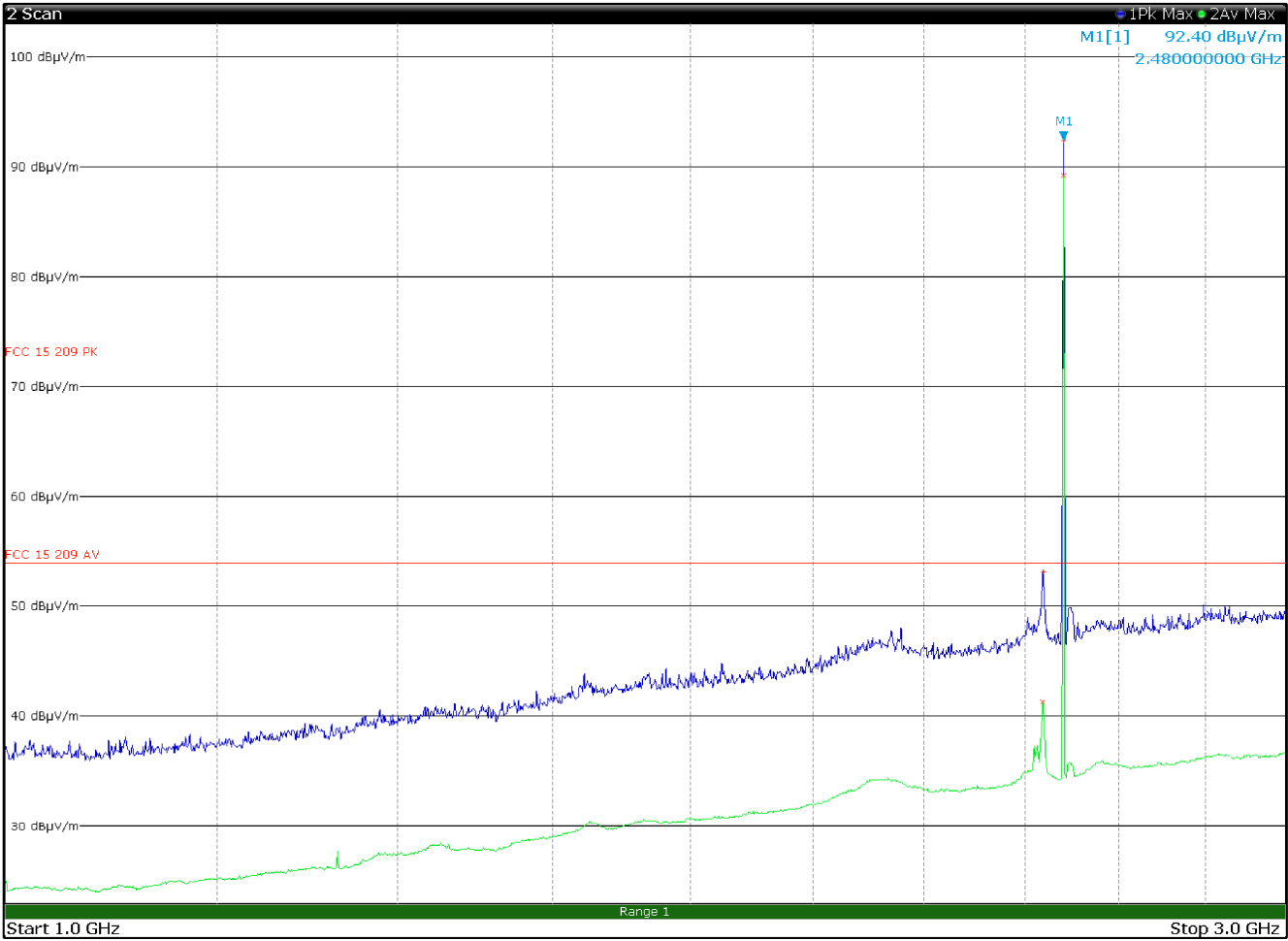
Radiated spurious emissions 1 to 3GHz, TX 2480 MHz, CH 00, 8DPSK MODULATION with antenna in vertical polarization
