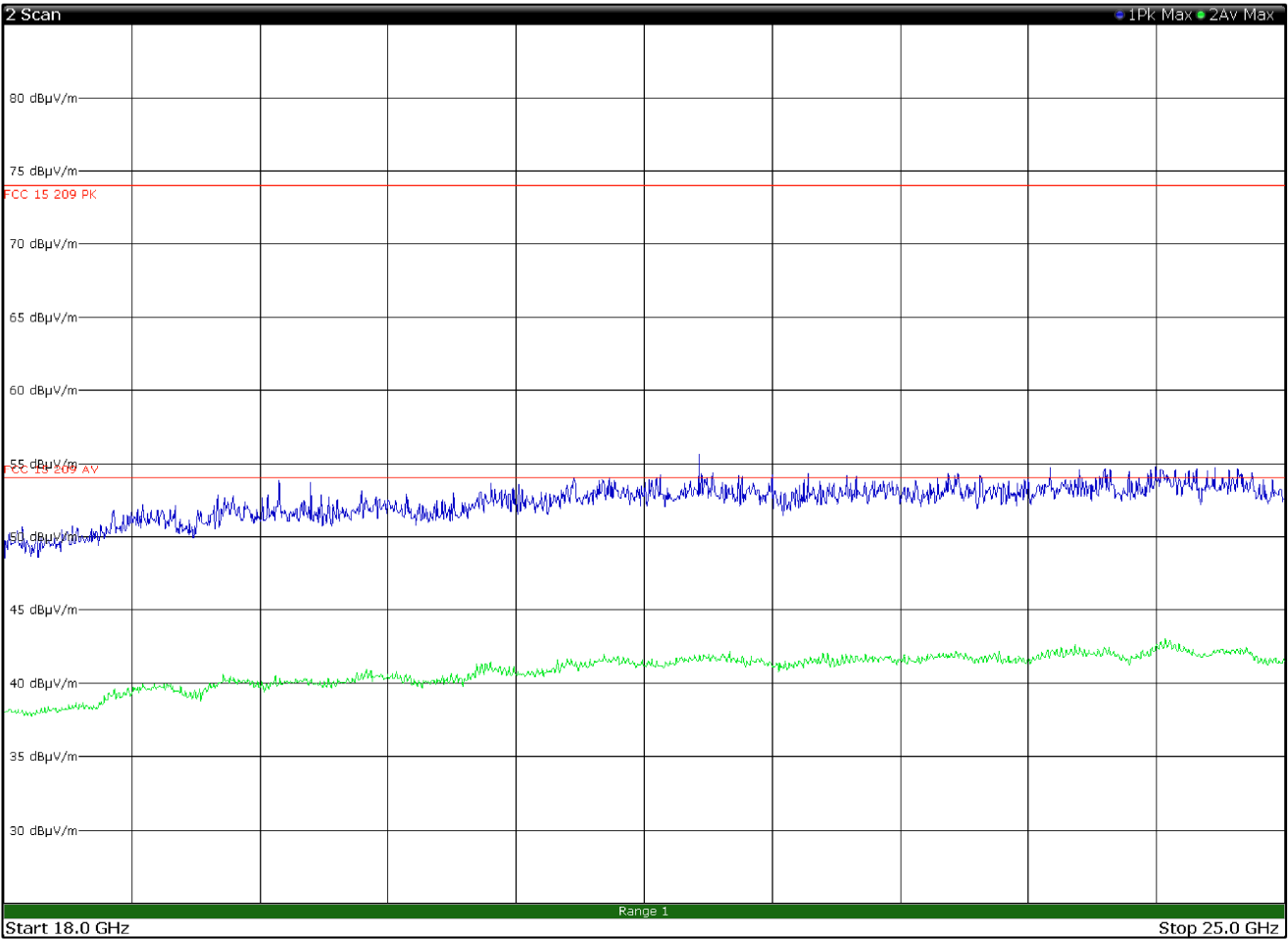
Radiated spurious emissions 18 to 25 GHz, TX 2402MHz, CH 00, 8DPSK MODULATION with antenna in vertical polarization
