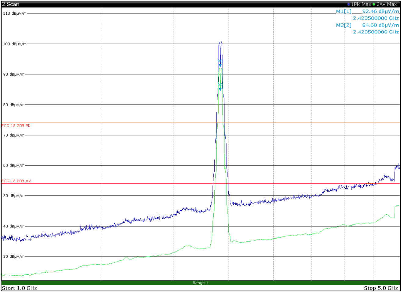
Radiated spurious emissions 1 to 5 GHz, TX 2422 MHz, CH03, 802.11n (40MHz), 13.5Mbps, multiple chain with antenna in horizontal polarization
