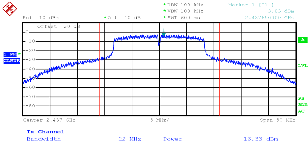
Output power TX 2437MHz, 802.11g, 6 Mbps, single chain
