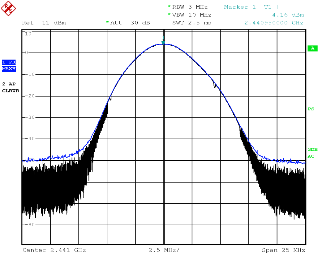
Output power TX 2441MHz, BT GFSK
