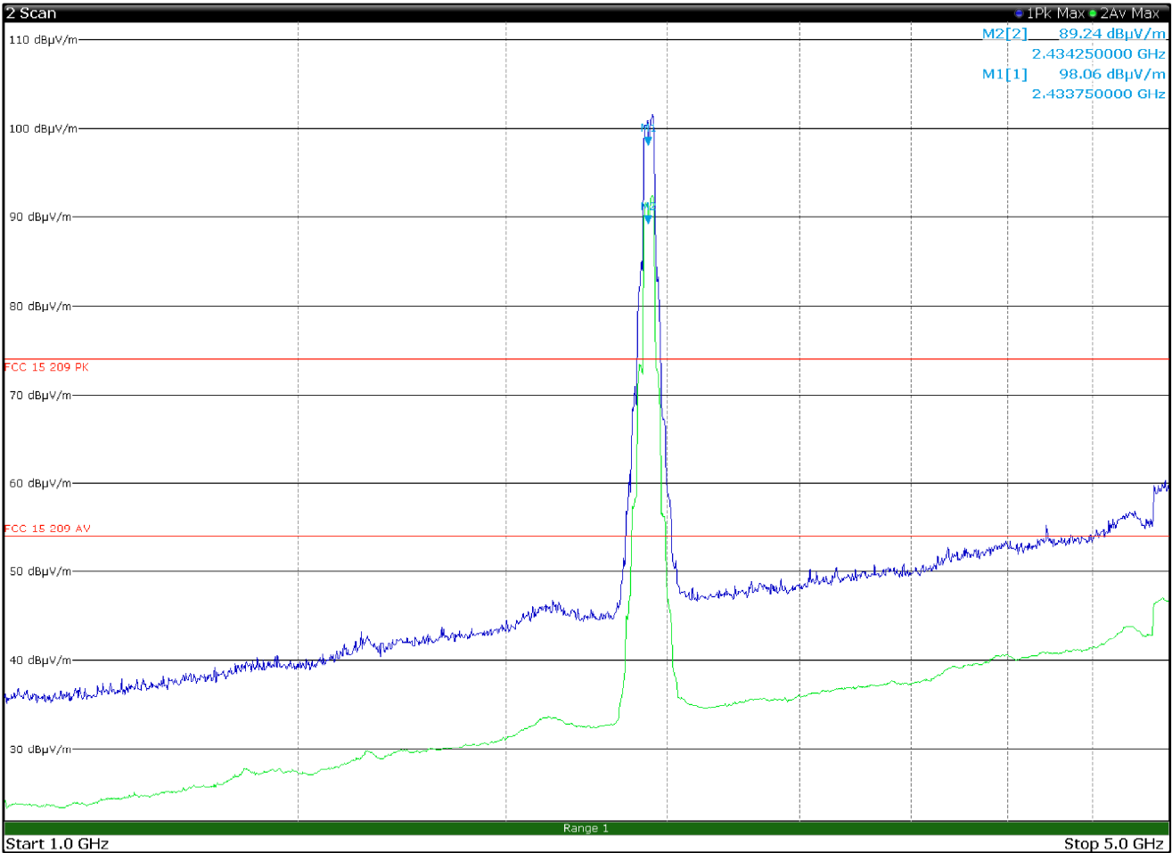
Radiated spurious emissions 1 to 5 GHz, TX 2437 MHz, CH06, 802.11n (40MHz), 13.5Mbps, multiple chain with antenna in horizontal polarization
