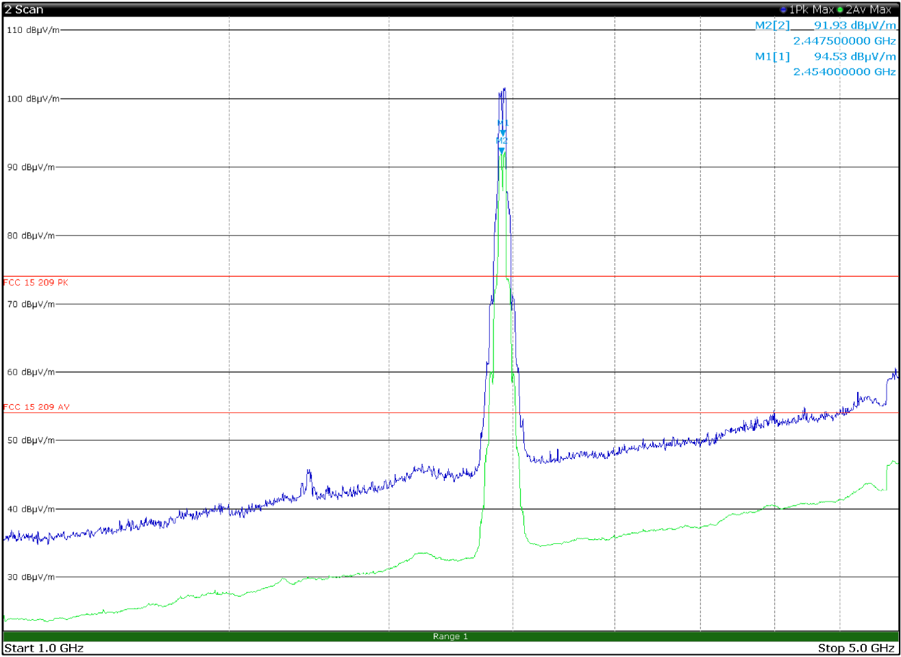
Radiated spurious emissions 1 to 5 GHz, TX 2452 MHz, CH09, 802.11n (40MHz), 13.5Mbps, multiple chain with antenna in horizontal polarization
