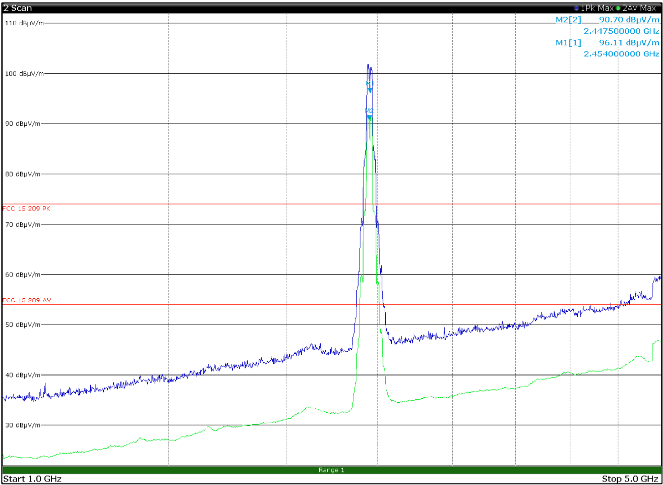
Radiated spurious emissions 1 to 5 GHz, TX 2452 MHz, CH09, 802.11n (40MHz), 13.5Mbps, multiple chain with antenna in vertical polarization
