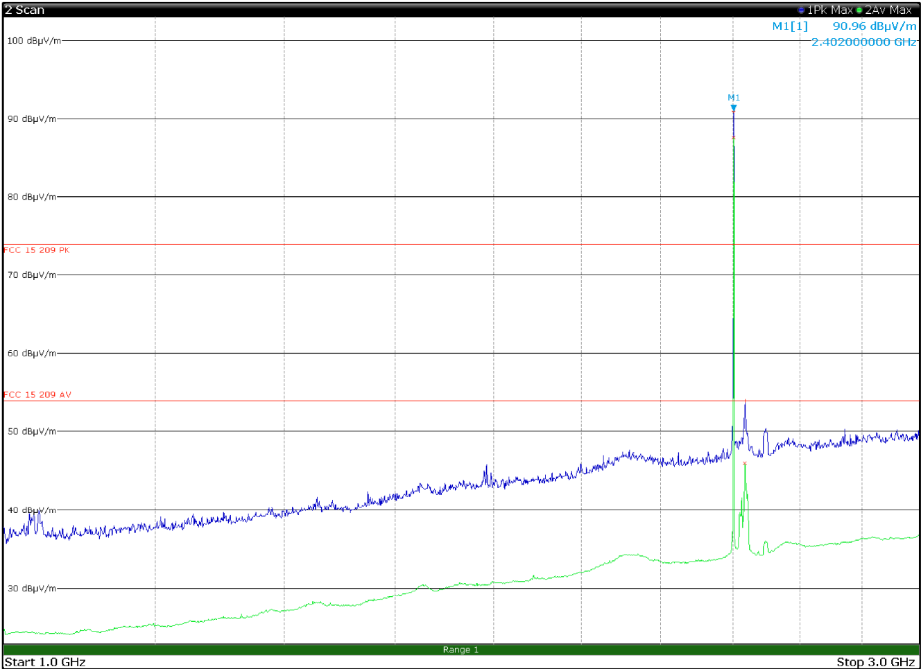
Radiated spurious emissions 1 to 3GHz, TX 2402 MHz, CH 00, 8DPSK MODULATION with antenna in horizontal polarization
