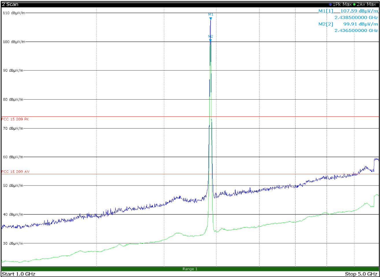
Radiated spurious emissions 1 to 5 GHz, TX 2437 MHz, CH06, 802.11n (20MHz), 6.5Mbps, multiple chain with antenna in vertical polarization
