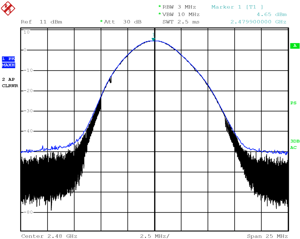
Output power TX 2480MHz, BT GFSK
