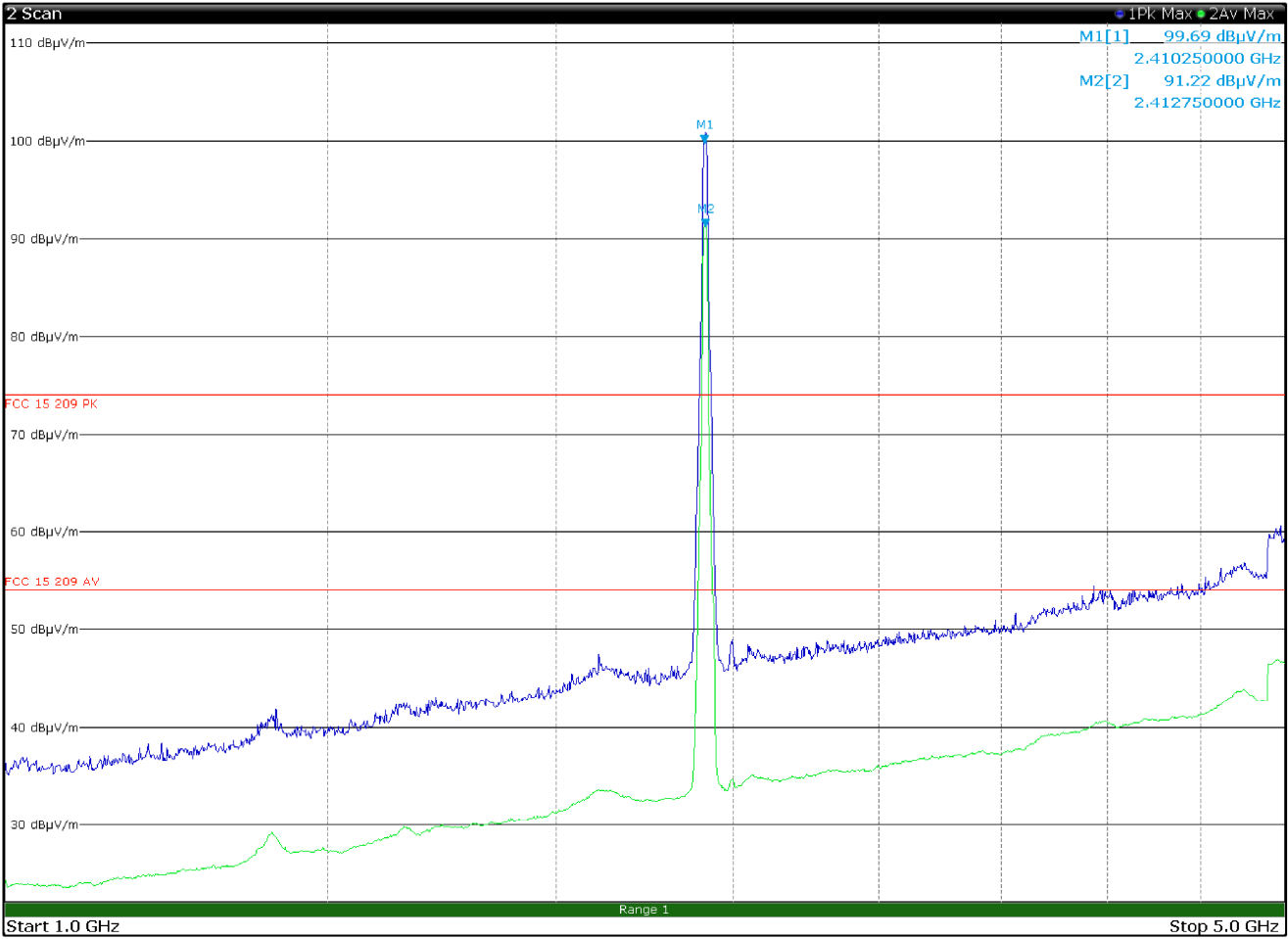
Radiated spurious emissions 1 to 5 GHz, X 2412 MHz, CH01, 802.11g, 6Mbps, multiple chain with antenna in vertical polarization
