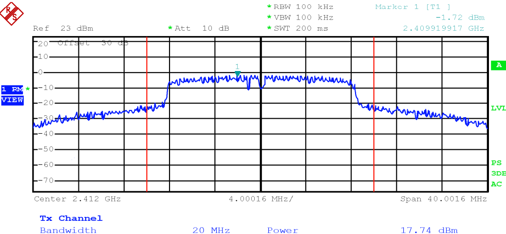
Output power TX 2412 MHz, 802.11g, 6 Mbps, multiple chain, chain 1
