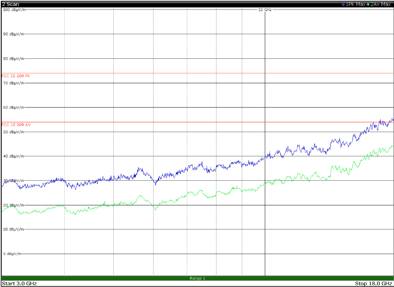
Radiated spurious emissions 3 to 18GHz, TX 2441MHz, CH 00, 8DPSK MODULATION with antenna in vertical polarization
