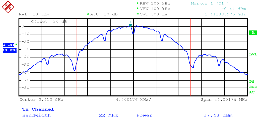
Output power TX 2412 MHz, 802.11b, 1 Mbps, single chain
