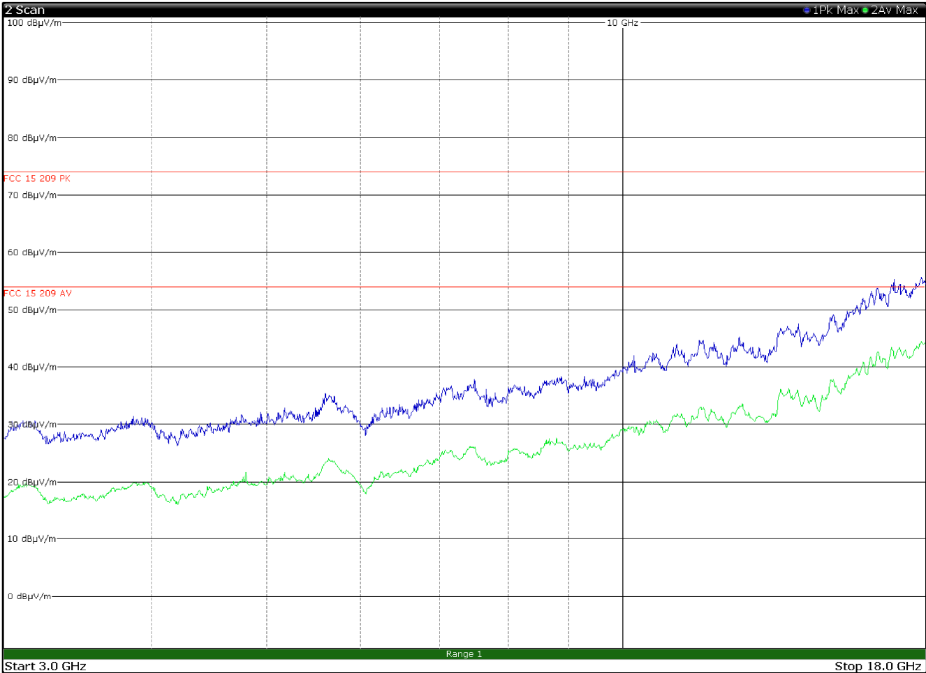
Radiated spurious emissions 3 to 18GHz, TX 2402MHz, CH 00, 8DPSK MODULATION with antenna in vertical polarization
