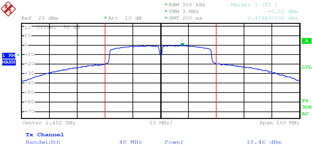
Output power TX 2452 MHz, 802.11 nHT40 13.5 Mbps, multiple chain, chain 1
