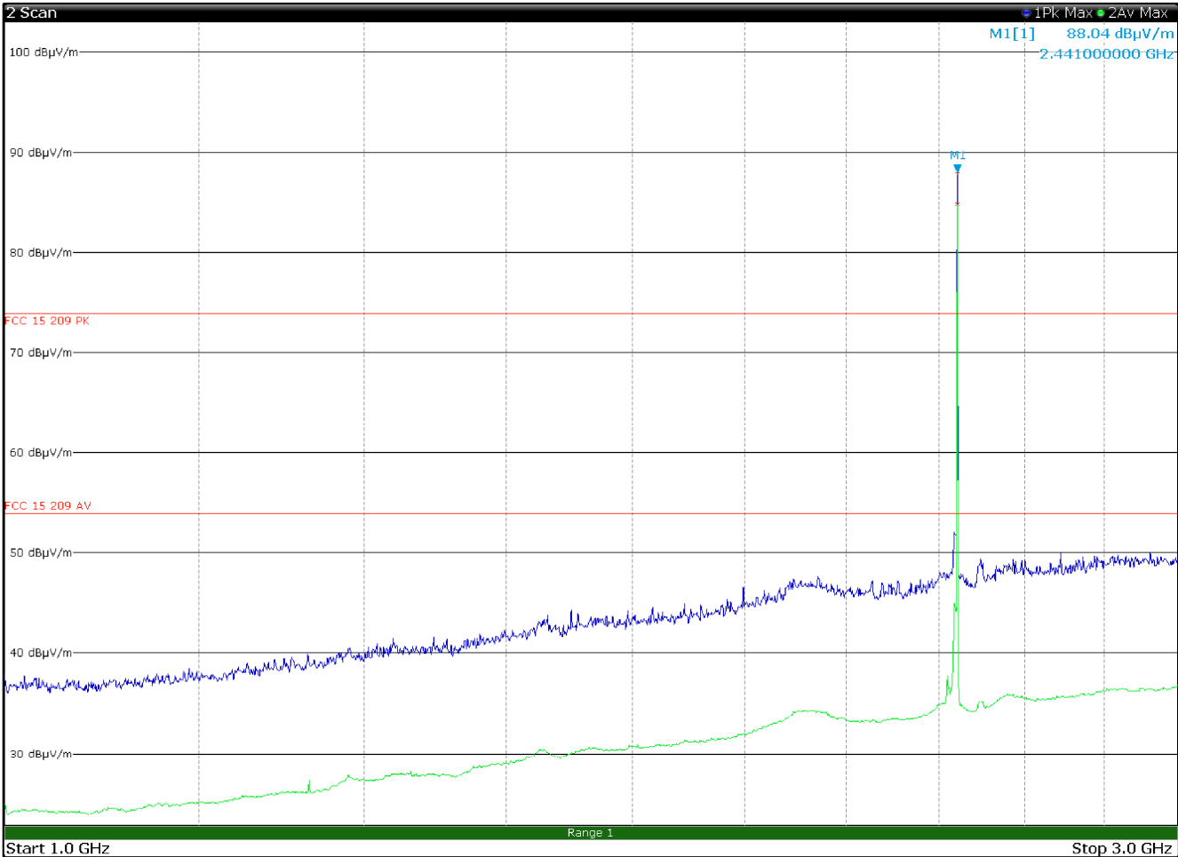
Radiated spurious emissions 1 to 3GHz, TX 2441 MHz, CH 00, 8DPSK MODULATION with antenna in vertical polarization
