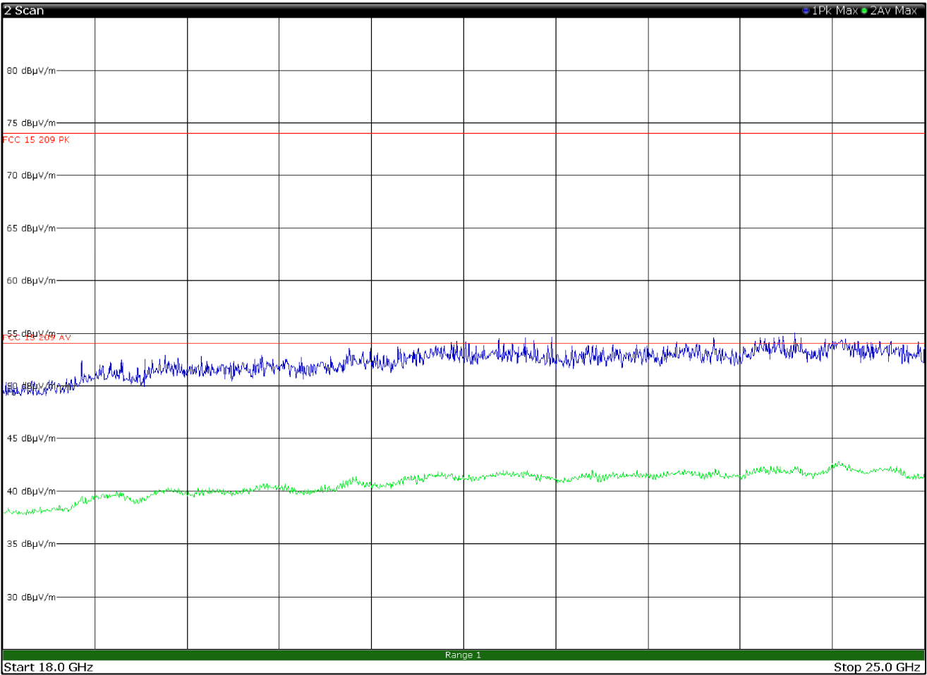
Radiated spurious emissions 18 to 25 GHz, TX 2480MHz,8DPSK MODULATION with antenna in vertical polarization
