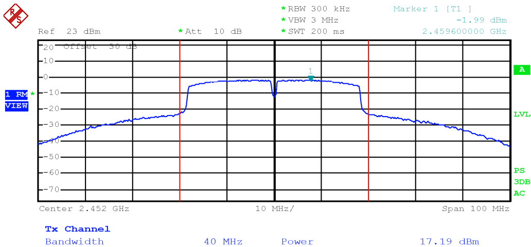
Output power TX 2452MHz, 802.11 nHT40 13.5 Mbps, multiple chain, chain 0
