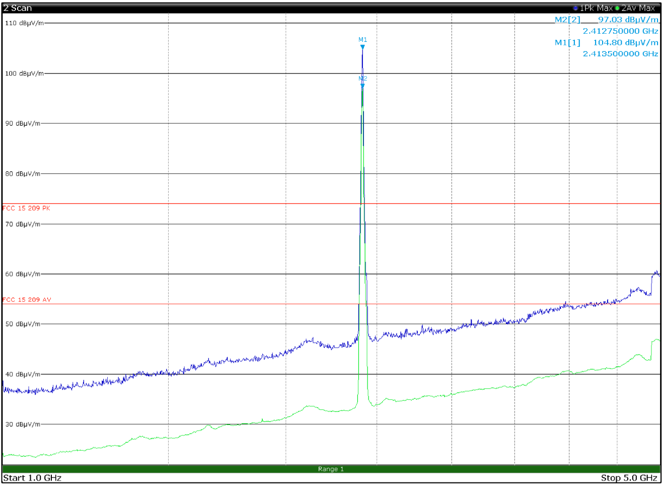
Radiated spurious emissions 1 to 5 GHz, TX 2412 MHz, CH01, 802.11n (20MHz), 6.5Mbps, multiple chain with antenna in vertical polarization
