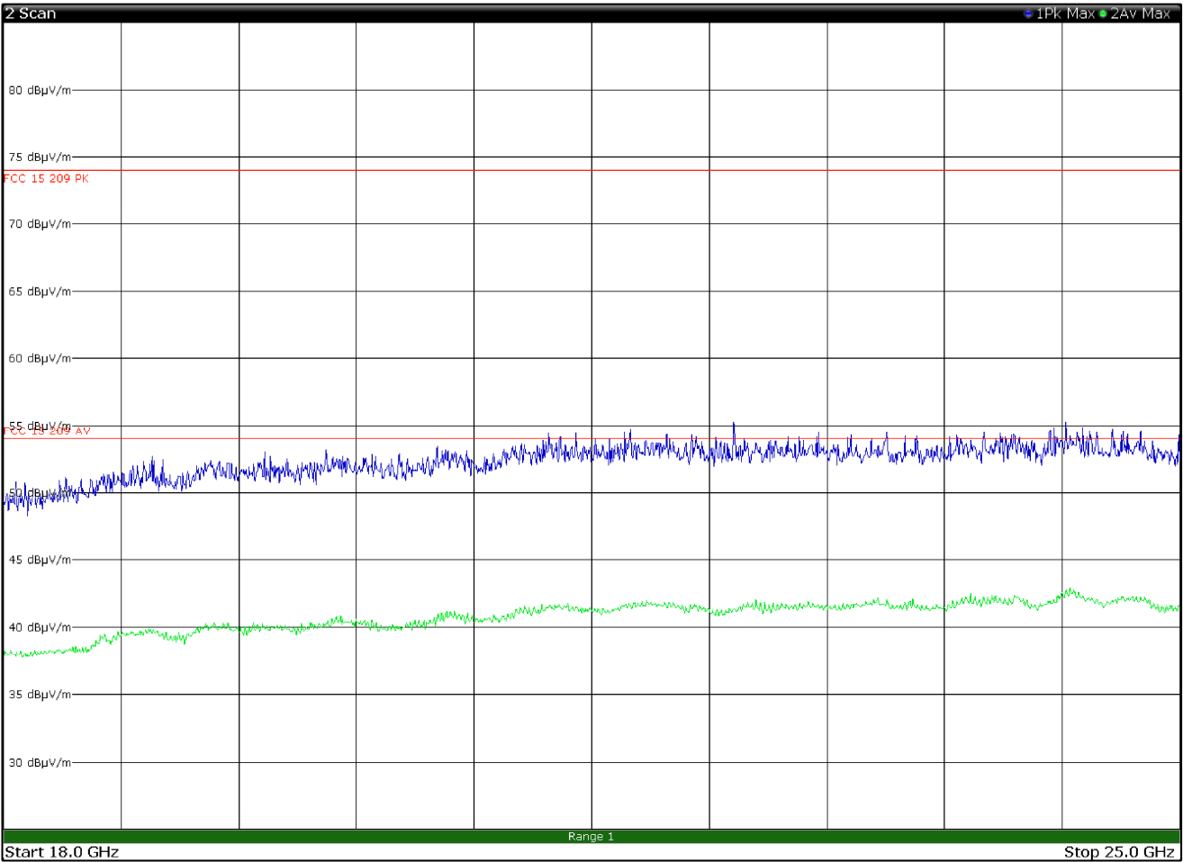
Radiated spurious emissions 18 to 25 GHz, TX 2480MHz,8DPSK MODULATION with antenna in horizontal polarization
