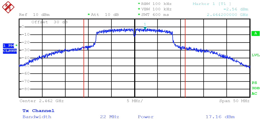
Output power TX 2462MHz, 802.11g, 6 Mbps, single chain
