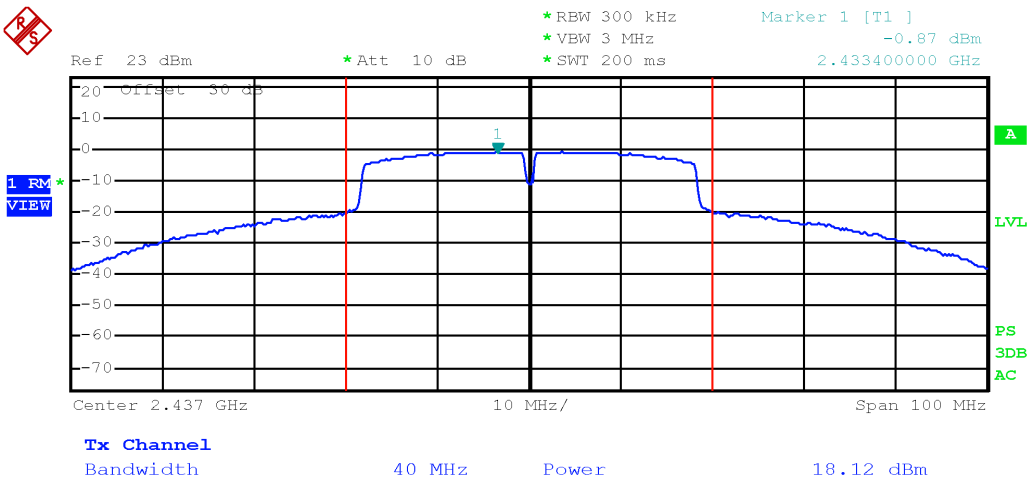
Output power TX 2437 MHz, 802.11 nHT40 13.5 Mbps, multiple chain, chain 1
