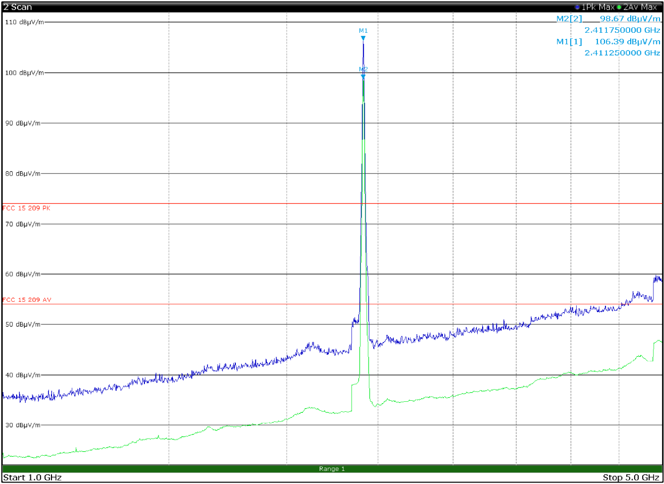
Radiated spurious emissions 1 to 5 GHz, TX 2412 MHz, CH01, 802.11n (20MHz), 6.5Mbps, multiple chain with antenna in horizontal polarization
