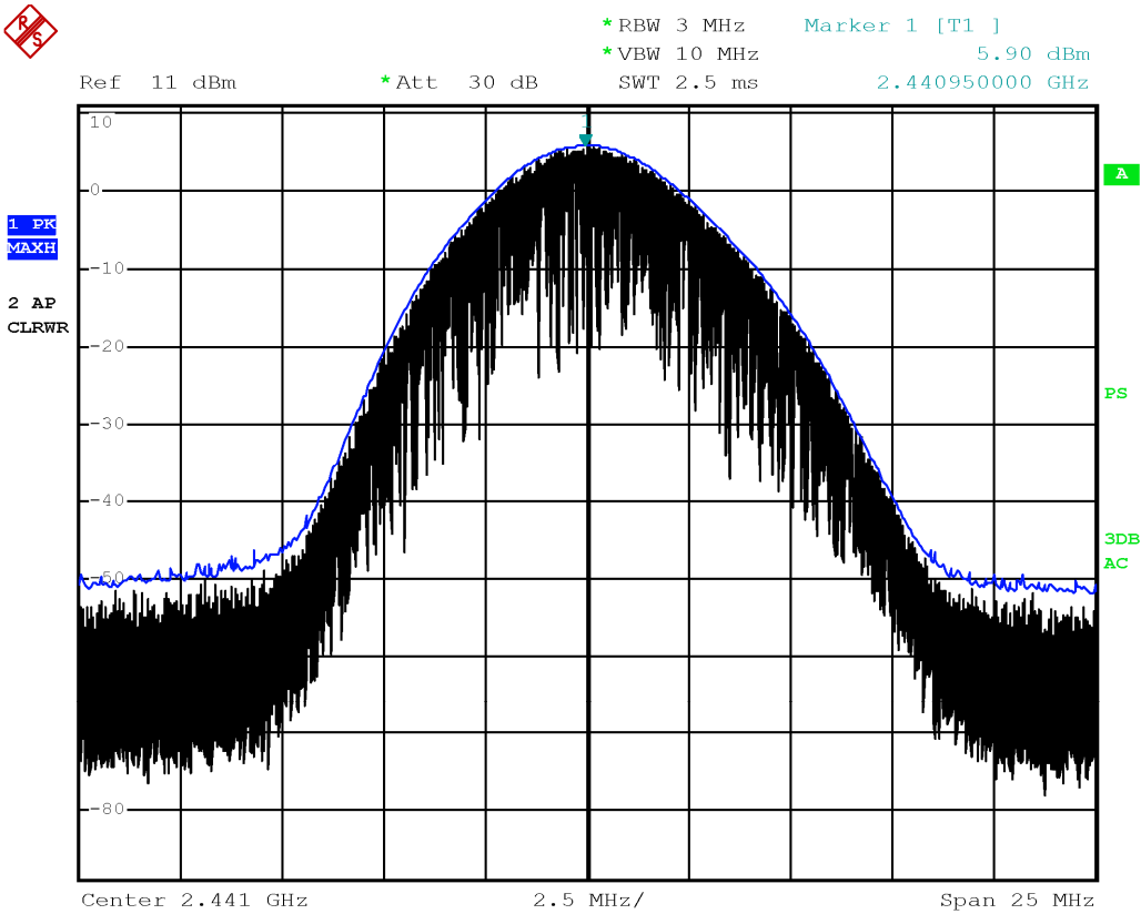
Output power TX 2441MHz, BT 8DPSK
