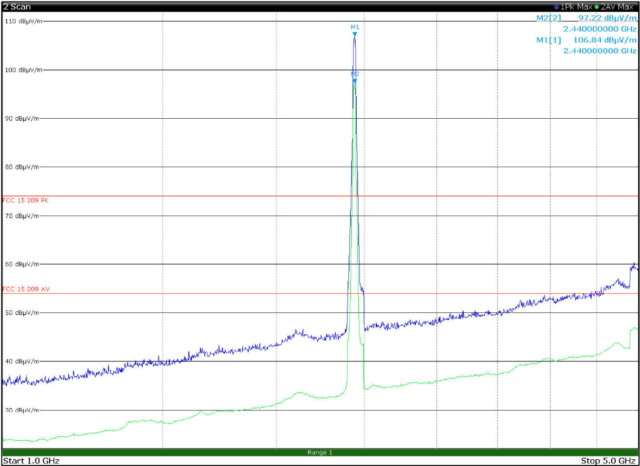
Radiated spurious emissions 1 to 5 GHz, TX 2437 MHz, CH06, 802.11g, 6Mbps, multiple chain with antenna in vertical polarization
