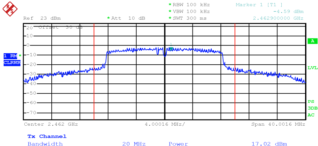
Output power TX 2462 MHz, 802.11g, 6 Mbps, multiple chain, chain 0
