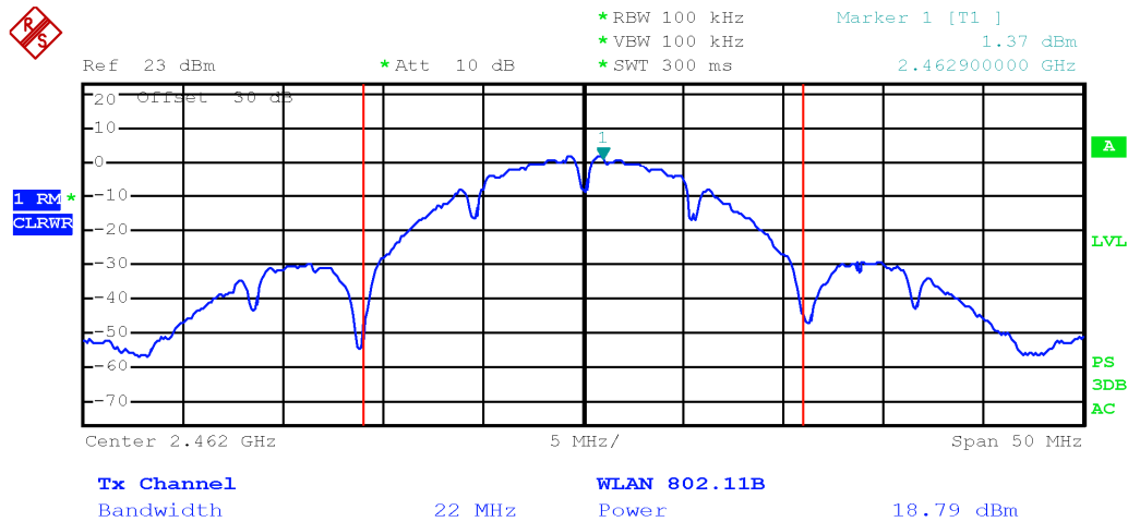
Output power TX 2462 MHz, 802.11b, 1 Mbps, multiple chain, chain 1
