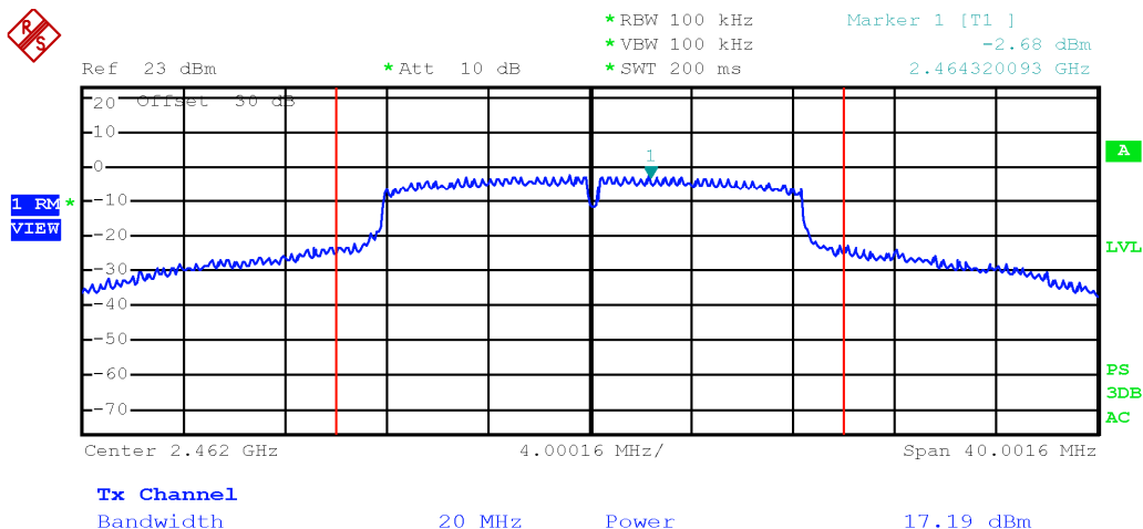
Output power TX 2462 MHz, 802.11 nHT20 6.5 Mbps, multiple chain, chain 0
