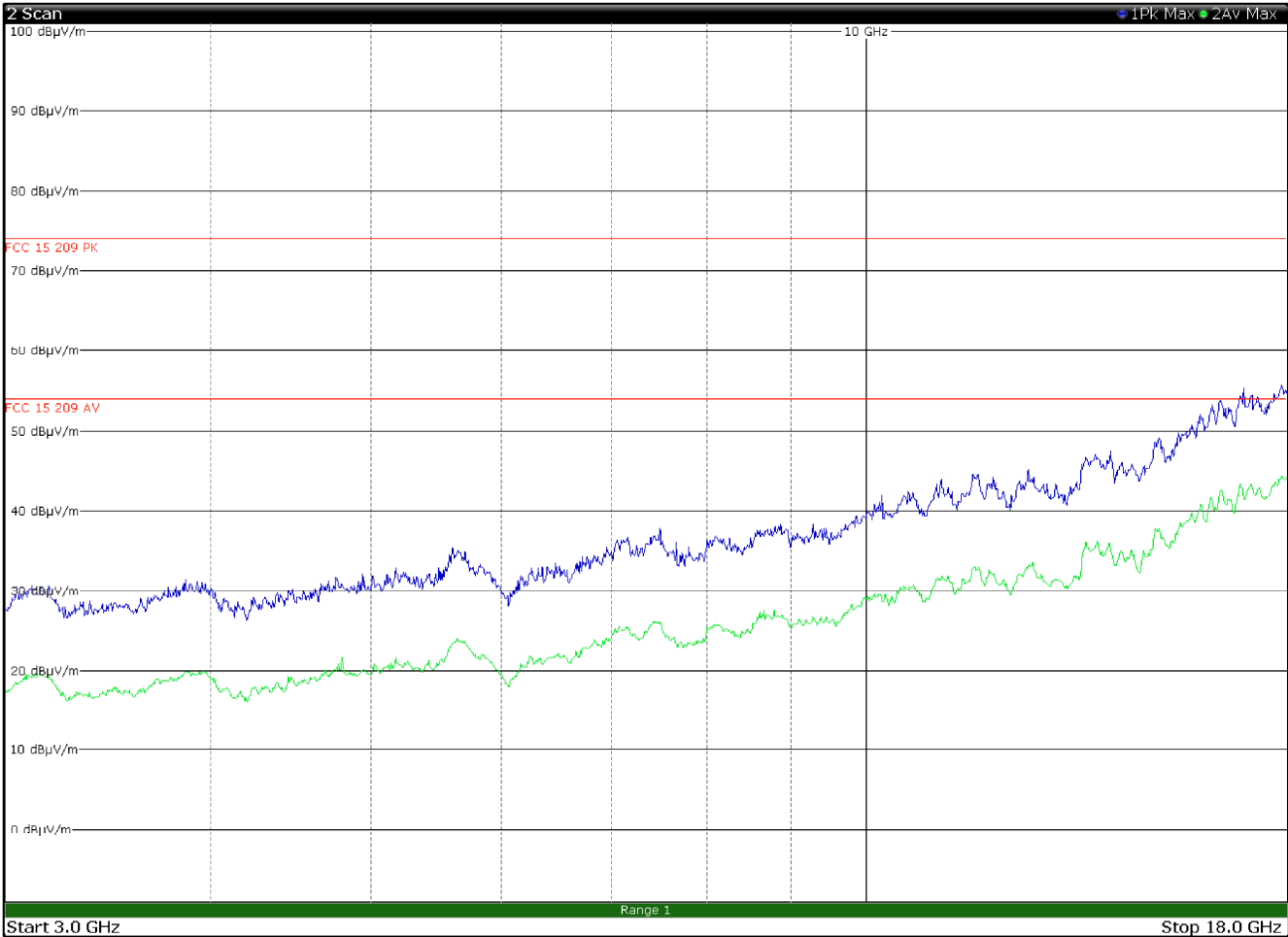
Radiated spurious emissions 3 to 18GHz, TX 2441 MHz, CH 00, 8DPSK MODULATION with antenna in horizontal polarization
