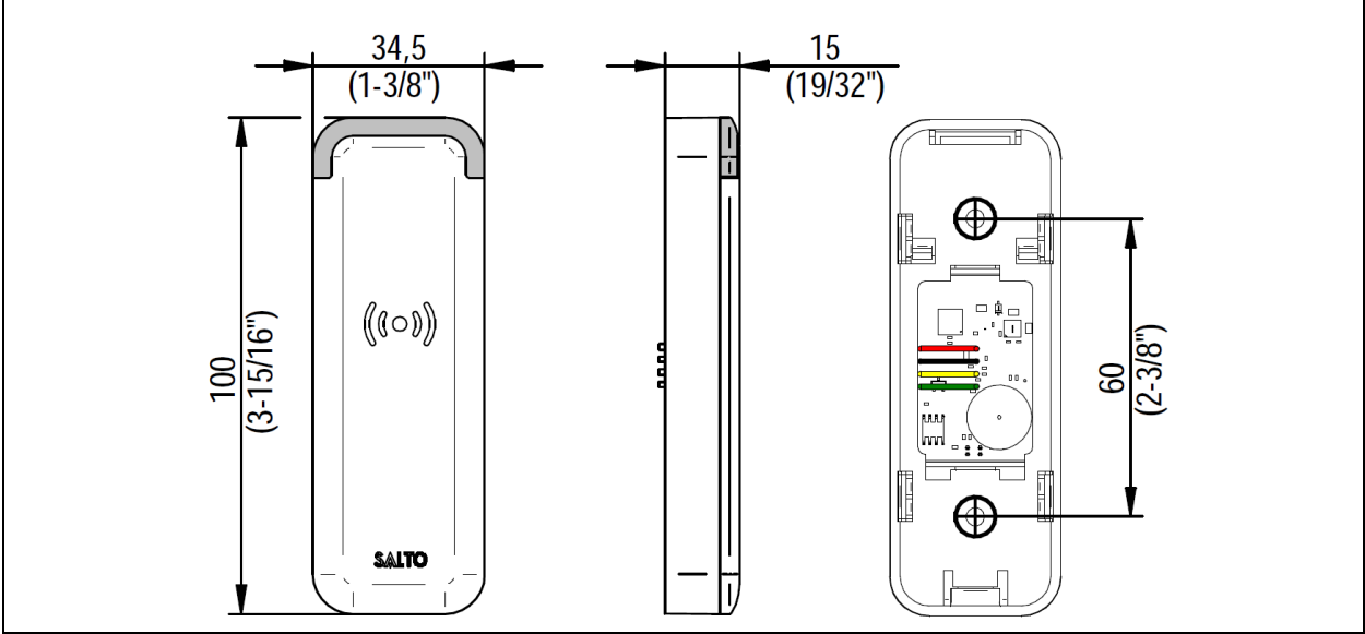
Photo 6: Dimensions
