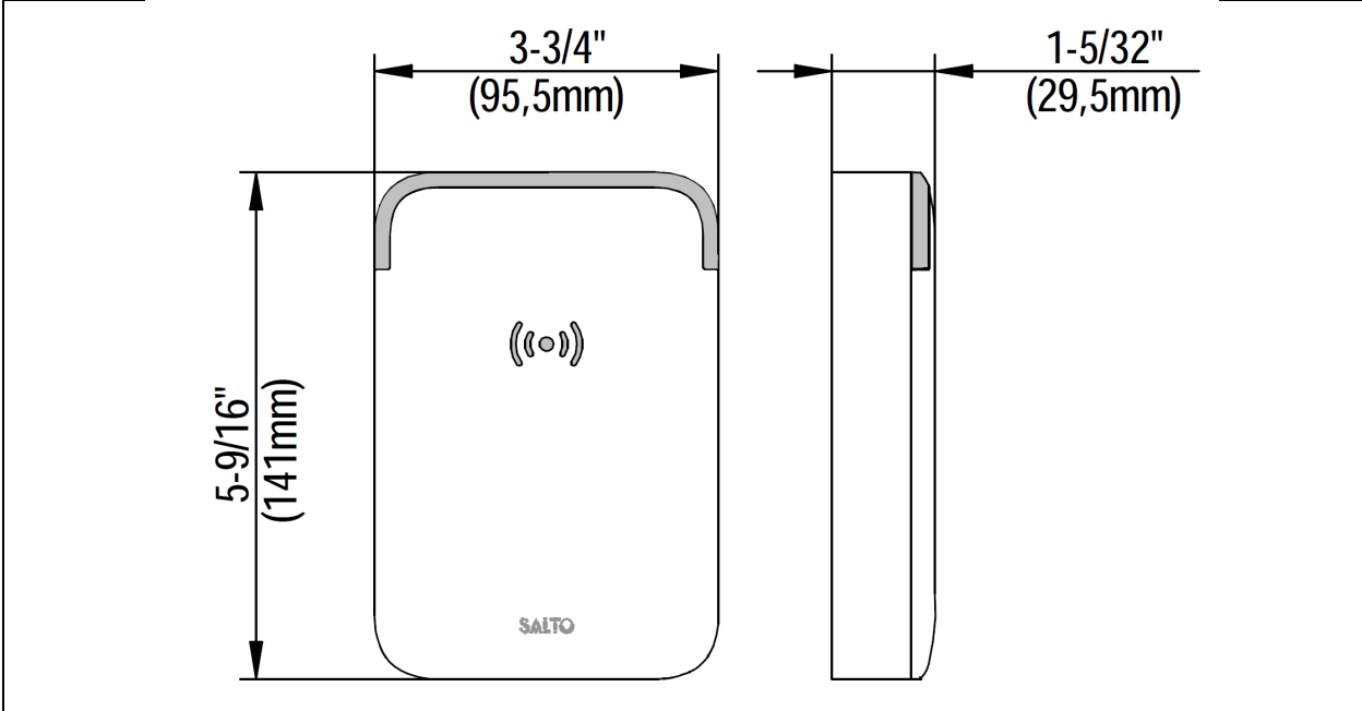
Photo 4: Dimensions.
