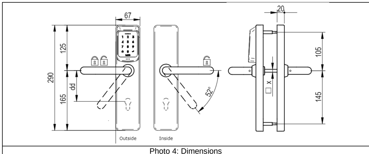
Photo 4: Dimensions
