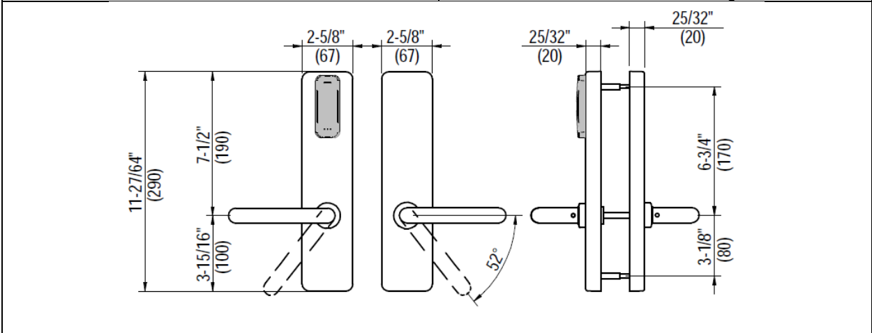
Photo 5: Dimensions
