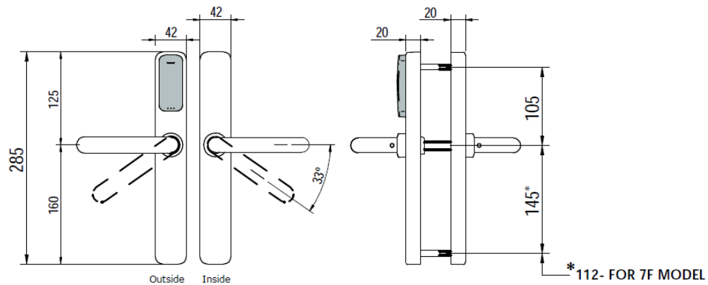
Photo 5: Dimensions
