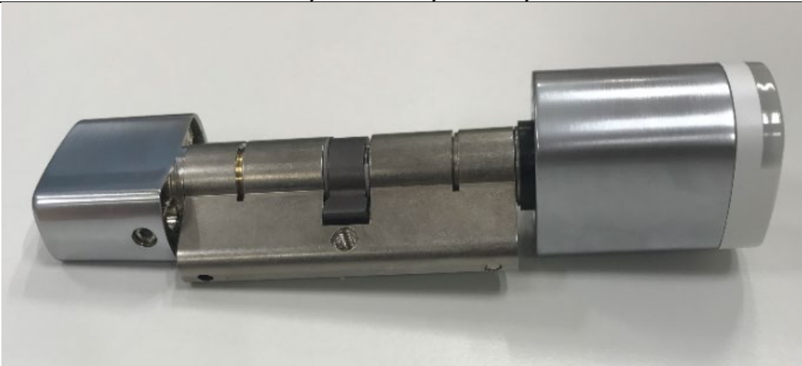
Photo 3: Side view of the cylinder knob, cylinder body and interior thumbturn.
