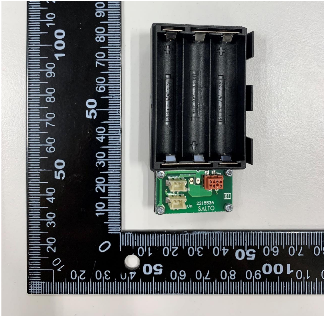
Top view
