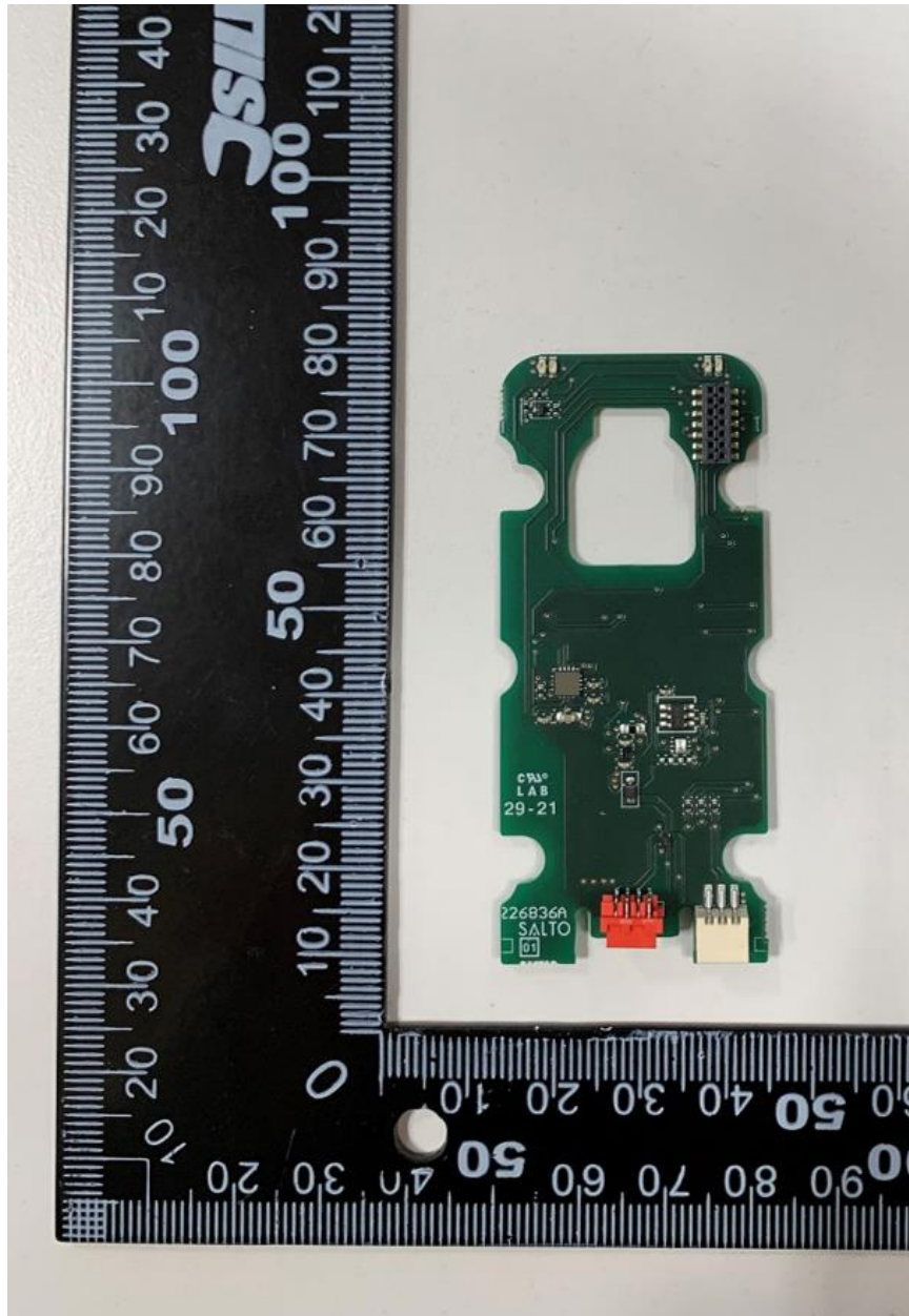
Top View
