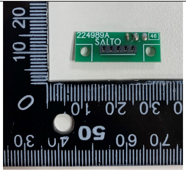
Photo 11: Bottom view
