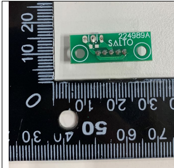
Photo 10: Top view
