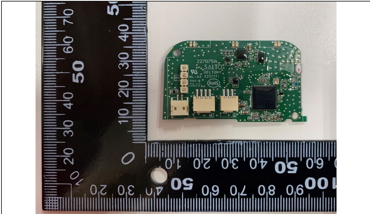
Photo 1: Top view
