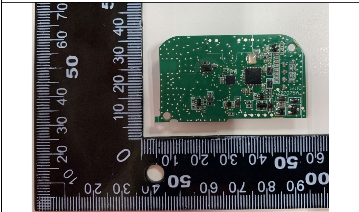
Photo 2: Bottom view
