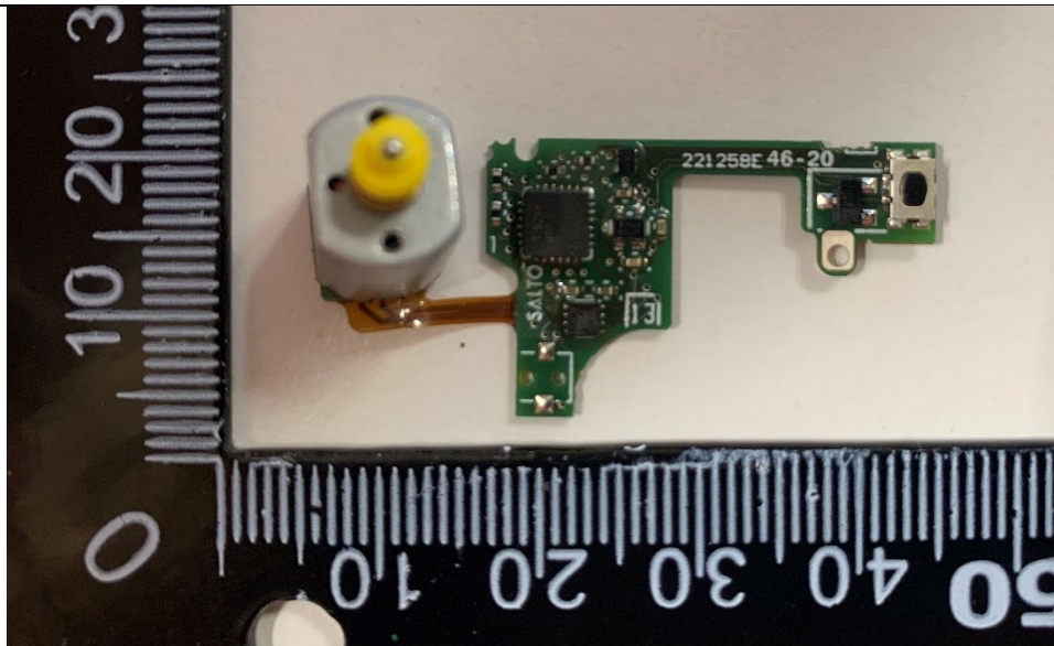
Photo 6: Motor circuit top view
