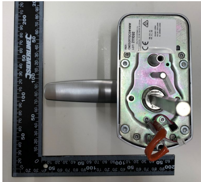
Photo 6: Outdoor back view
