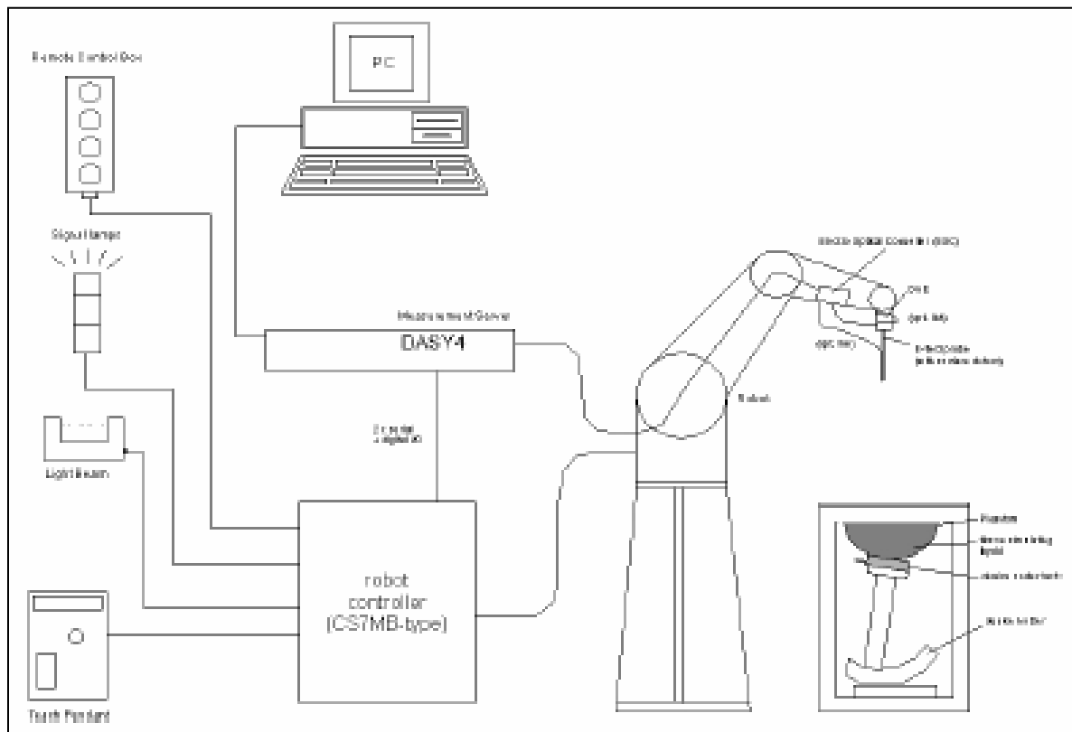
Figure 1: Measurement System diagram
