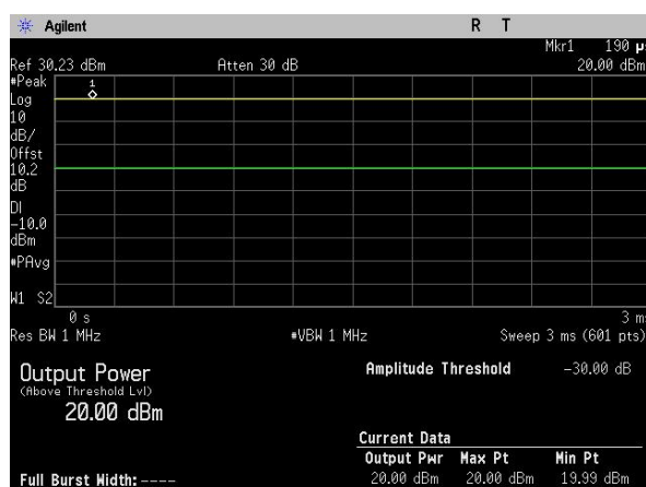
CW Signal-20dBm Peak power
