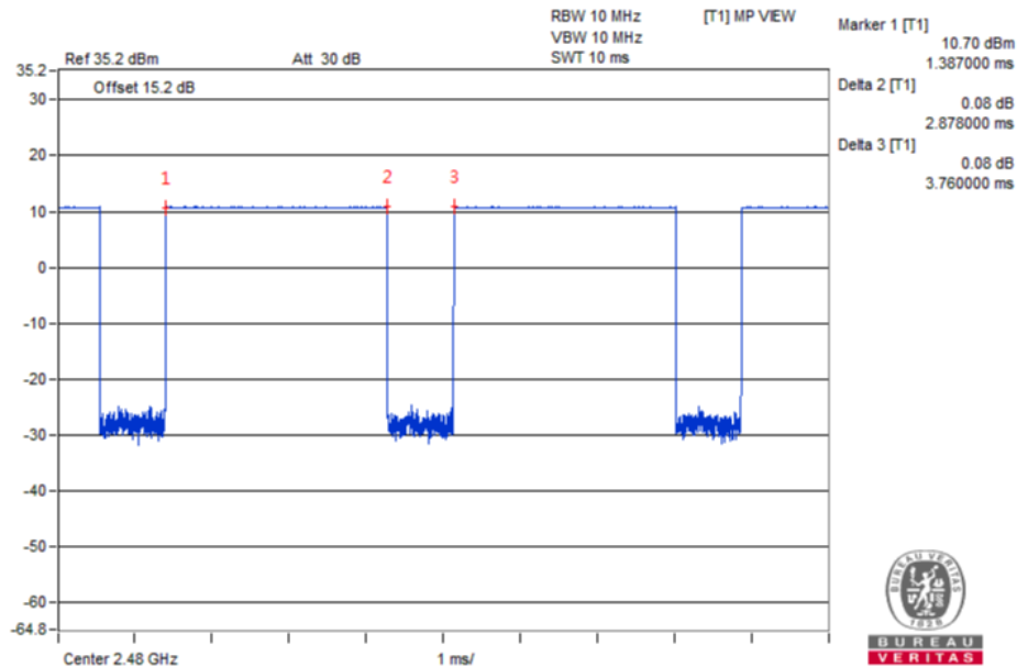
Time-domain plot for Bluetooth transmission signal
