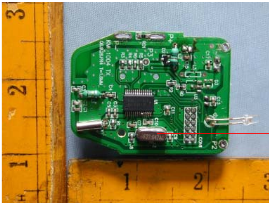
Full View of Component Side
