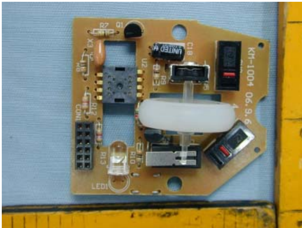
Component Side of Button
