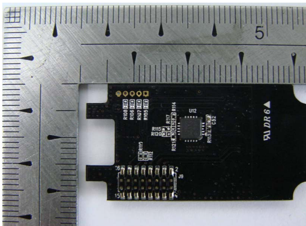
BLUETOOTH BOARD (BOTTOM)
