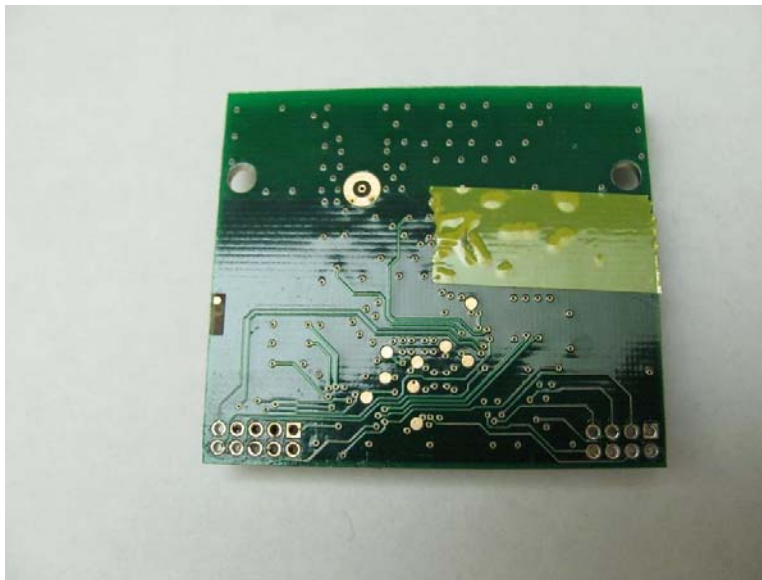
Figure 4- Mica/PCB Rear
