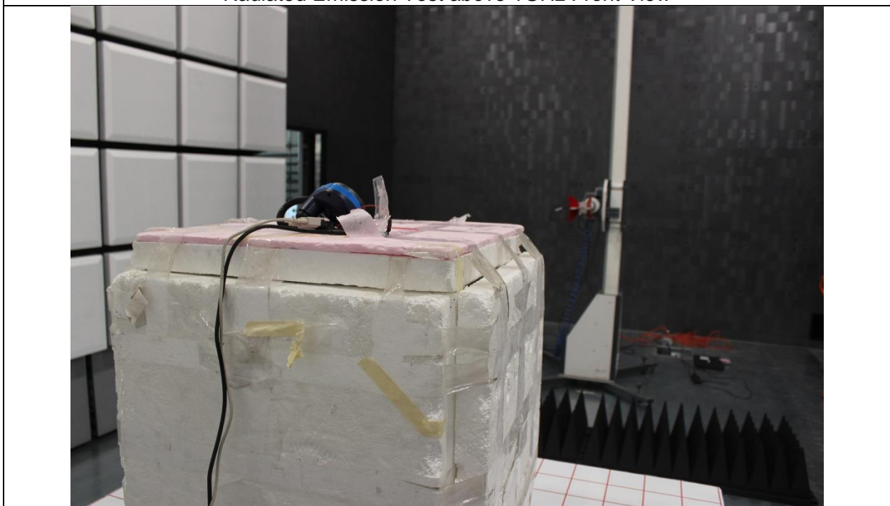
Radiated Emission Test above 1GHz Rear View
