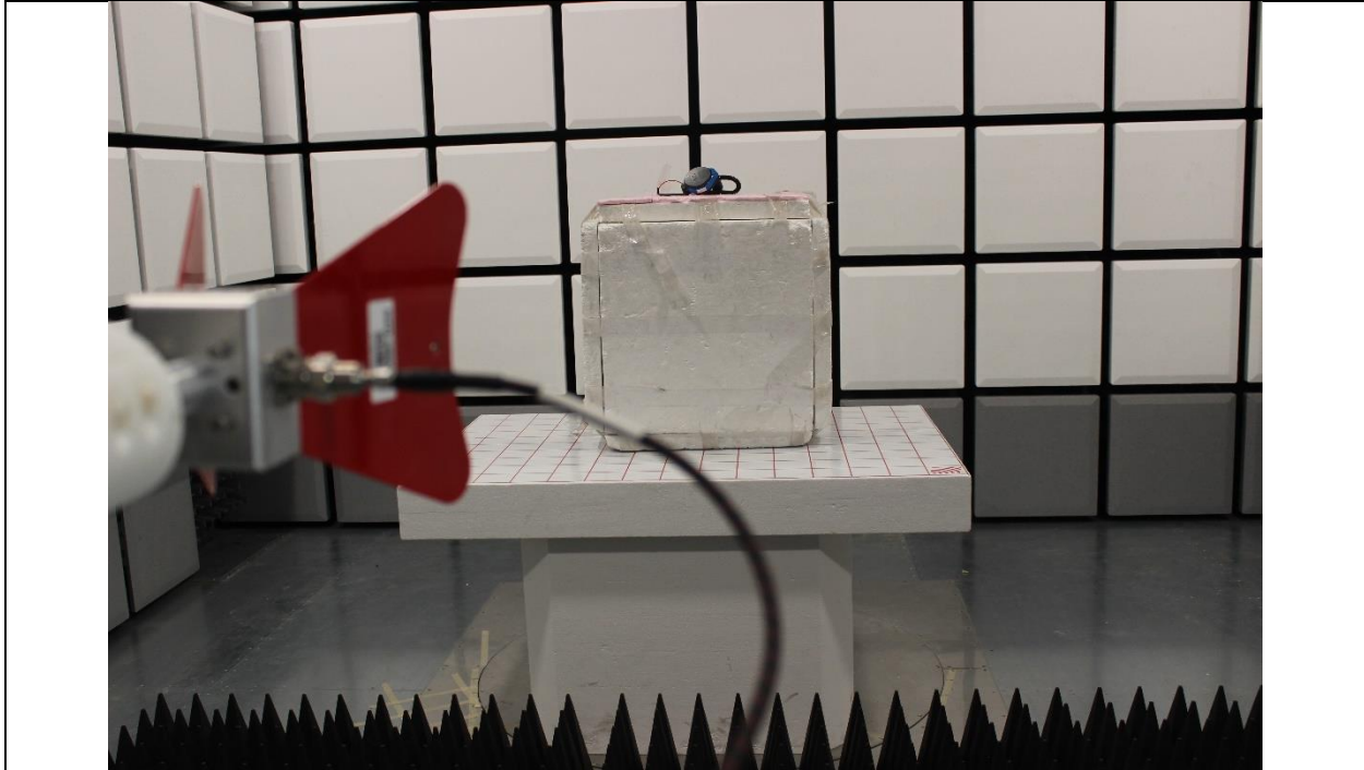
Radiated Emission Test above 1GHz Front View
