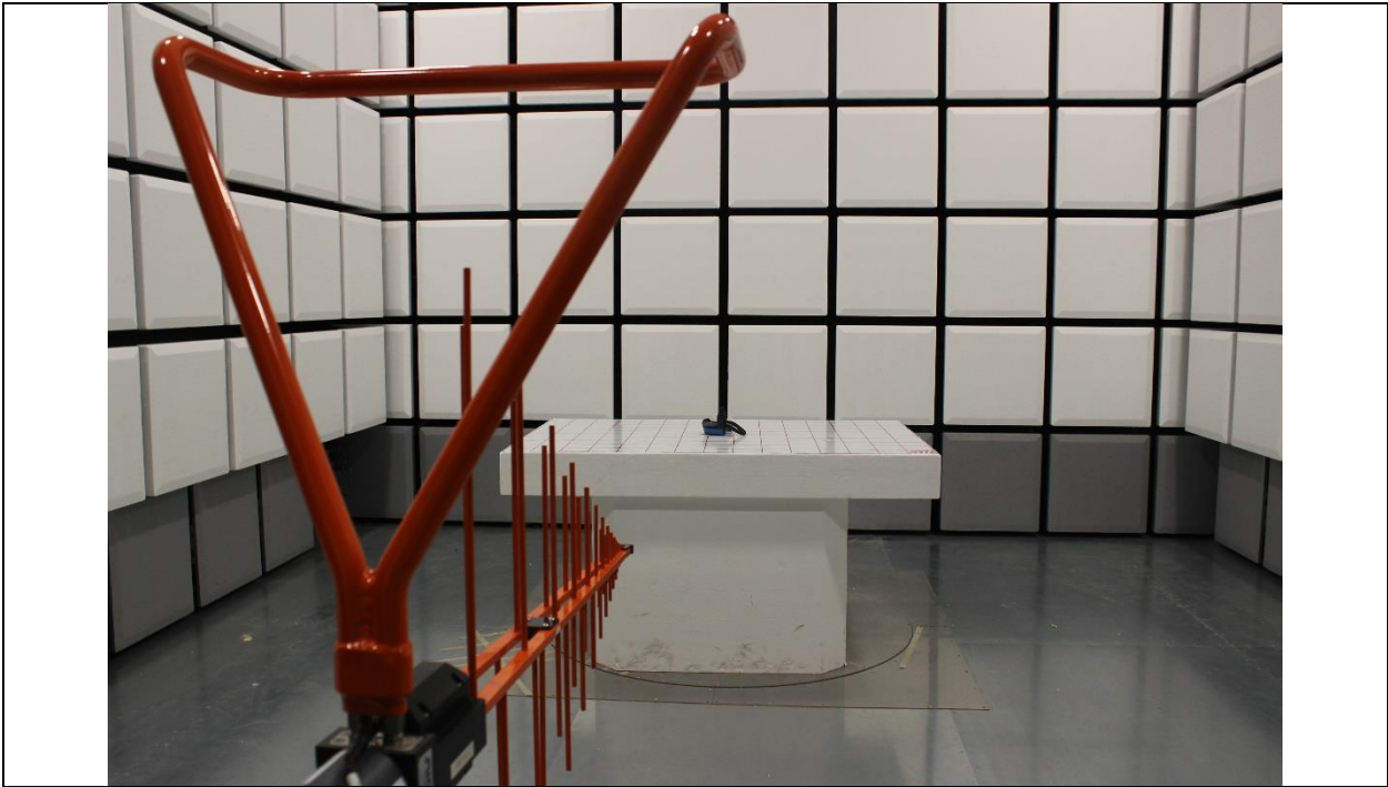
Radiated Emission Test below 1GHz Front View
