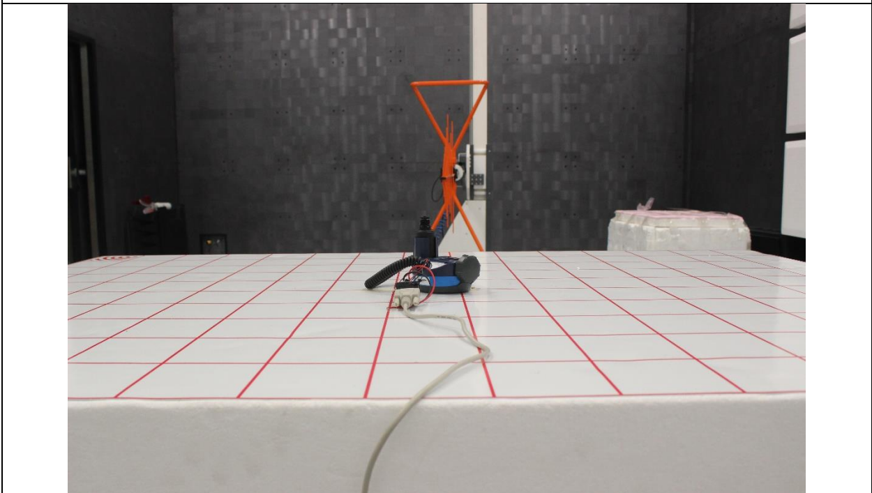
Radiated Emission Test below 1GHz Rear View
