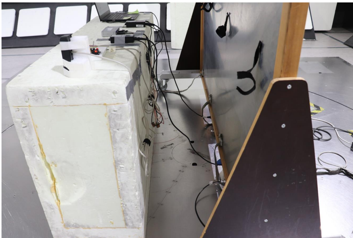
Photograph 5. Conducted Emission
