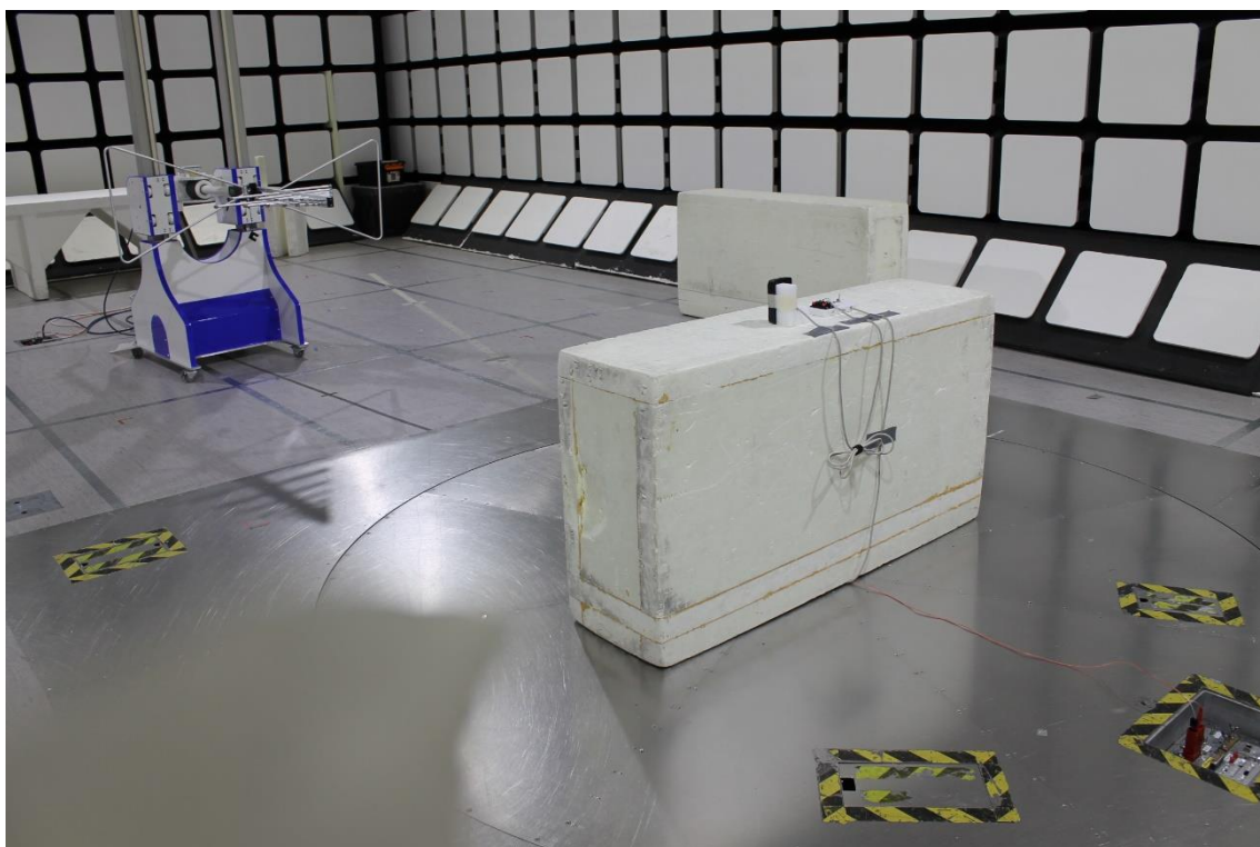
Photograph 4. Radiated Emissions 30 – 1000 MHz
