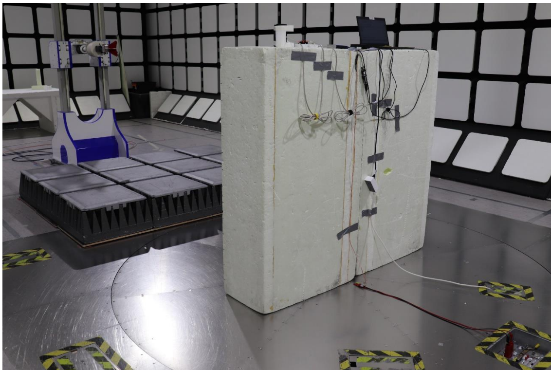
Photograph 4. Radiated Emissions 1 – 18 GHz
