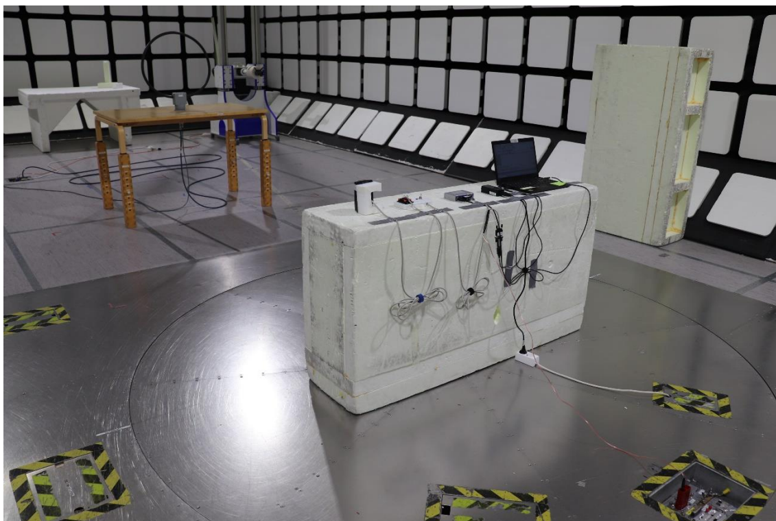
Photograph 3. Radiated Emissions 9 kHz – 30 MHz
