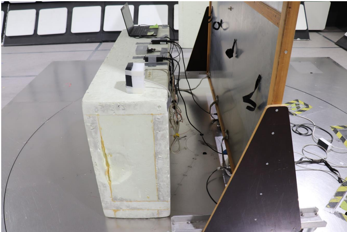
Photograph 5. Conducted Emission
