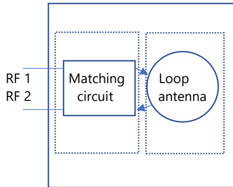
Picture 1. Matching circuit and Loop Antenna
