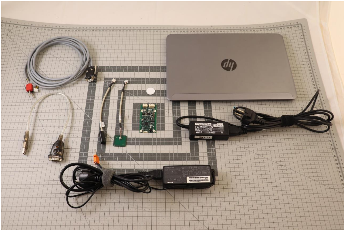
Photograph 1. The EUT and peripherals
