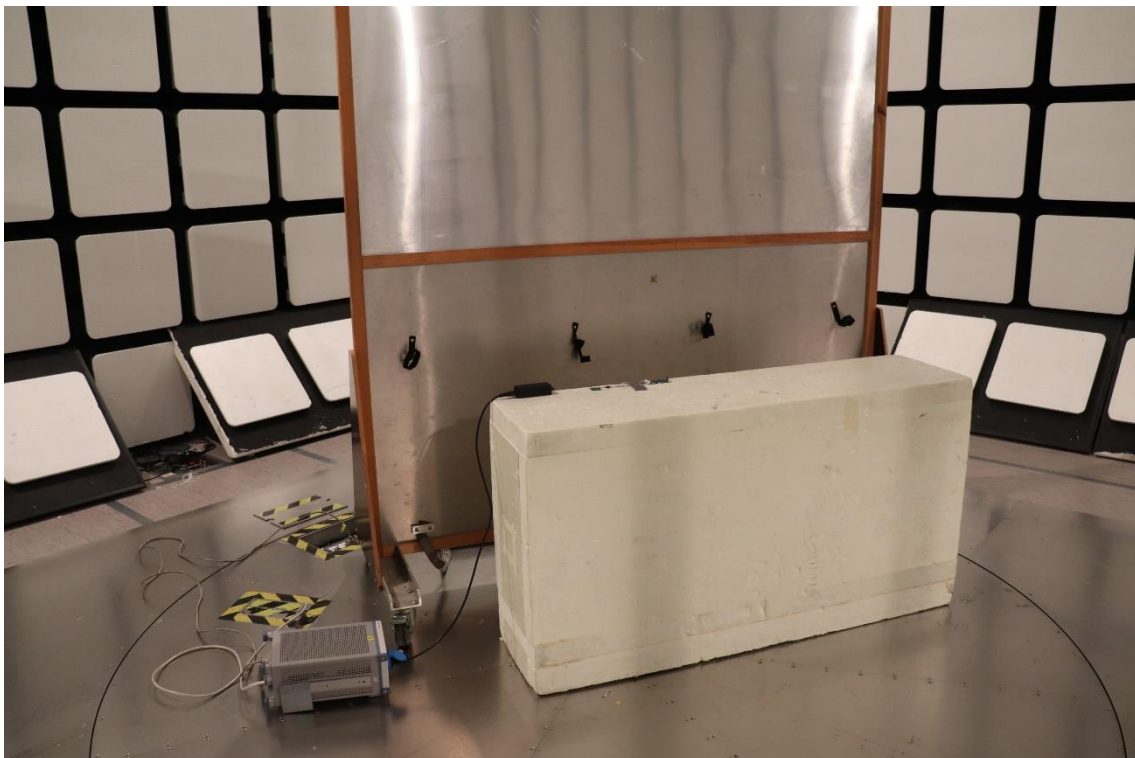
Photograph 7. Conducted Emission
