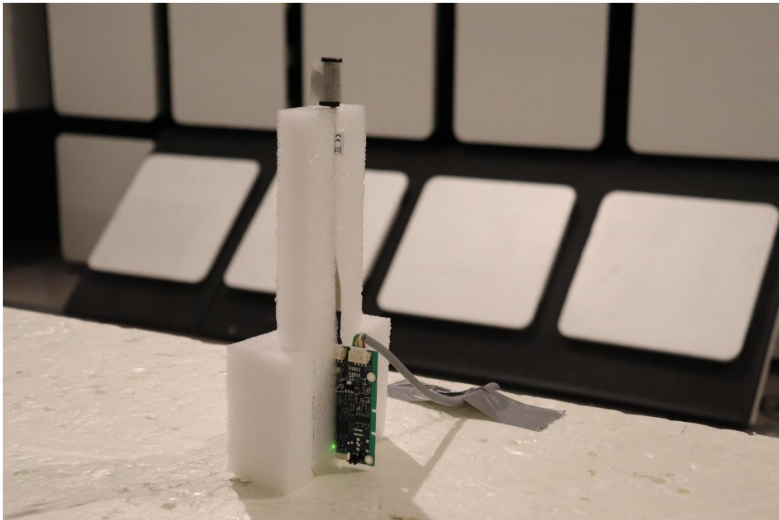
Photograph 4. The EUT positioning during Radiated Emissions, Cylinder Antenna
