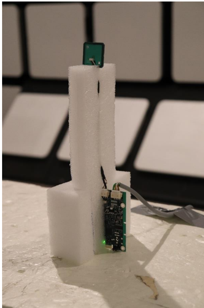
Photograph 3. The EUT positioning during Radiated Emissions, PCB Antenna
