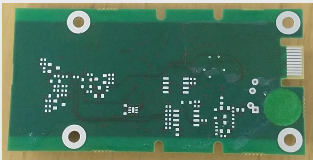
Picture 2. 9CD 3.0 PCB Bottom
