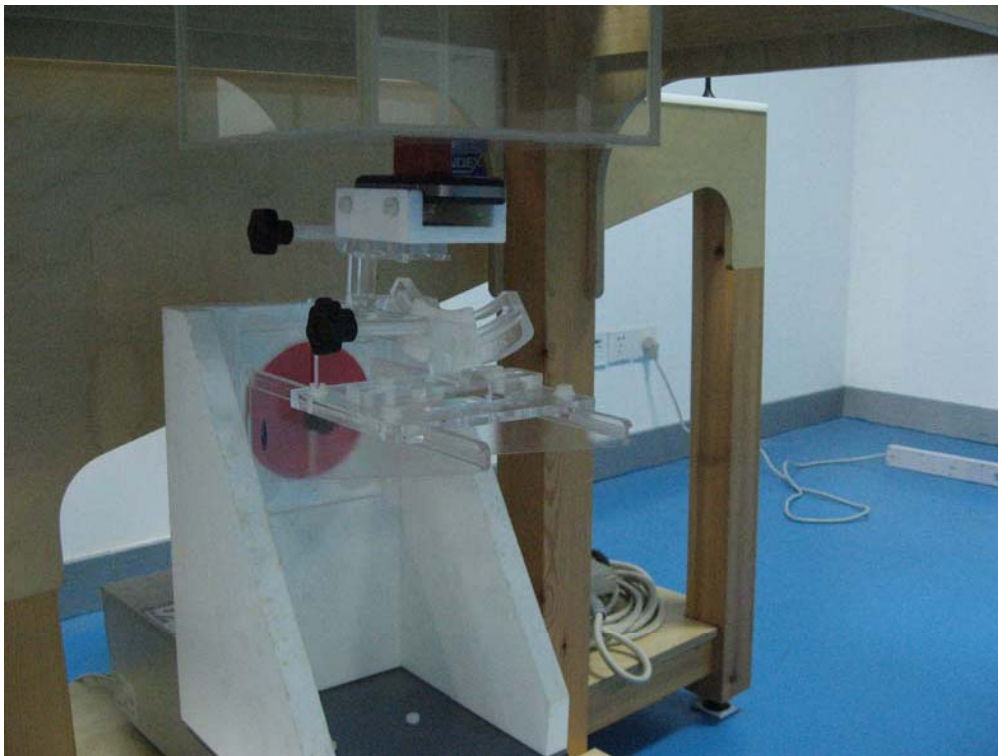
Fig.8 Side Position(1.5cm distance between the phantom and back of the phone)
