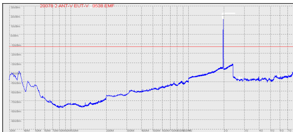
(Plot F.2: CDMA 1900MHz Channel = 9538, Test Antenna Vertical)
