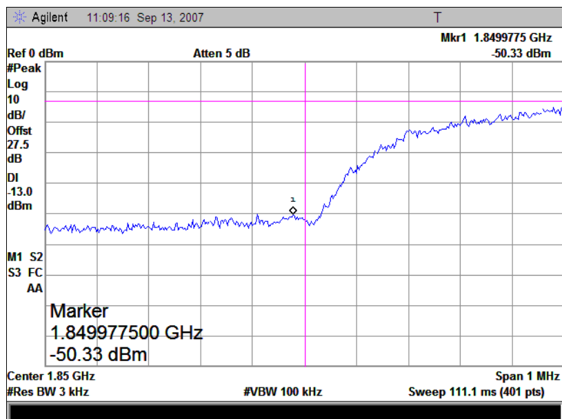
(Plot C: Channel = 9262)
