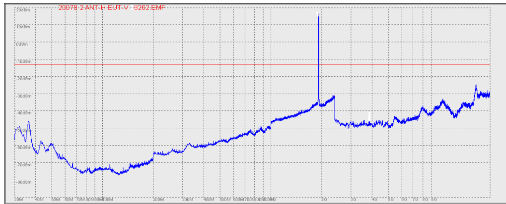
(Plot D.1: CDMA 1900MHz Channel = 9262, Test Antenna Horizontal)
