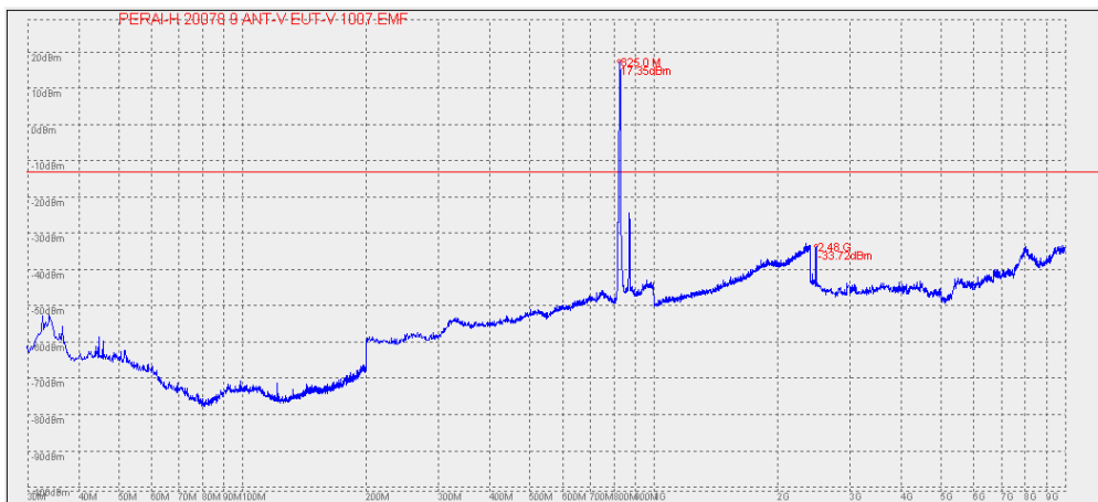
(Plot A.2: CDMA 850MHz Channel = 4132, Test Antenna Vertical)
