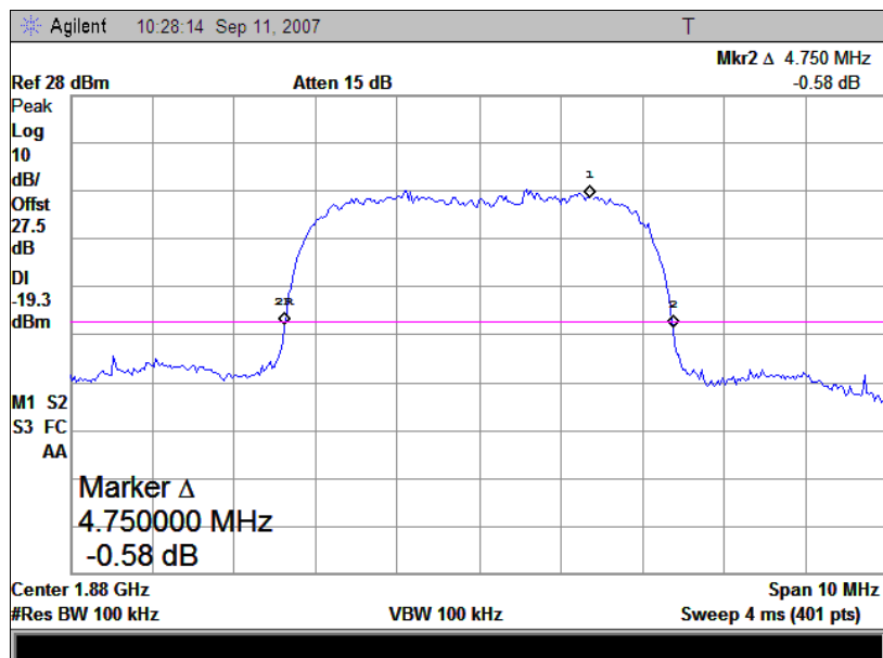
(Plot B: WCDMA 1900MHz Channel = 9400)
