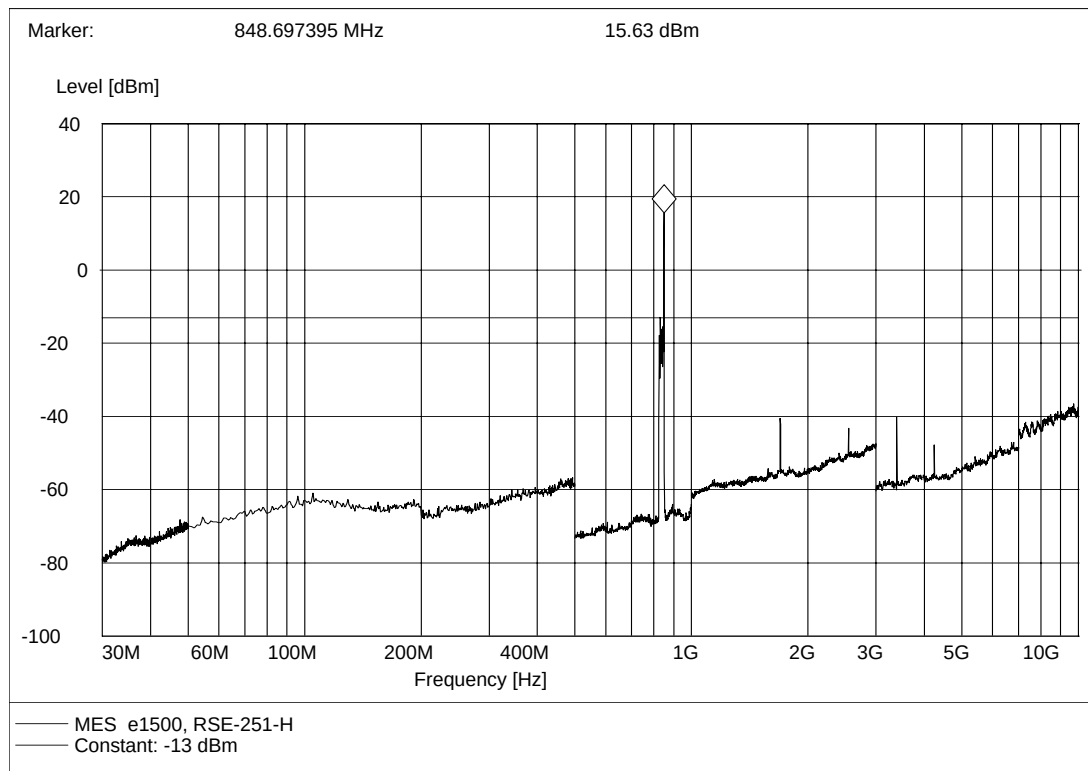
(Plot C.1: GSM 850MHz Channel = 251, Test Antenna Horizontal)
