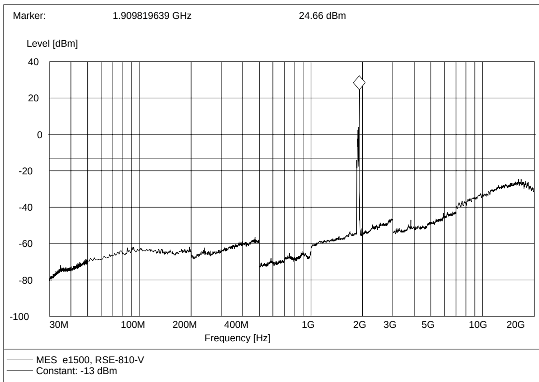
(Plot F.2: GSM 1900MHz Channel = 810, Test Antenna Vertical)
