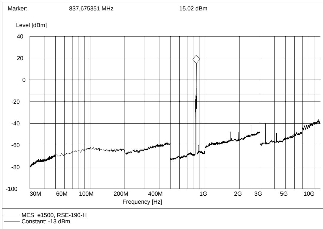
(Plot B.1: GSM 850MHz Channel = 190, Test Antenna Horizontal)
