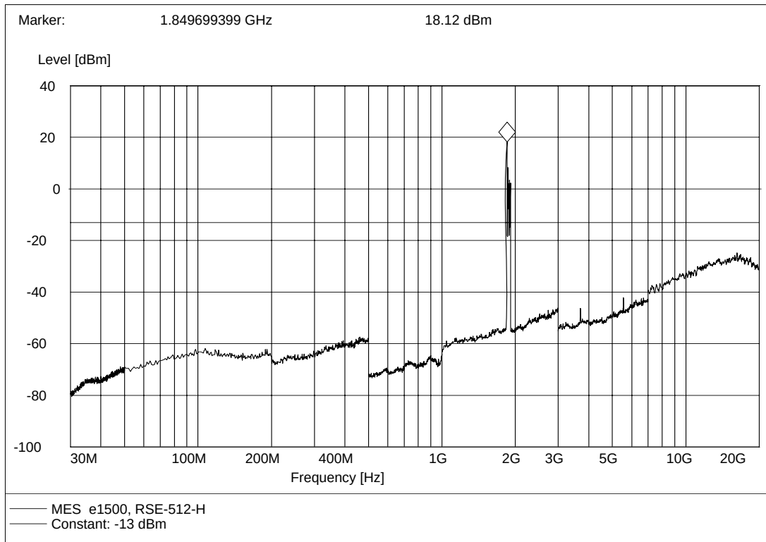
(Plot D.1: GSM 1900MHz Channel = 512, Test Antenna Horizontal)
