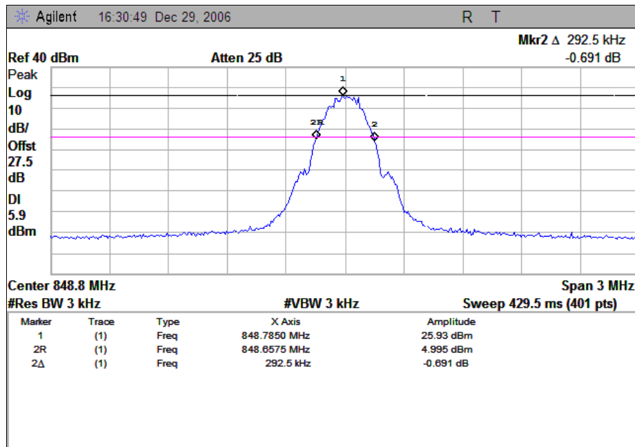
(Plot C: GSM 850MHz Channel = 251)
