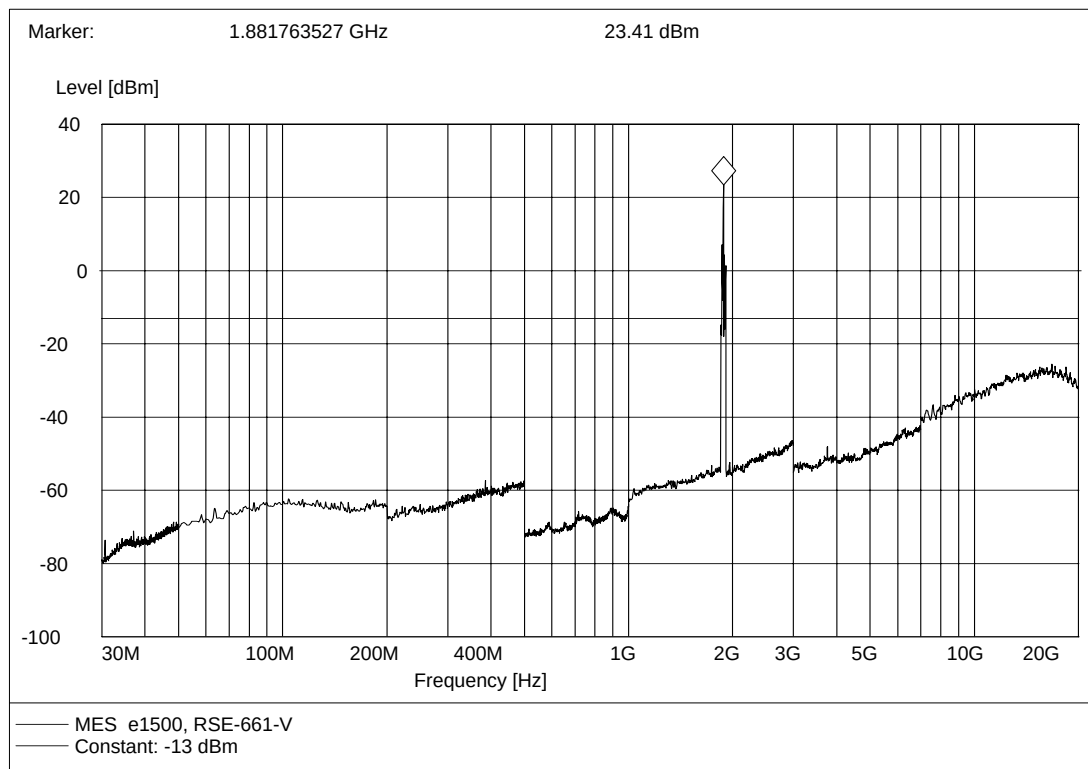
(Plot E.2: GSM 1900MHz Channel = 661, Test Antenna Vertical)
