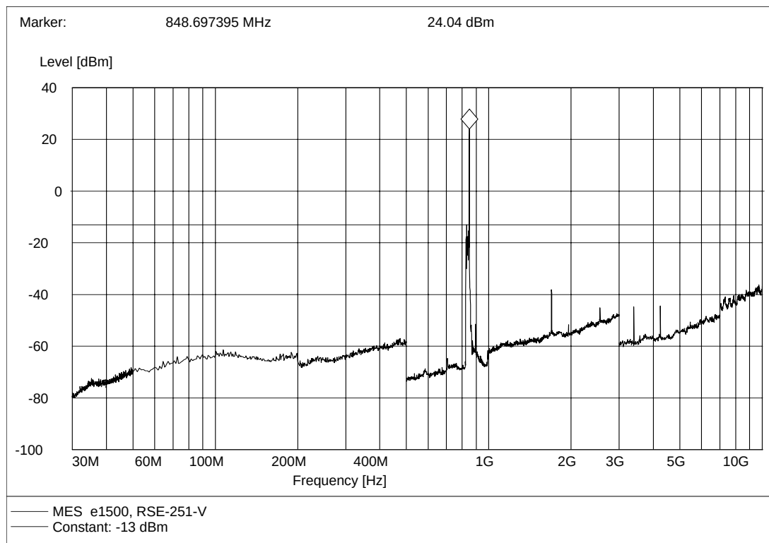
(Plot C.2: GSM 850MHz Channel = 251, Test Antenna Vertical)
