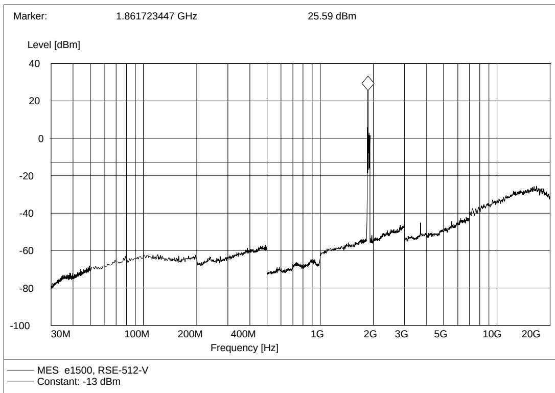
(Plot D.2: GSM 1900MHz Channel = 512, Test Antenna Vertical)
