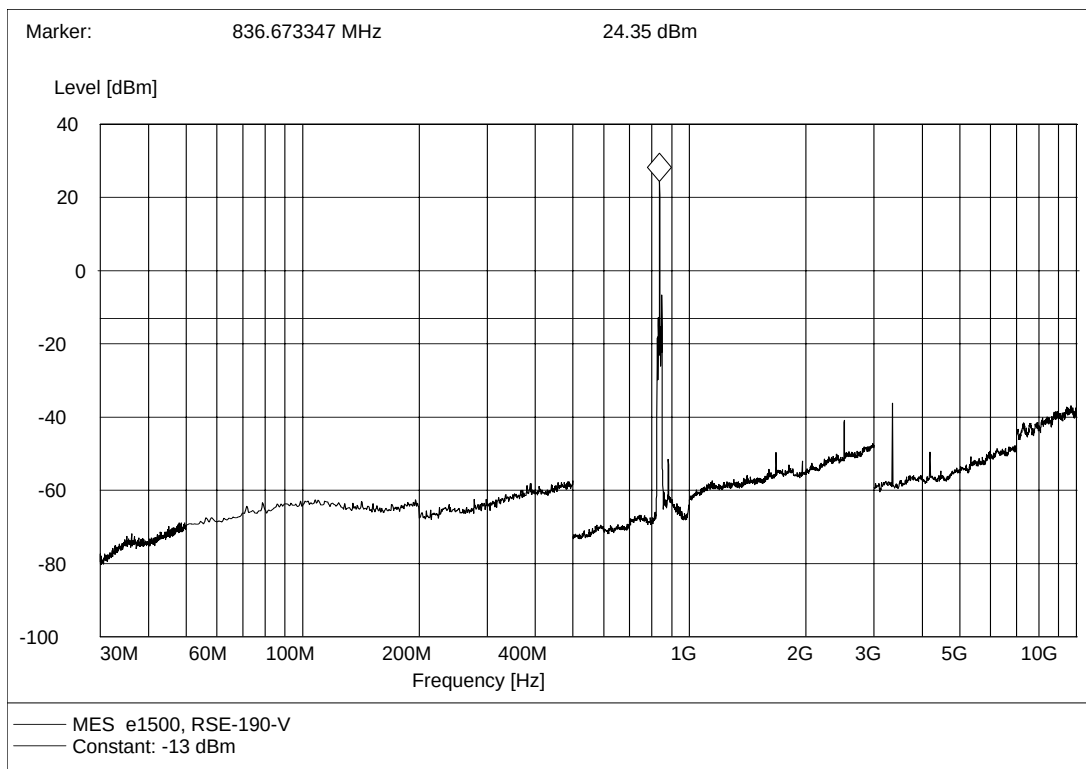
(Plot B.2: GSM 850MHz Channel = 190, Test Antenna Vertical)
