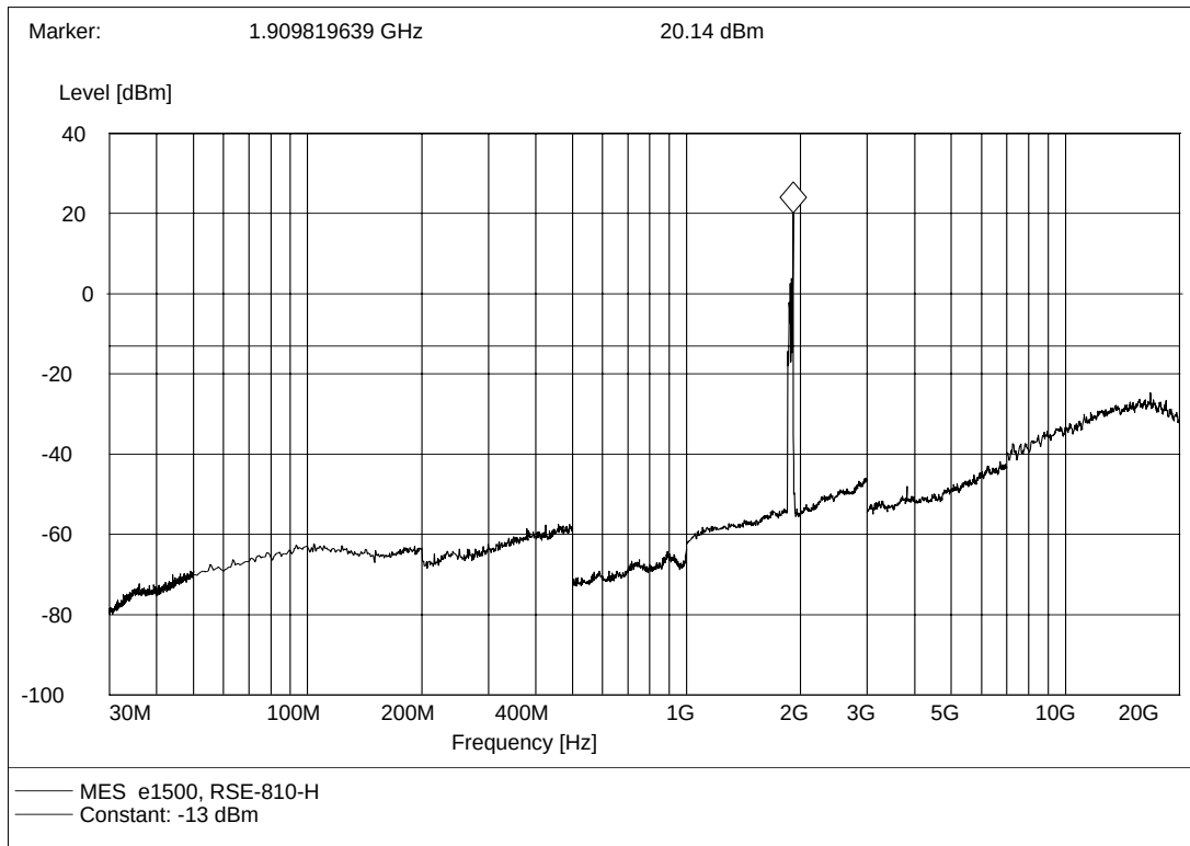
(Plot F.1: GSM 1900MHz Channel = 810, Test Antenna Horizontal)
