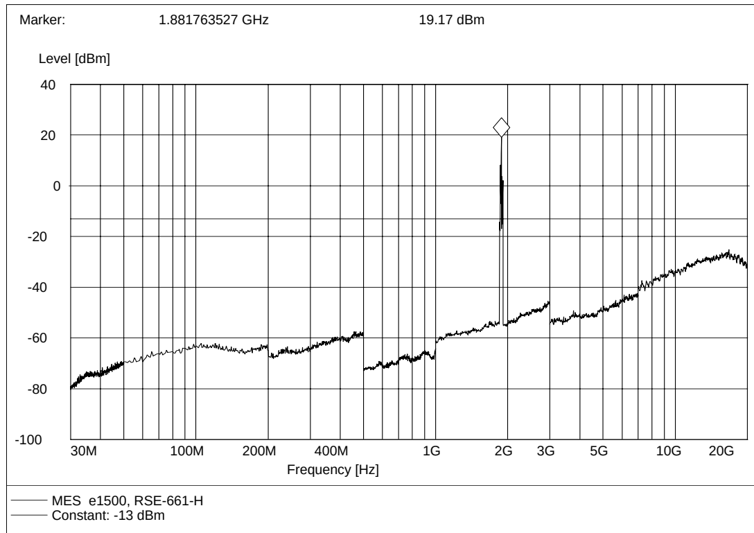
(Plot E.1: GSM 1900MHz Channel = 661, Test Antenna Horizontal)
