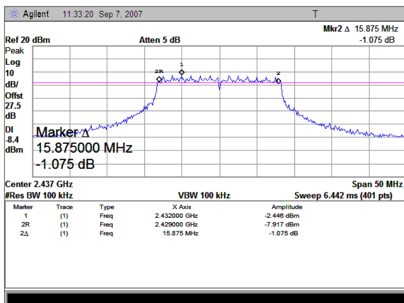
(Plot E: Channel = 2437)
