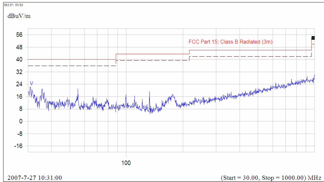
(Plot A.6: Antenna Vertical, 30MHz to 1GHz)
