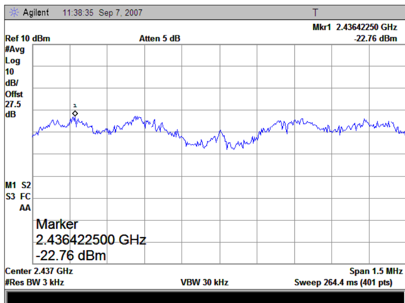
(Plot E: Channel = 6)
