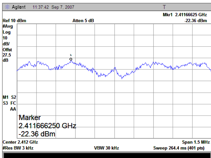
(Plot D: Channel = 1)
