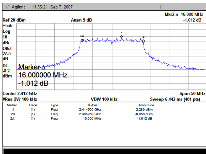
(Plot D: Channel = 2412)
