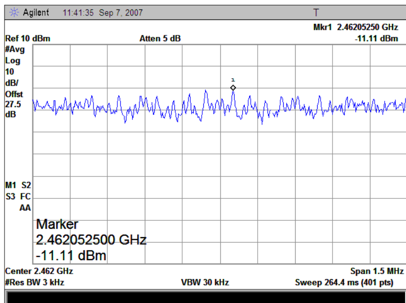
(Plot C: Channel = 11)
