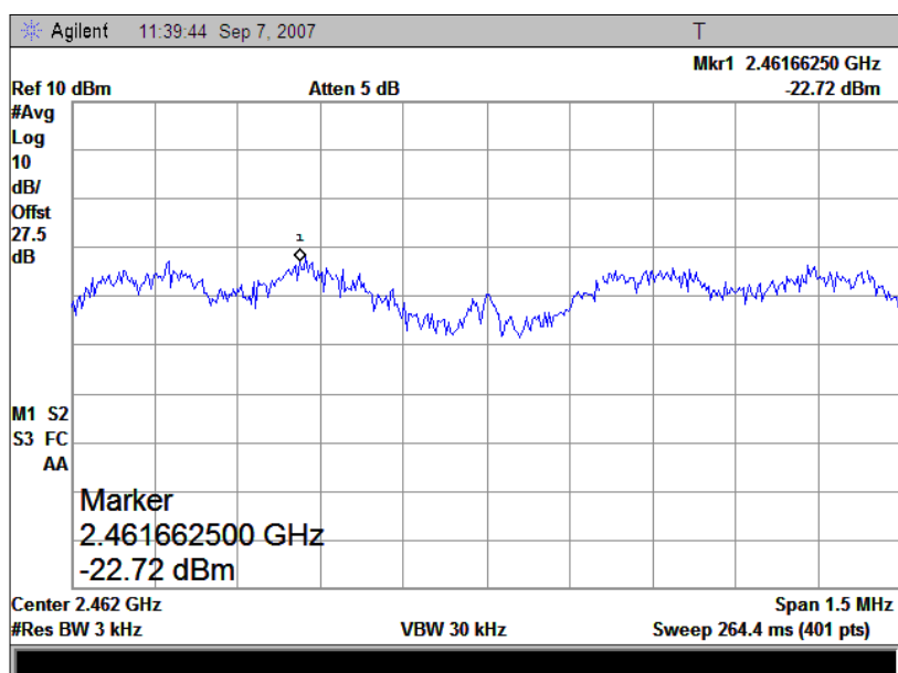
(Plot F: Channel = 11)
