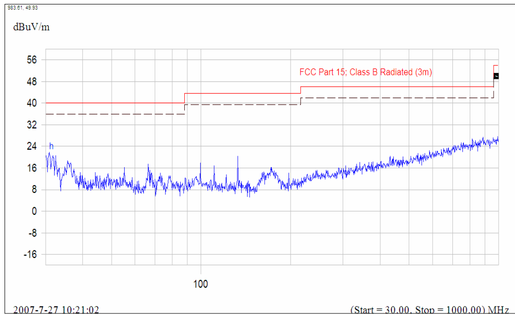
(Plot A.2: Antenna Horizontal, 30MHz to 1GHz)
