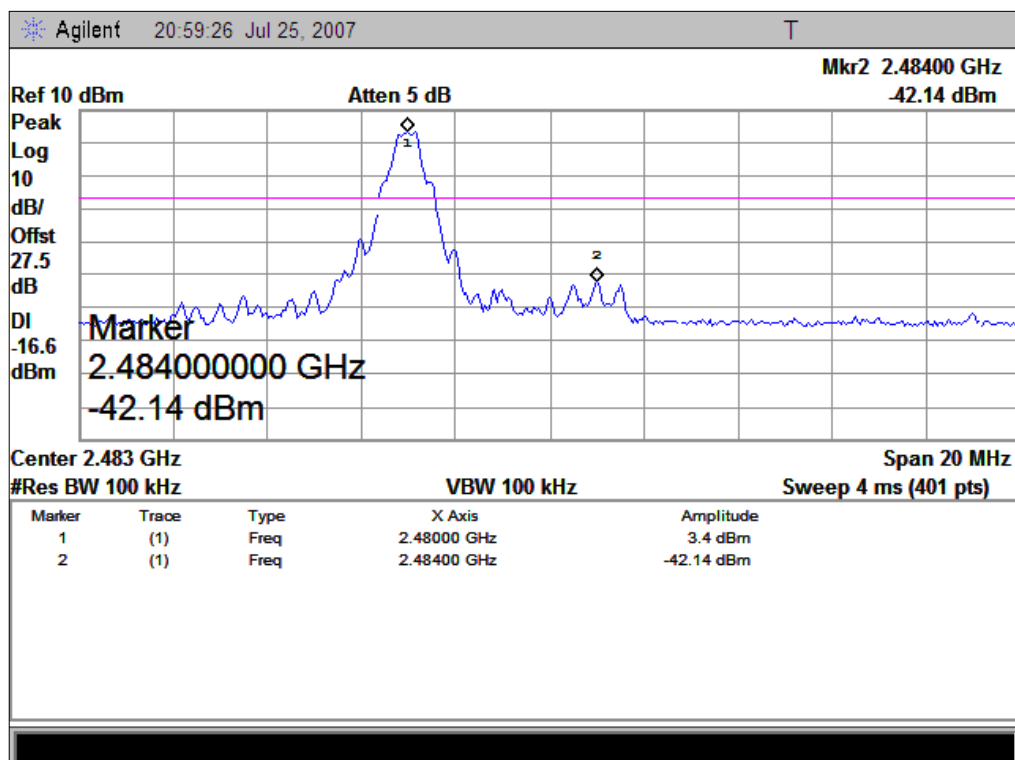
(Plot B: Channel = 78)
