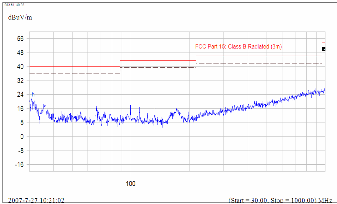
(Plot C.2: Antenna Horizontal, 30MHz to 1GHz)
