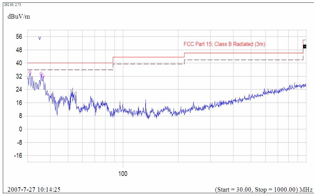
(Plot A.6: Antenna Vertical, 30MHz to 1GHz)
