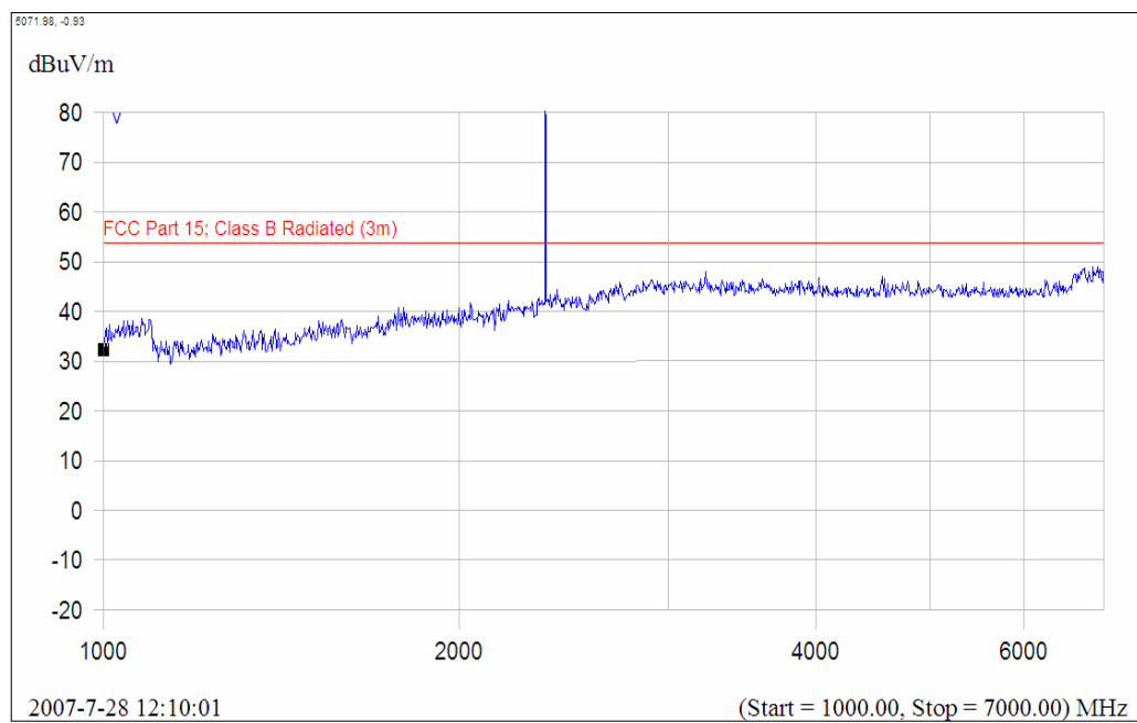
(Plot A.7: Antenna Vertical, 1GHz to 7GHz)
