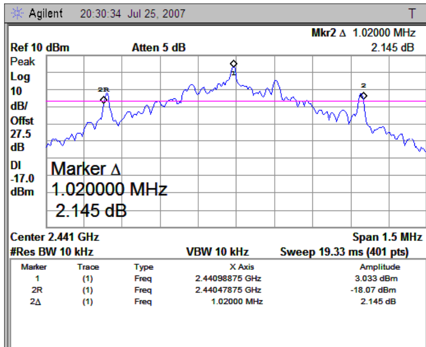
(Plot B: Channel = 2441)
