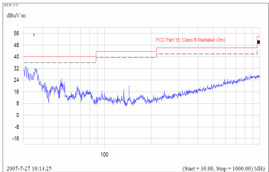
(Plot B.6: Antenna Vertical, 30MHz to 1GHz)
