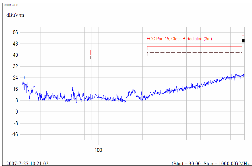
(Plot B.2: Antenna Horizontal, 30MHz to 1GHz)
